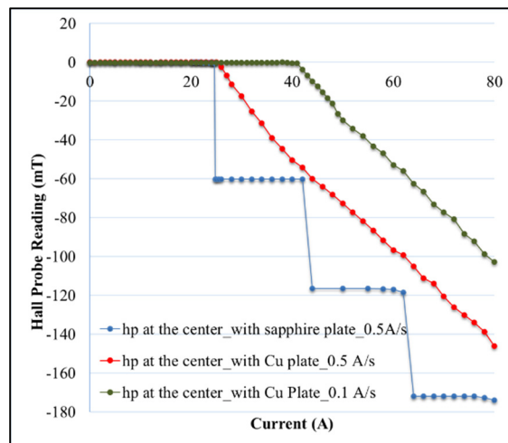
Figure 8: The centre Hall probe responses against forward current observed for \text{Nb}_3\text{Sn} thin film fabricated on sapphire substrate having 1.5\text{ }\mu\text{m} thickness.
