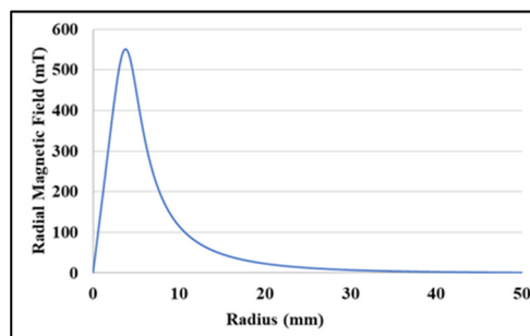
Figure 5: The radial magnetic field generated from magnet on the sample surface with the magnet current 100 A and the corrected separation between the magnet and the sample 1.465 mm.
