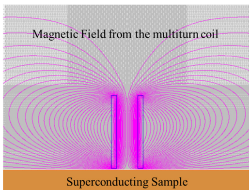
Figure 2: Magnetic field lines from the multiturn coil placed on the superconducting sample in Meissner state.
