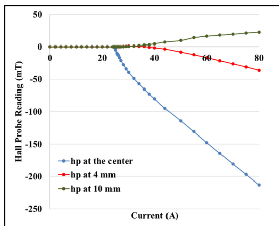
Figure 6: Magnetic field penetration measurements on bulk Nb with thickness 88.9\text{ }\mu\text{m} at 4.35\text{ K} .
