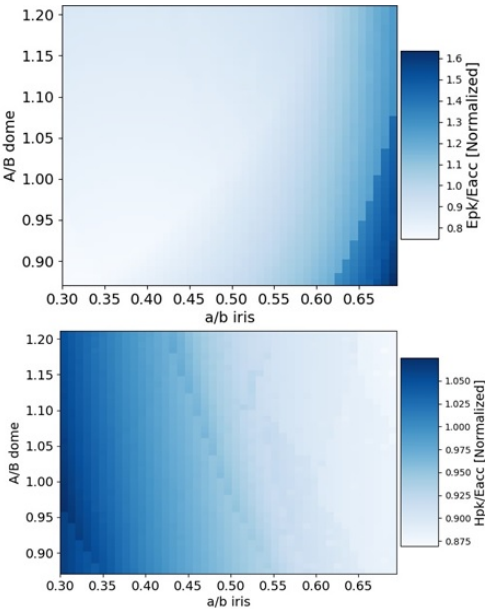
Figure 4: The surface plot by changing the iris and the dome ratio to select the parameters to minimize the E_{pk}/E_{acc} (top) and H_{pk}/E_{acc} (bottom).
