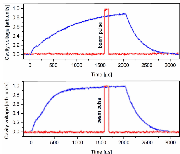
Figure 2: Shape of the cavity voltage before (top) and after (bottom) optimisation.
