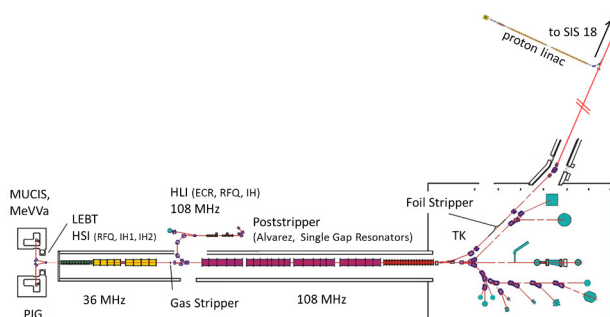
Figure 1: Schematic overview of the GSI UNILAC and FAIR proton linac.
