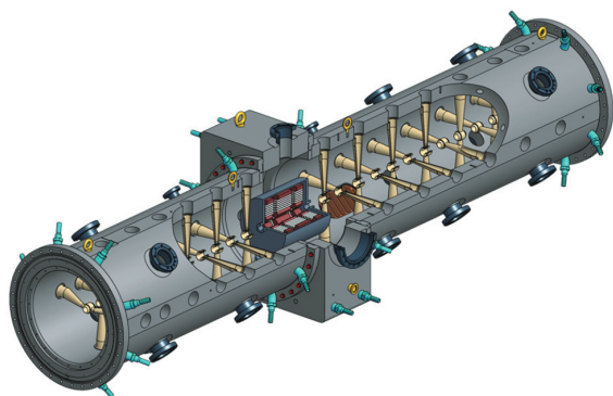
Figure 9: 3D-view (CAD) of the second coupled CH-cavity (section I) [3].
