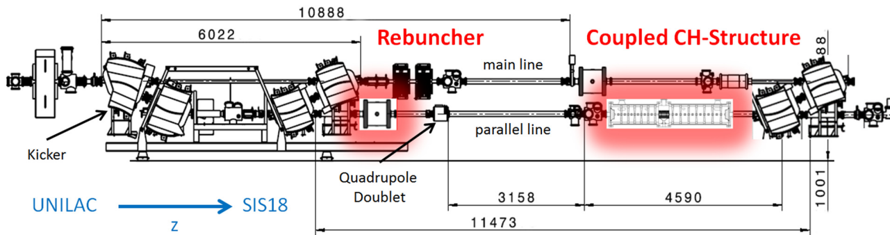
Figure 7: Proposal for first beam tests of high current proton beam operation with coupled CH-cavity in the transfer line.
