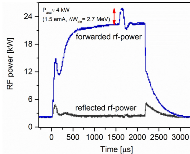
Figure 3: Forwarded and reflected RF power by the influence of the beam on the control system.
