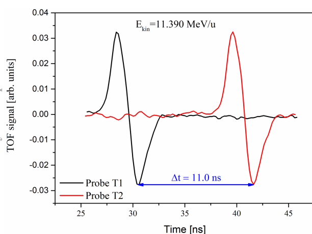
Figure 4: UNILAC proton beam energy measured with the Time of Flight method (phase probe, l=518.5 mm, 11 ns).
