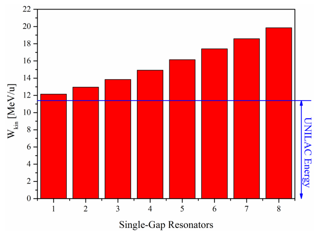
Figure 5: Proton beam energy of 20 MeV using eight single gap resonators.
