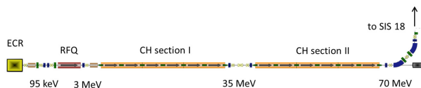
Figure 8: Schematic layout of the FAIR proton linac [3].
