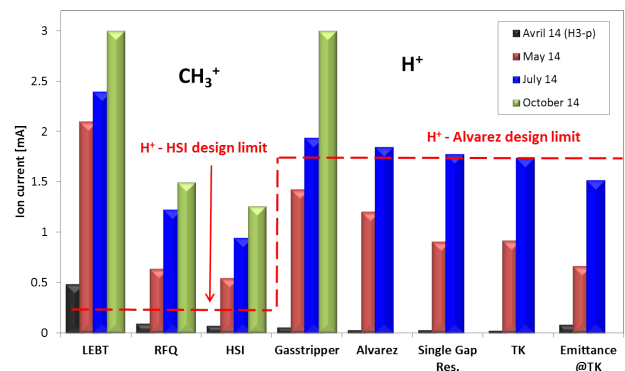
Figure 6: Beam current measurements at UNILAC and transfer line section; after stripping the proton beam operation is above the design limit.
