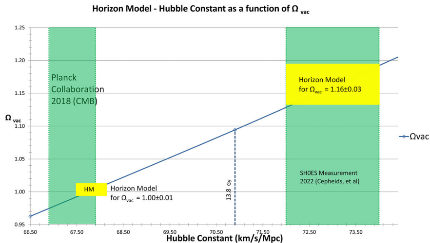
Fig. 1 Horizon Model (HM) values of the Hubble Constant as a function of \Omega_{vac} . With \Omega_{vac} = \Omega = 1.00 \pm 0.01 , the HM value for H ( 67.87 \pm 0.38 ) is within 0.8\sigma of the Planck collaboration measurement. The HM values for H are in perfect agreement with the SH0ES team measurement ( 73 \pm 1 ) if \Omega_{vac} = 1.16 \pm 0.03 . For a Hubble time of 13.8 Gyr, \Omega_{vac} = 1.094
