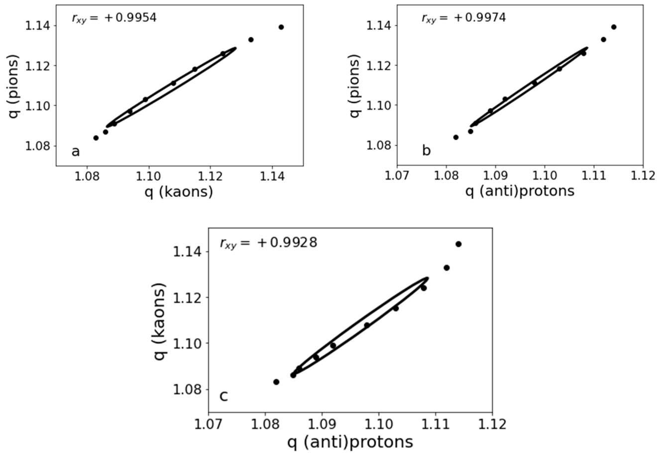
Figure 6. The q(\text{pions}) versus q(\text{kaons}) (a), q(\text{pions}) versus q((\text{anti})\text{protons}) (b), and q(\text{kaons}) versus q((\text{anti})\text{protons}) (c) dependencies, obtained using Equation (5) and presented in Table 2. The corresponding 1-sigma confidence ellipses and Pearson correlation coefficients are also shown in the figures.
