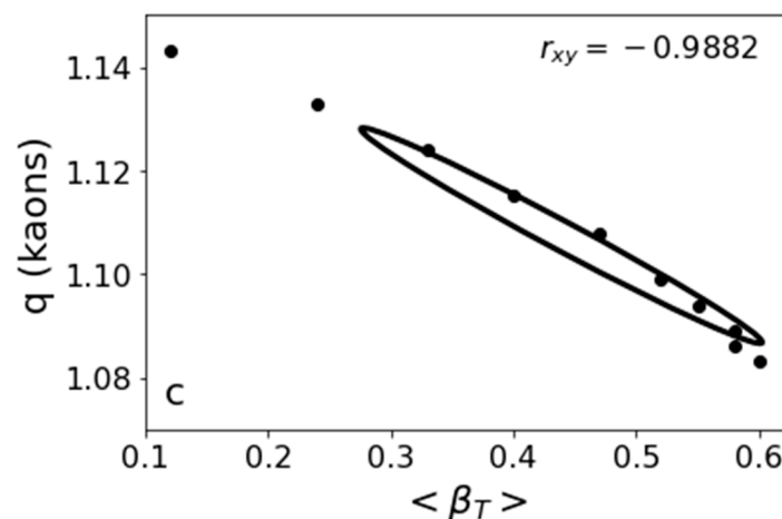
Figure 7. The q(\text{pions}) versus \langle \beta_T \rangle (a), q(\text{(anti)protons}) versus \langle \beta_T \rangle (b), and q(\text{kaons}) versus \langle \beta_T \rangle (c) dependencies, obtained using Equation (5) and presented in Table 2. The corresponding 1-sigma confidence ellipses and Pearson correlation coefficients are also shown in the figures.
