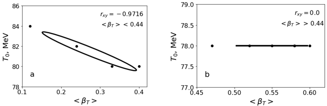
Figure 5. (a)—Dependence (•) of T_0 versus \langle\beta_T\rangle parameters, extracted using Equation (5) and presented in Table 2, in region \langle\beta_T\rangle < 0.44 . (b)—Dependence (•) of T_0 versus \langle\beta_T\rangle parameters, extracted using Equation (5) and presented in Table 2, in region \langle\beta_T\rangle > 0.44 . The corresponding 1-sigma confidence ellipses and Pearson correlation coefficients are also shown in the figures.
