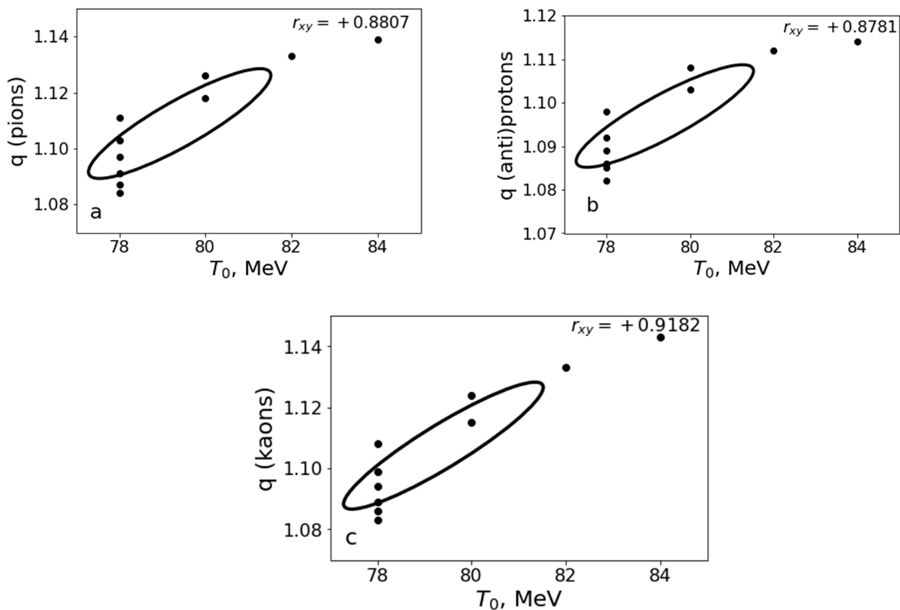
Figure 8. The q(\text{pions}) versus T_0 (a), q(\text{(anti)protons}) versus T_0 (b), and q(\text{kaons}) versus T_0 (c) dependencies, obtained using Equation (5) and presented in Table 2. The corresponding 1-sigma confidence ellipses and Pearson correlation coefficients are also shown in the figures.
