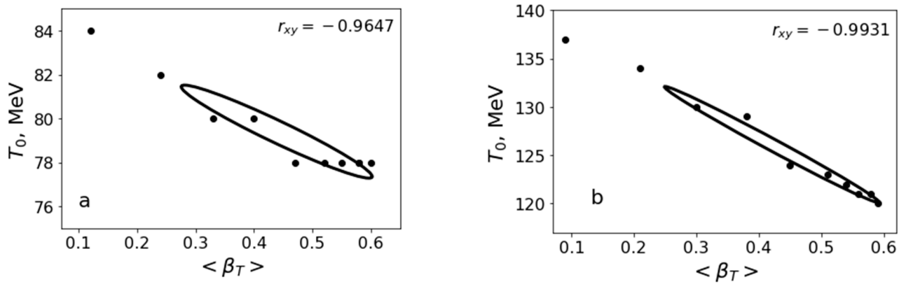
Figure 4. (a)—Dependence (•) of T_0 versus \langle\beta_T\rangle parameters extracted using Equation (5) and presented in Table 2. (b)—Dependence (•) of T_0 versus \langle\beta_T\rangle parameters extracted using Equation (4) and presented in Table 3. The 1-sigma confidence ellipse (which corresponds to a 68% confidence interval) of the covariance of parameters T_0 and \langle\beta_T\rangle and the calculated Pearson correlation coefficient, r_{xy} , between T_0 and \langle\beta_T\rangle are also given in the figures.
