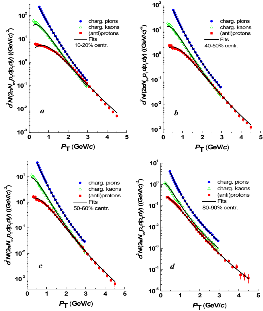
Figure 2. The resulting fit curves by non-consistent Tsallis function with included transverse flow (Equation (4)) of the experimental midrapidity transverse momentum spectra of the charged pions (●), kaons (△), and protons and antiprotons (■) in Pb + Pb collisions at \sqrt{s_{nn}} = 2.76 TeV at various centralities: 10–20% (a), 40–50% (b), 50–60% (c), and 80–90% (d).
