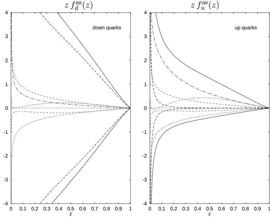
Fig. 4. Asymptotic electron structure function. The positively valued curves show the quark content of unpolarized electron, (e_R^- + e_L^-)/2 . The negative ones — the left-right asymmetry, (e_R^- - e_L^-)/2 . Full lines give the asymptotic result with all \gamma , Z and W included. The other curves give the contributions from: \gamma\gamma — dashed-dotted; \gamma Z — dotted; ZZ — short dashed; WW — long dashed.
