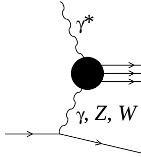
Fig. 2. \gamma, Z, W contributions to the \gamma^* e^- scattering
