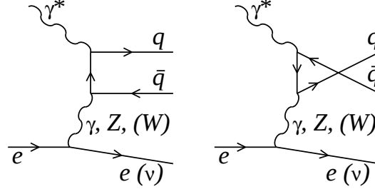
Fig. 3. Feynman diagrams contributing to the electron \rightarrow quark/anti-quark splitting functions
