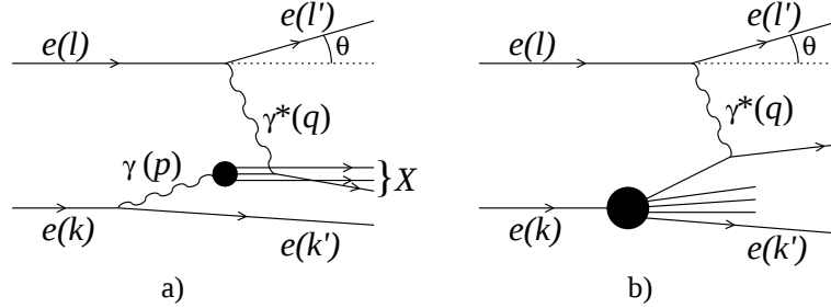
Fig. 1. Deep inelastic scattering on a photon (a) and electron (b) target
