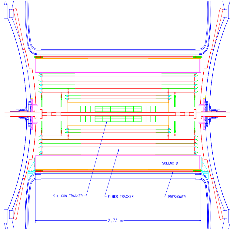
Figure 3.4: The DØ central tracking system.
