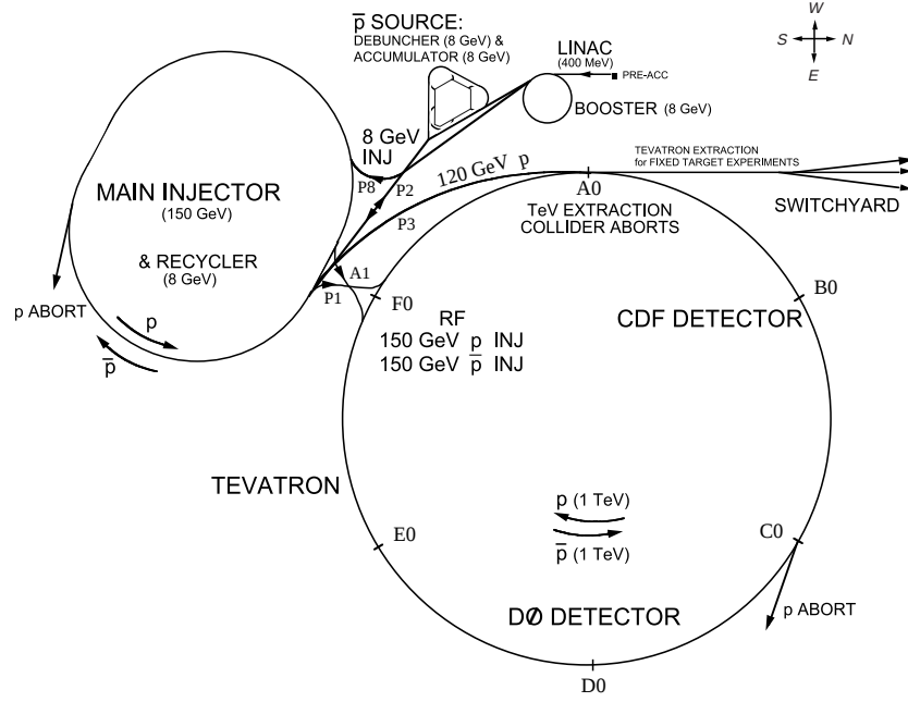
Figure 3.1: The Fermilab accelerator complex.
