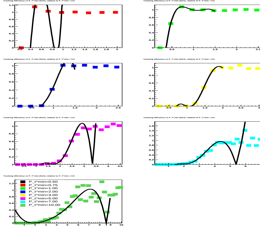
Figure A.14: Estimated tracking efficiency as a function of track P_T .
