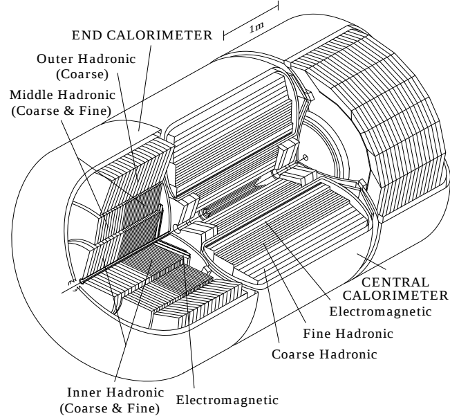
Figure 3.7: Cut-away view of the calorimeter, showing the division into electromagnetic and hadronic sections as well as central and forward regions.
