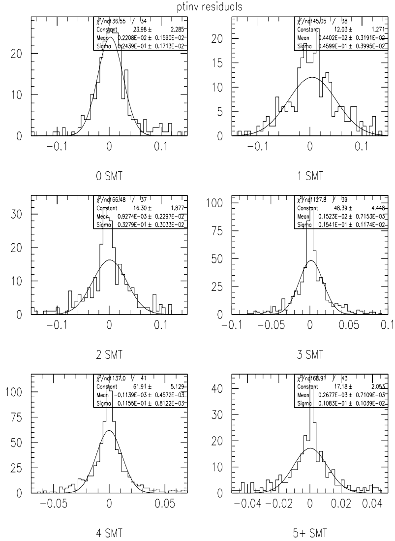
Figure A.20: Residual in the track parameter \frac{q}{P_T} , for reconstructed and simulated tracks in 100 t\bar{t} \rightarrow \ell j j events, for varying number of SMT clusters on the track.
