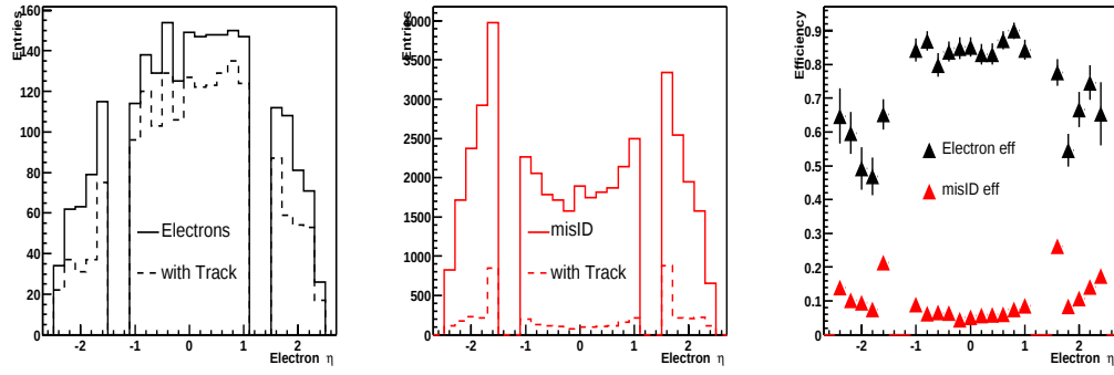
Figure B.5: Efficiencies to have a track candidate for calorimeter EM objects in the signal and background samples.
