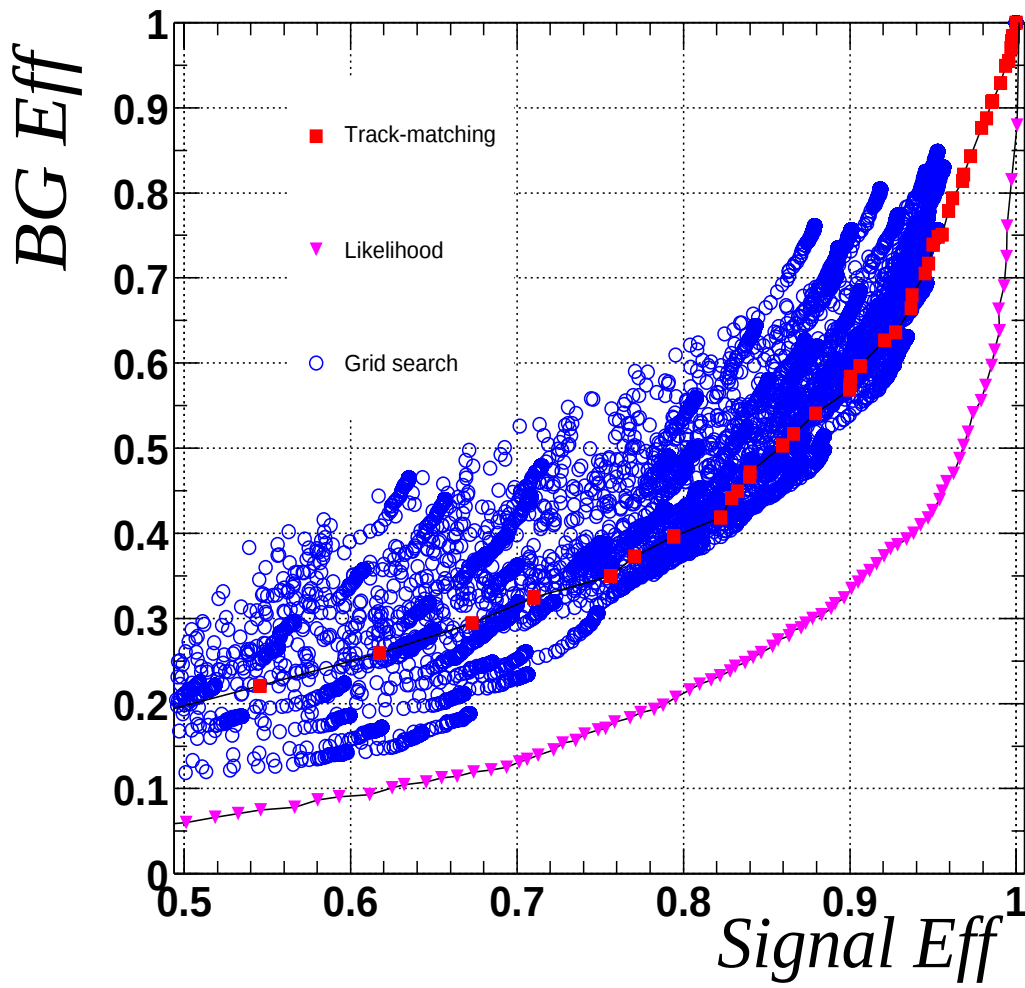
Figure B.8: A comparison of the performance of the track matching, the likelihood and a grid-search in the central calorimeter over the six likelihood variables.
