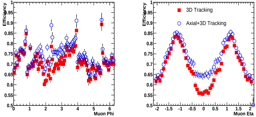
Figure 5.7: Muon tracking and matching efficiencies as a function of \phi and \eta of the muon, in data.
