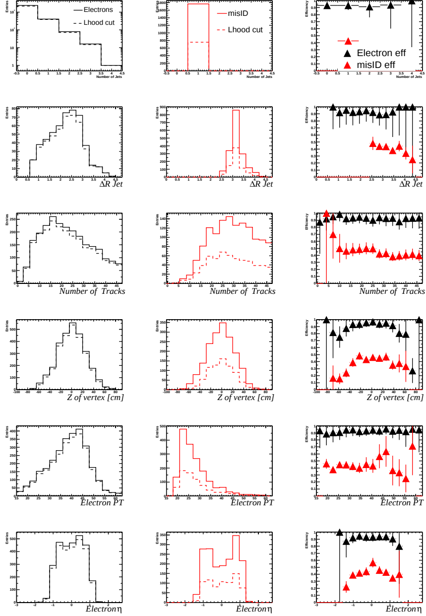
Figure B.9: The topological dependence of the signal and background efficiencies in the central calorimeter given a fixed cut on the discriminant. The distributions in the signal and background samples are the two left columns, respectively. The efficiencies are shown in the rightmost column.
