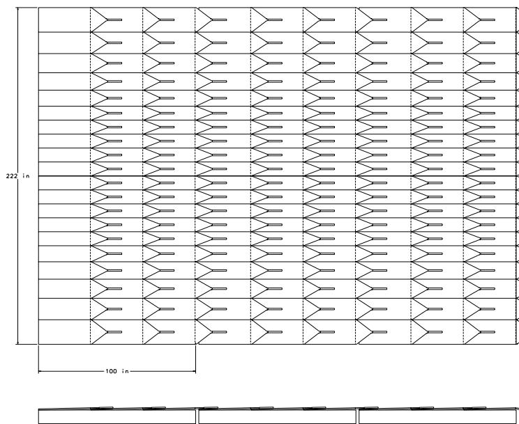
Figure 3.12: Arrangement of scintillator pixels in the central muon system.
