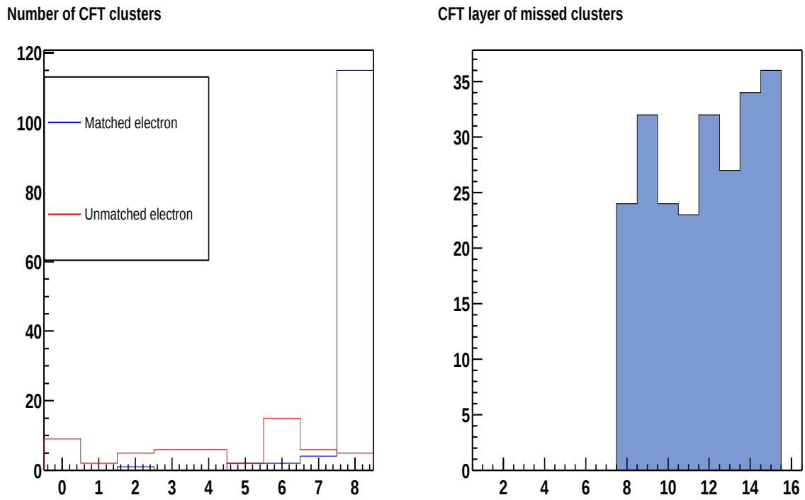
Figure A.10: Left, the number of layers with a CFT cluster within 0.025 radians of the propagated electron position for matched and unmatched electrons. Right, the layers on which clusters were not found.
