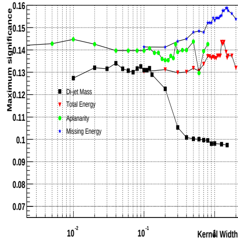
Figure D.4: Variation of support vector regression performance (measured by maximum significance s , defined in the text), as a function of the width of the Gaussian kernel for each physics parameter.
