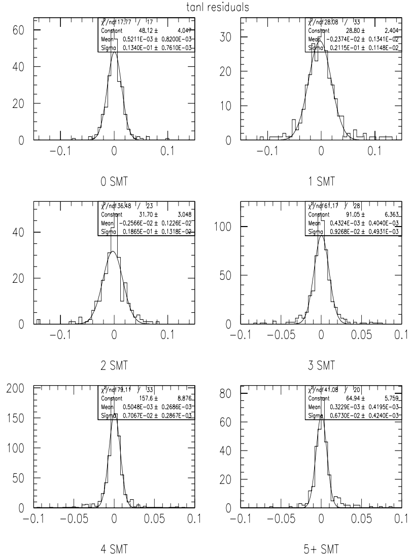
Figure A.19: Residual in the track parameter \tan \lambda , for reconstructed and simulated tracks in 100 t\bar{t} \rightarrow llj\bar{j} events, for varying number of SMT clusters on the track.
