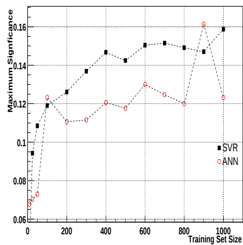
Figure D.5: Variation of support vector regression and artificial neural network performance (measured by maximum significance s , defined in the text), as a function of the size of the training sample.
