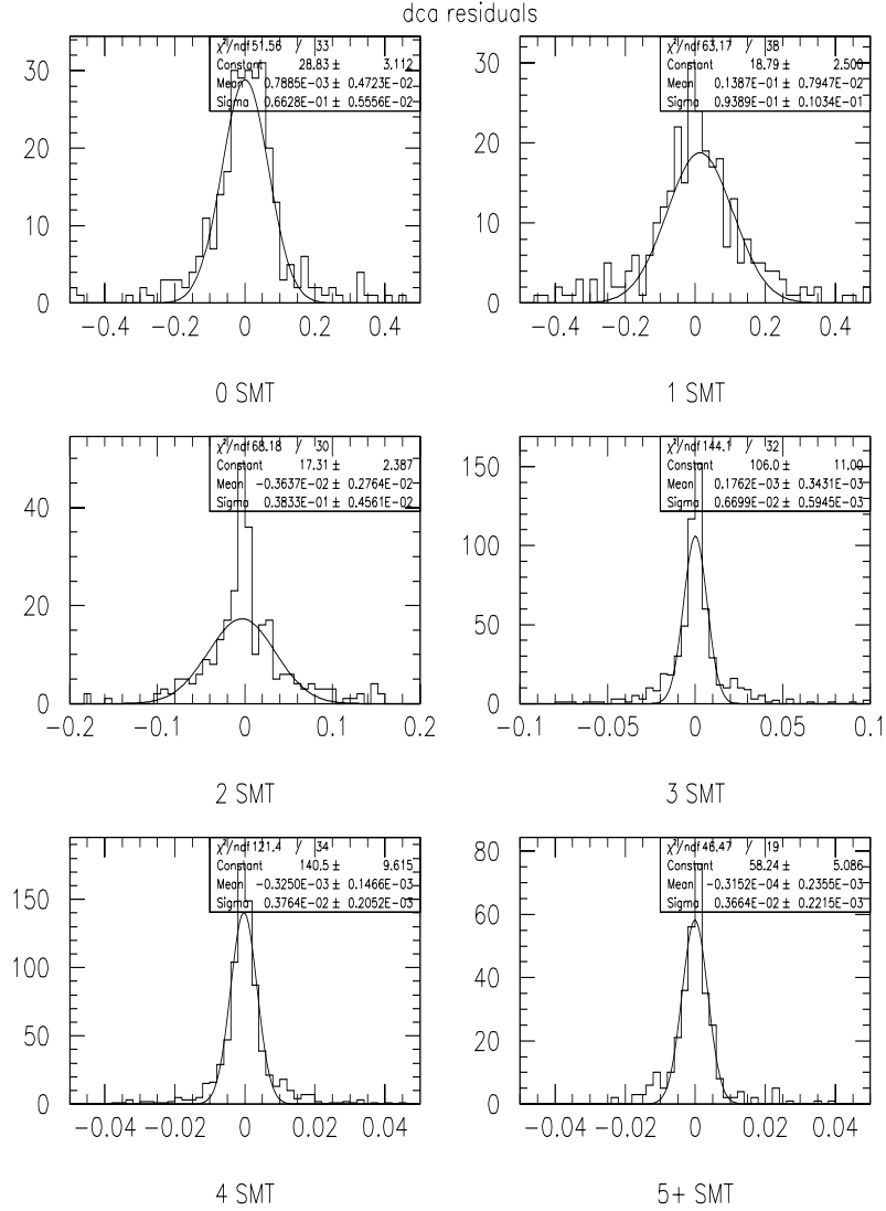
Figure A.16: Residual in the track parameter DCA , for reconstructed and simulated tracks in 100\ t\bar{t} \rightarrow llj\bar{j} events, for varying number of SMT clusters on the track.
