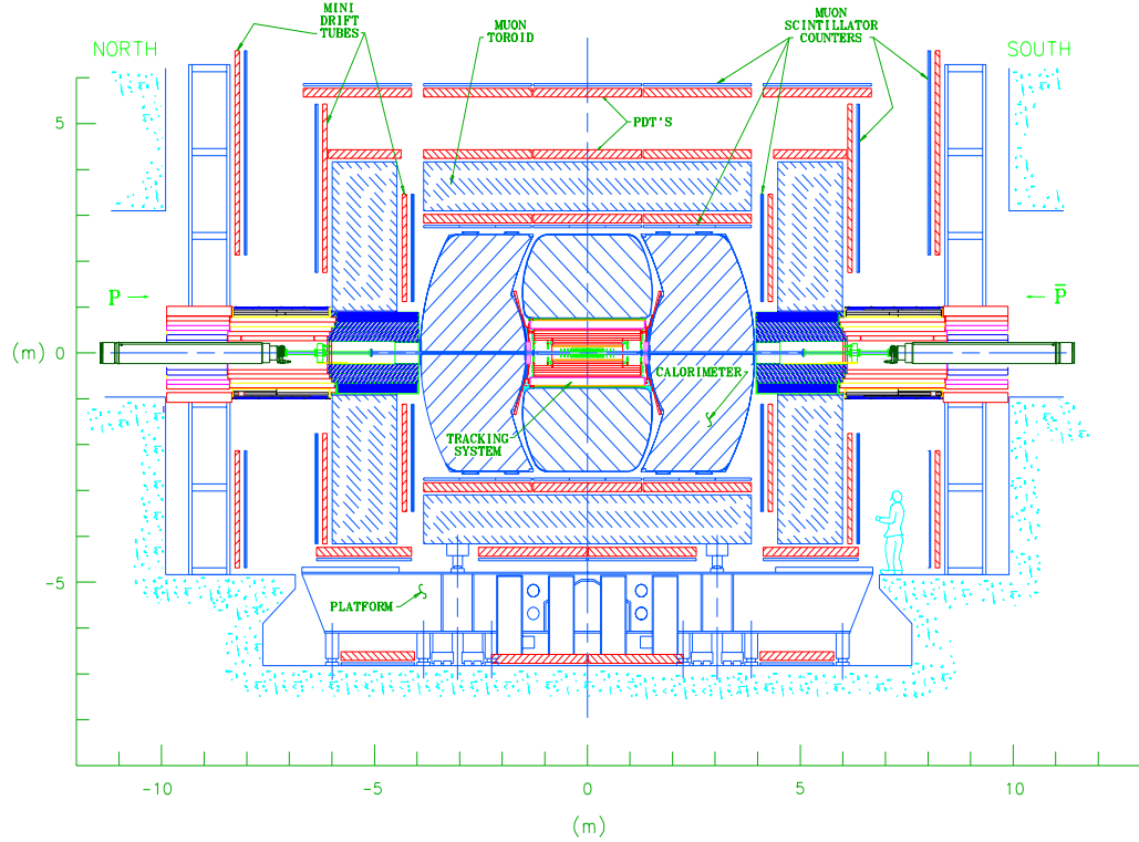
Figure 3.3: Side view of the DØ detector.
