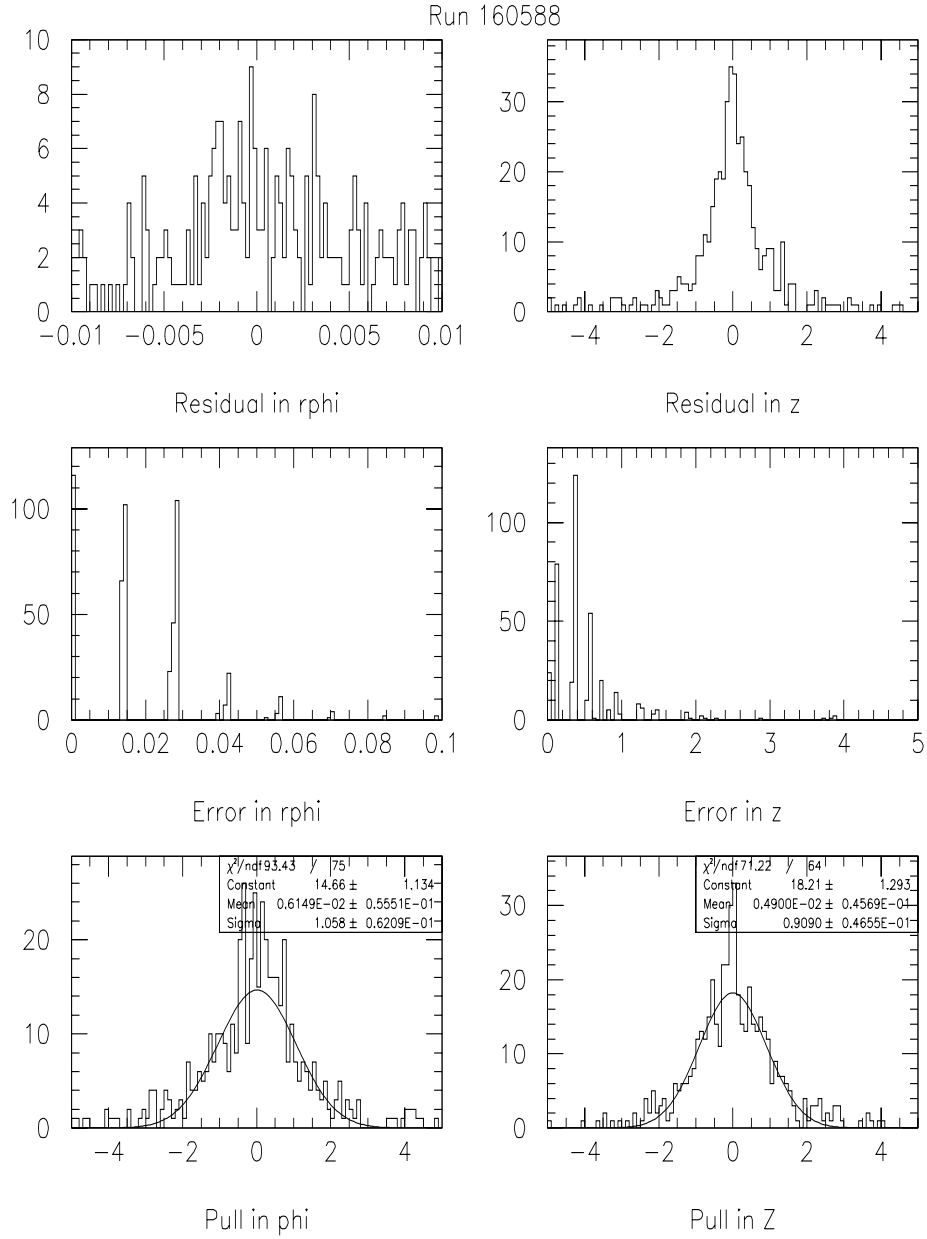
Figure A.23: Top shows hit to track residuals; middle shows cluster errors; bottom shows hit to track pulls. Left column shows quantities in r\phi ; right column shows quantities in z . From run 160588.
