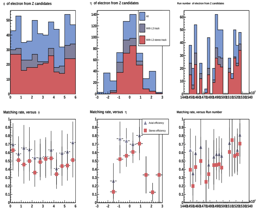
Figure A.7: Efficiency for matching electrons to tracks in Z \rightarrow e^+e^- data. Top row shows the absolute numbers of EM objects, axial matched EM's and stereo matched EM's as a function of \phi (left), \eta (middle) and run number (right). Bottom shows the axial and stereo efficiency.
