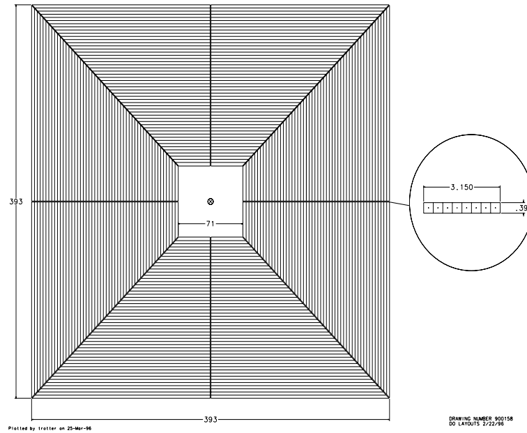
Figure 3.11: Arrangement of drift tubes in the forward muon system.
