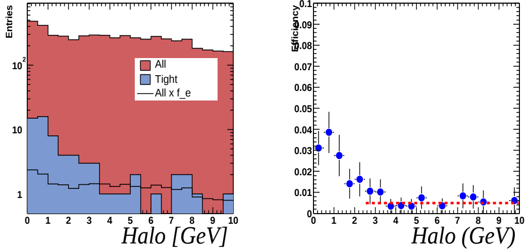
Figure 6.1: Preselected events which contain a loose electron, and the subset of those events which contain a tight electron, ( left ). The rate at which loose electrons pass the tight cuts, as a function of the muon halo energy ( right ). Shown for the central calorimeter.
