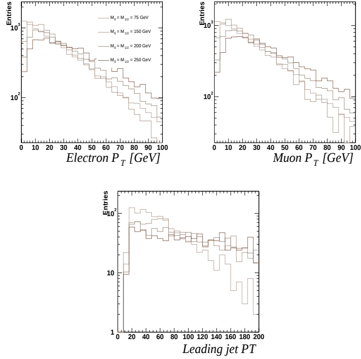
Figure 9.7: Electron, muon and jet energies for \tilde{t}_1^+ \tilde{t}_1^- \rightarrow b l \nu \chi_1^0 b l \nu \chi_1^0 production at selected mSUGRA model points
