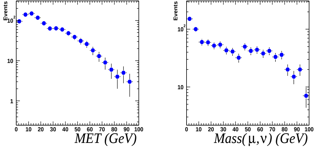
Figure 6.3: Distributions in missing transverse energy and transverse mass of isolated muon events.
