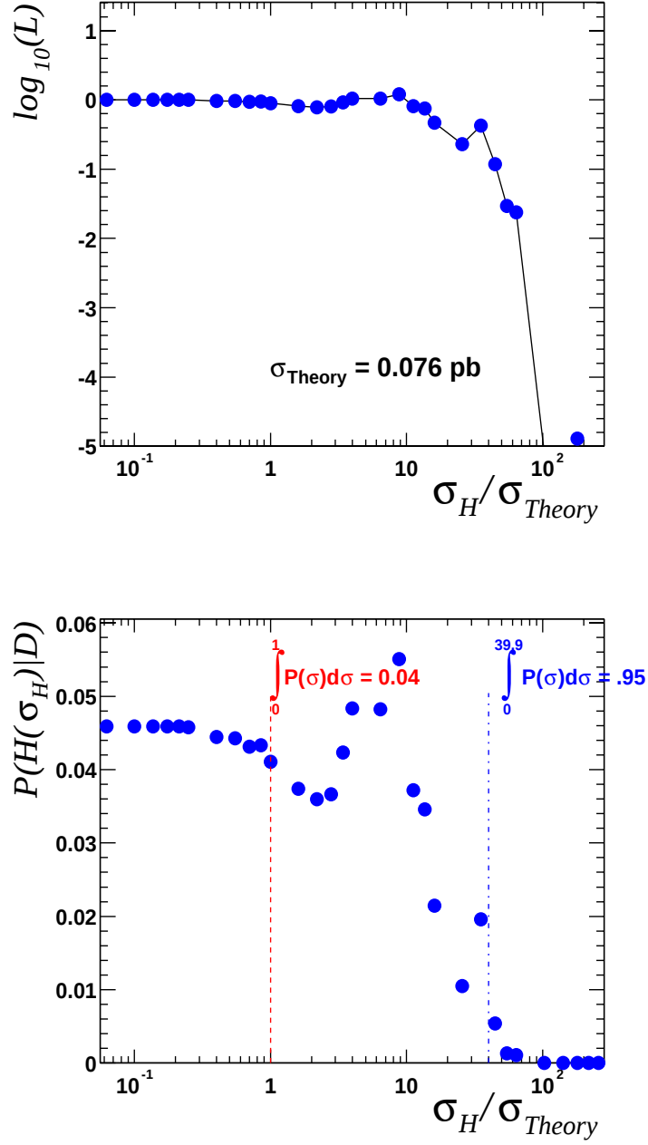
Figure 9.19: Tests of the hypothesis H_{\chi_1^\pm \chi_2^0} with m_0, m_{1/2} = 150 \text{ GeV} , at varying cross-sections, relative to the theoretical prediction.
