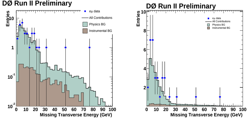
Figure 9.34: Missing transverse energy in e\mu events with no jets, for data and backgrounds in both log and linear scales.
