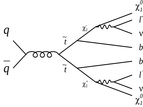
Figure 9.6: Feynman diagram for the leading contribution to the process p\bar{p} \rightarrow \tilde{t}_1^+ \tilde{t}_1^- \rightarrow b\bar{b} l \nu \chi_1^0 l \nu \chi_1^0 .
