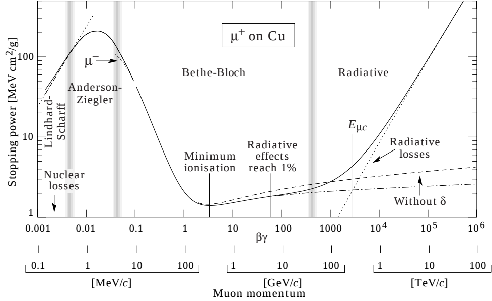
Figure 3.2: Energy loss through ionization of muons in various energy regimes. From [62].
