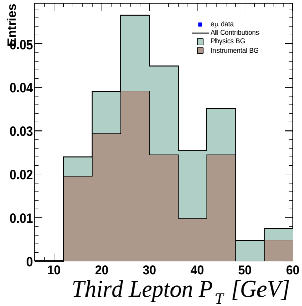
Figure 9.16: Estimation of contributions to trilepton final state. No events are seen in the data
