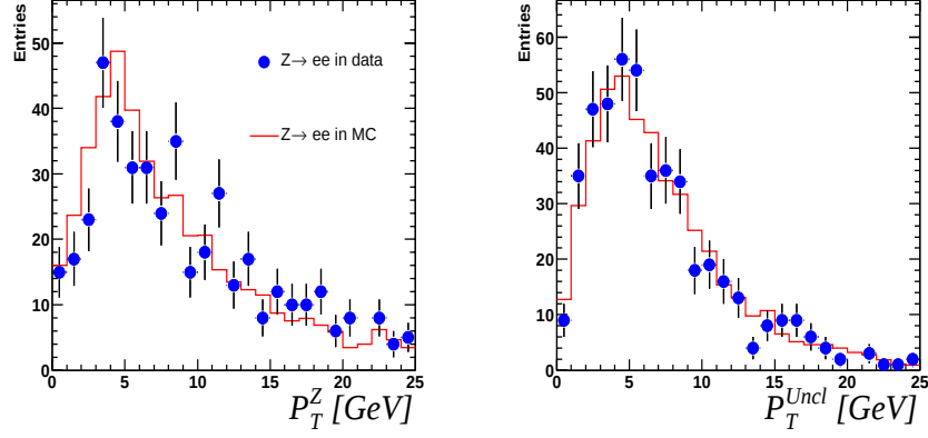
Figure 5.17: Transverse momentum of the Z boson, and the unclustered energy in data and simulation
