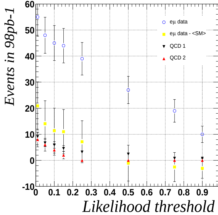
Figure 6.5: Variation in estimated sizes of real and misidentified contributions to e\mu dataset with likelihood threshold.
