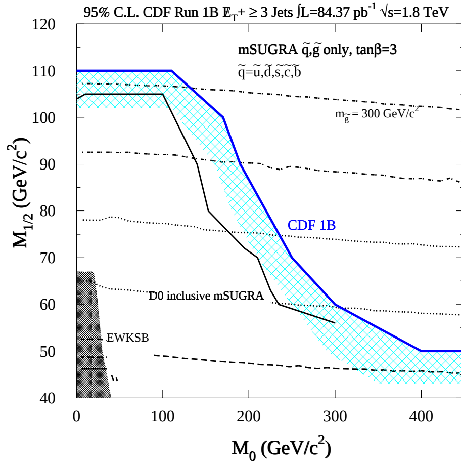
Figure 9.31: Exclusions in the m_0, m_{\frac{1}{2}} plane using jets and \cancel{E}_T signatures in Run1, from [74].
