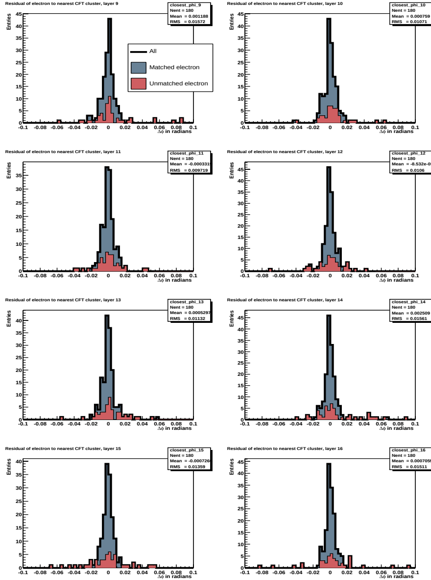
Figure A.9: Residual between electron and the nearest CFT cluster at each of eight axial CFT layers. The solid line shows all the clusters, the blue region shows track matched electrons and the red region shows unmatched electrons.
