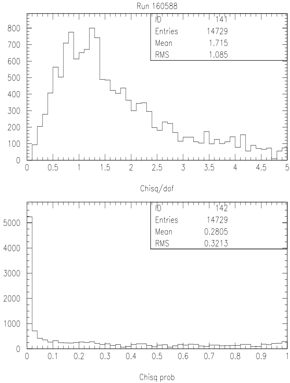
Figure A.24: Top, \chi^2/N_{dof} for tracks from run 160588. Bottom, the \chi^2 probability for each track.
