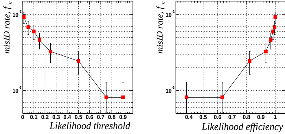
Figure 6.4: Variation in electron misidentification rate and efficiency with varying likelihood thresholds.
