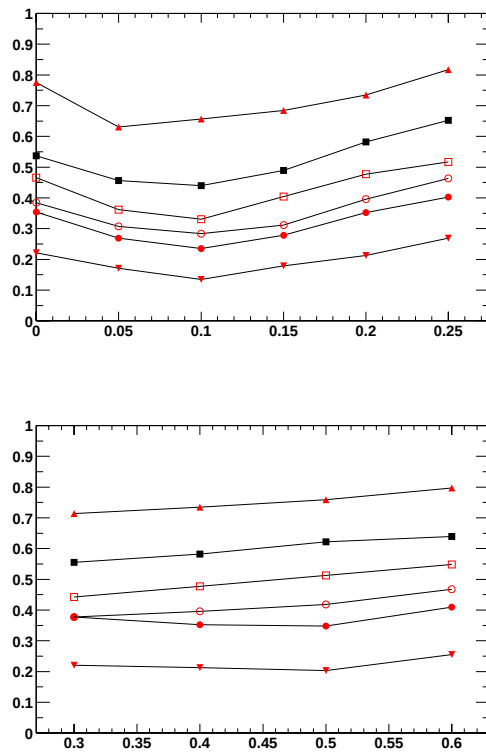
Figure C.8: QCD efficiency for different inner cone sizes, at given signal ( Z ) efficiencies.
