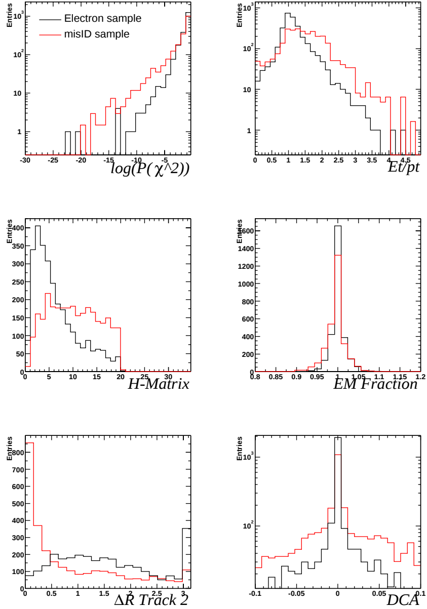
Figure B.1: Distributions of variables used in the likelihood for central calorimeter signal and backgrounds samples, as defined in the text. Distributions are shown only for EM objects which have a track candidate.
