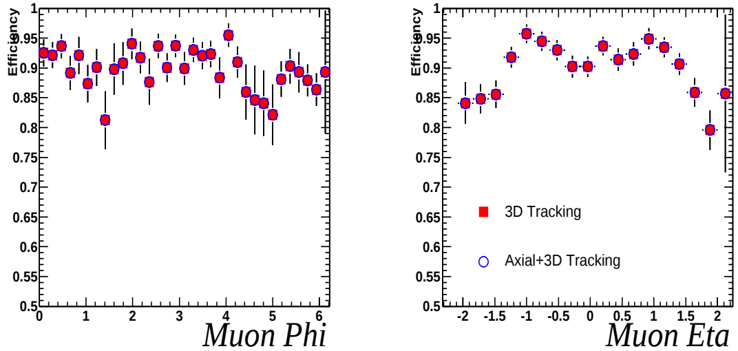
Figure 5.6: Muon tracking and matching efficiencies as a function of \phi and \eta of the muon, in simulated events.
