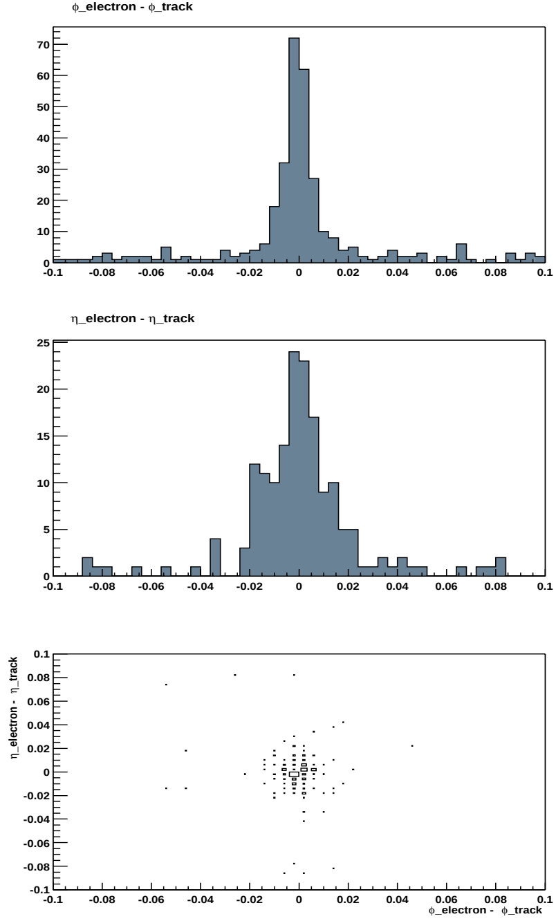
Figure A.6: Residuals between EM object and nearest track in Z \rightarrow e^+e^- data. Top is \Delta\phi ; middle is \Delta\eta ; bottom shows the correlation.
