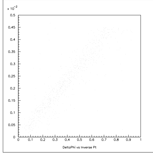
Figure A.1: Distance in \phi between the outer two axial CFT hits versus inverse P_T for tracks from Z \rightarrow b\bar{b} events. Units of \Delta\phi are radians and of P_T^{-1} are \text{GeV}^{-1} .
