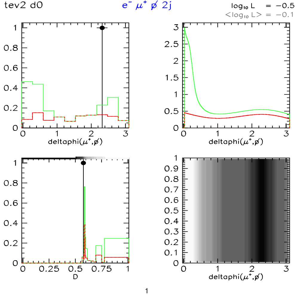
Figure 9.23: Test of the hypothesis H_{\tilde{t}\tilde{t}} with m_0, m_{\frac{1}{2}} = 150 GeV in the e^- \mu^+ \cancel{p} 2j final state. Clockwise from top left: histogrammed events in the selected variable for the Standard Model ( red ) and the new physics hypothesis ( green ); probability densities for each hypothesis; subregions of the variable determined by placing cuts on the discriminant; and binned values of the discriminant for SM and new physics.
