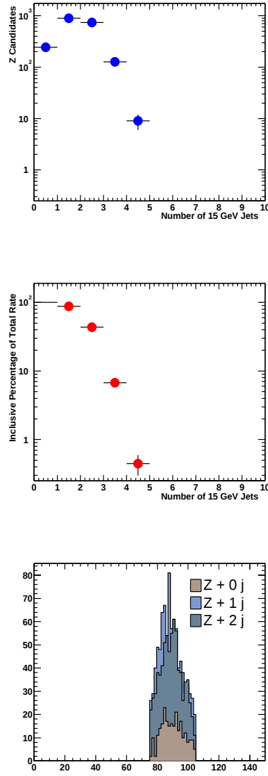
Figure 6.9: Jet multiplicity in ALPGEN simulated Z \rightarrow \mu\mu events ( top ), inclusive percentage of total rate ( middle ) and invariant mass distributions for leading portions ( bottom ).
