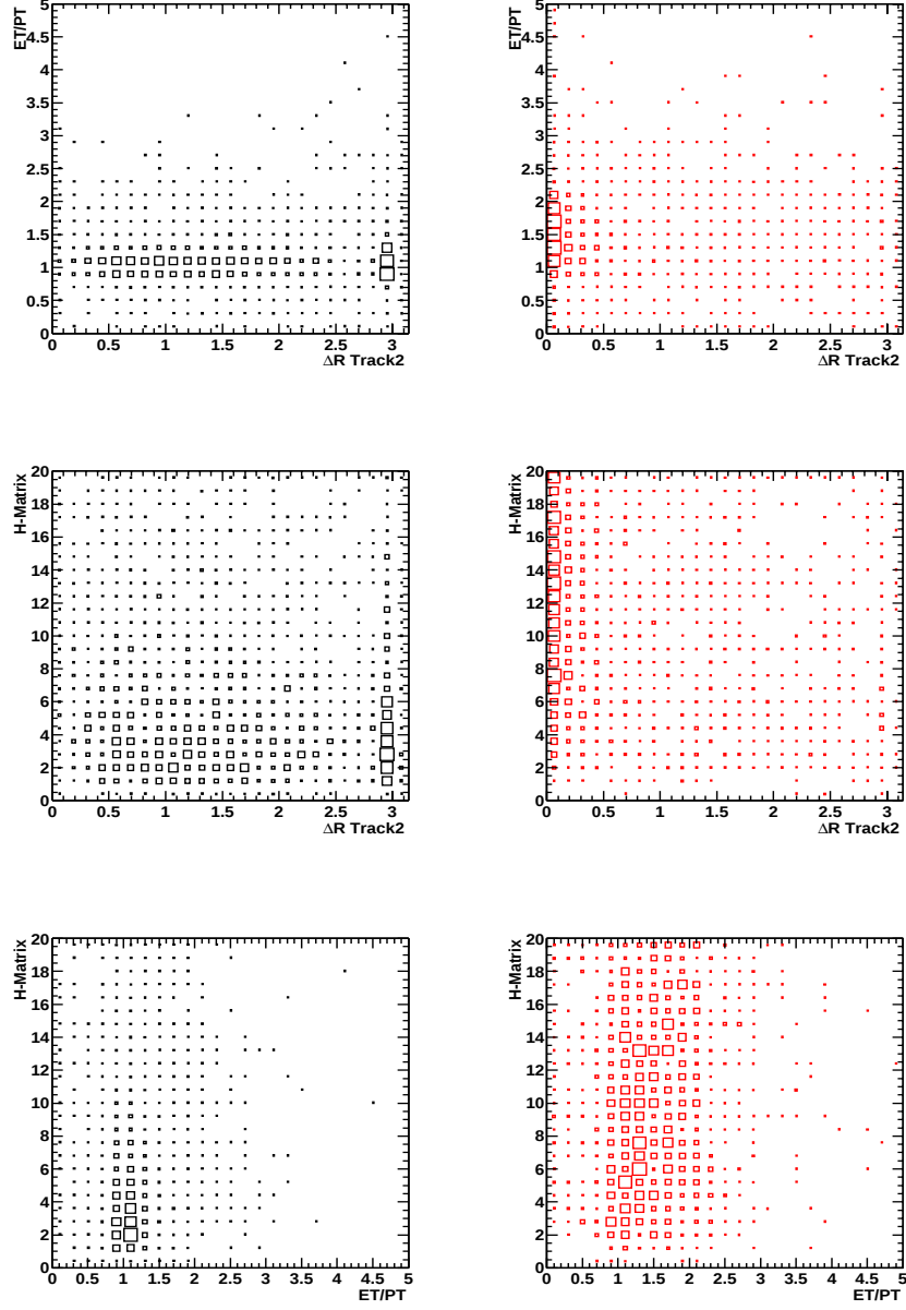
Figure B.2: Correlations between selected variables use in the construction of the likelihood, for the central calorimeter signal sample ( left ) and the background sample ( right ). Distributions are shown only for those electrons which have a track candidate.
