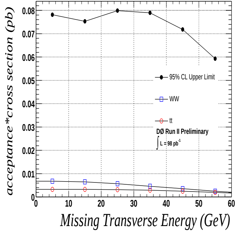
Figure 9.38: Upper limits on the production cross section of new physics in the e\mu j channel, as a function of the lower threshold on missing transverse energy in the event.
