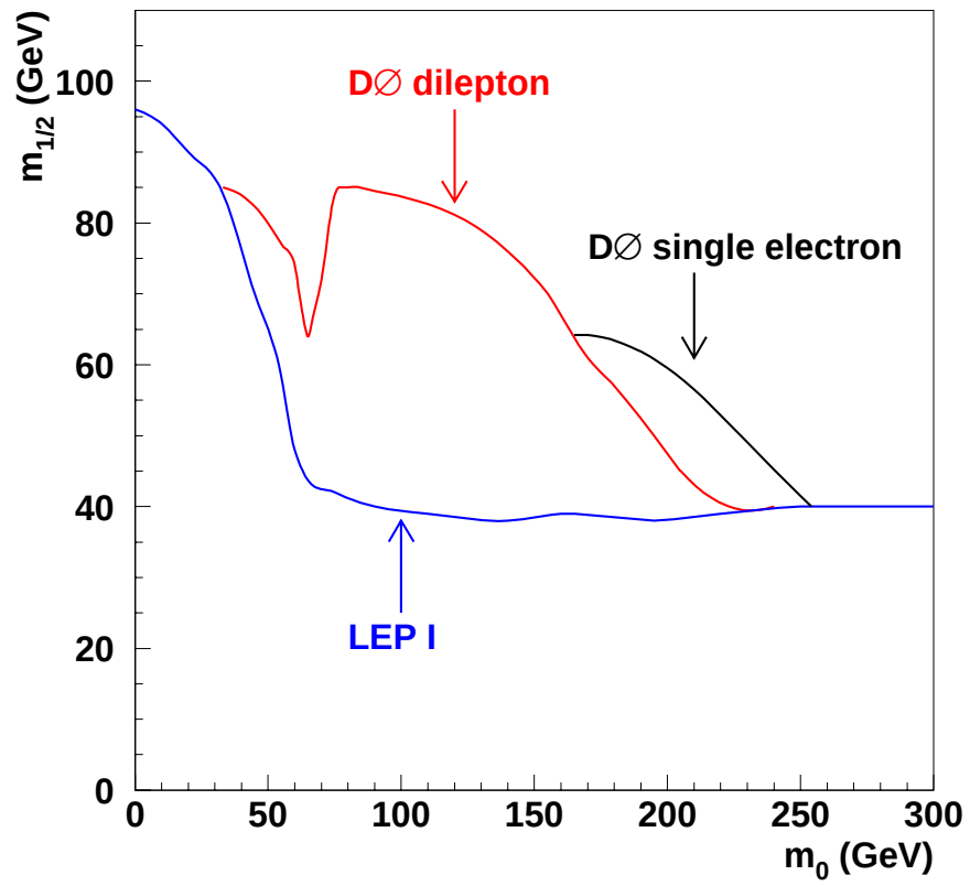
Figure 9.30: Exclusions in the m_0, m_{1/2} using dilepton and electron+jets signatures in Run1, from [75].
