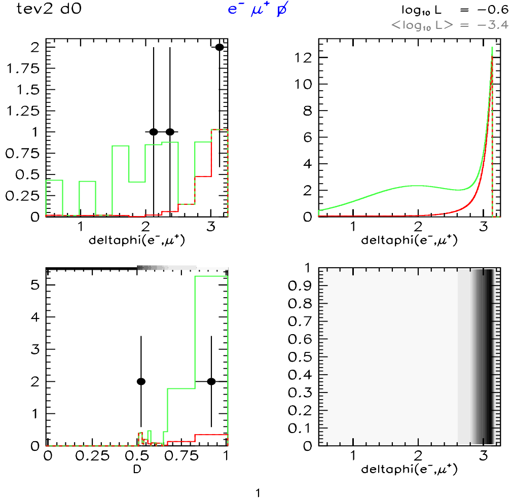
Figure 9.21: Test of the hypothesis H_{\chi_1^+ \chi_1^-} with m_0, m_{1/2} = 150 GeV in the e^- \mu^+ \cancel{p}_T final state. Clockwise from top left: histogrammed events in the selected variable for the Standard Model ( red ) and the new physics hypothesis ( green ); probability densities for each hypothesis; subregions of the variable determined by placing cuts on the discriminant; and binned values of the discriminant for SM and new physics.
