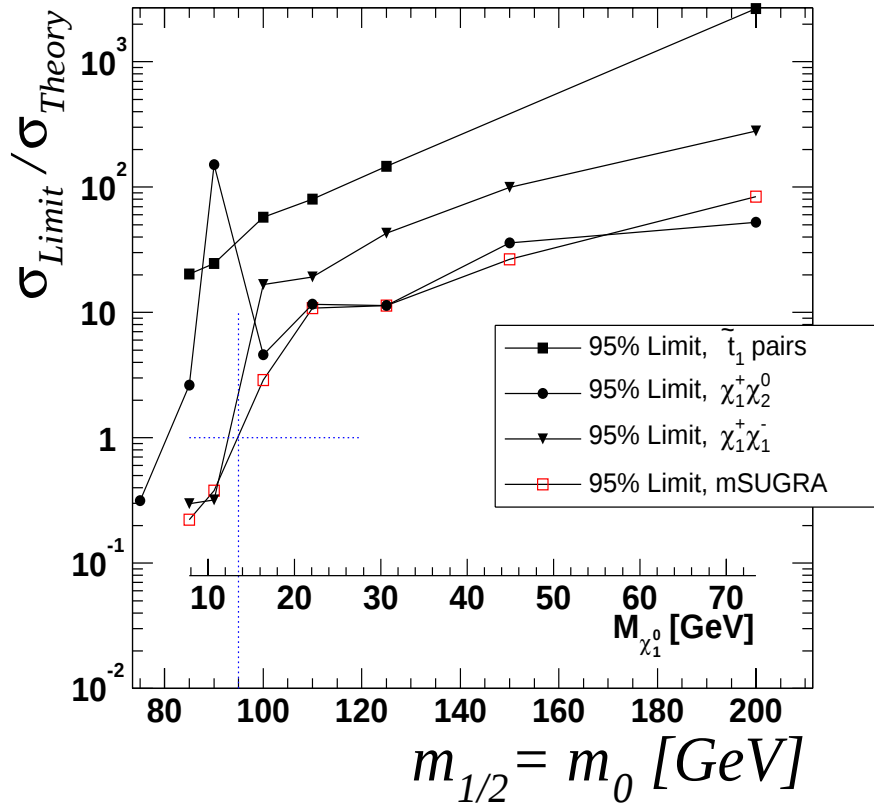
Figure 9.27: Limits on mSUGRA with varying parameters m_0 = m_{\frac{1}{2}} .
