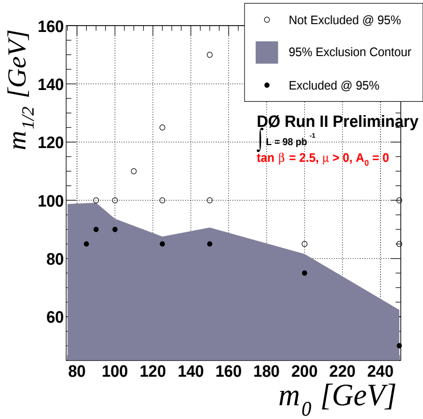
Figure 9.28: Limits on mSUGRA with \mu > 0 in the m_0, m_{\frac{1}{2}} plane.
