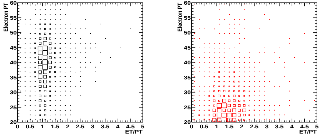
Figure B.3: Correlations between E_T/p_T and electron p_T for the central calorimeter signal sample ( left ) and the background sample ( right ). Distributions are shown only for those electrons which have a track candidate.
