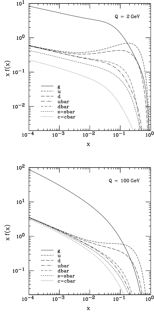
Figure 2.2: Parton distribution functions at varying scales of transverse momentum exchange ( Q^2 )[8].
