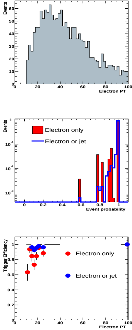
Figure 4.4: Top, distribution of P_T for electrons in t\bar{t} \rightarrow e\mu jj events. Center, per-event probability to pass L1 EM trigger, when only electrons are allowed to fire the trigger, or when either electrons or jets may fire it. Bottom, total L1 EM efficiency as a function of corrected electron P_T .
