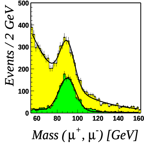
Figure 5.5: Di-muon invariant mass of a local, central-matched muon and a central track. Cases where the second track has a reconstructed muon are also shown.
