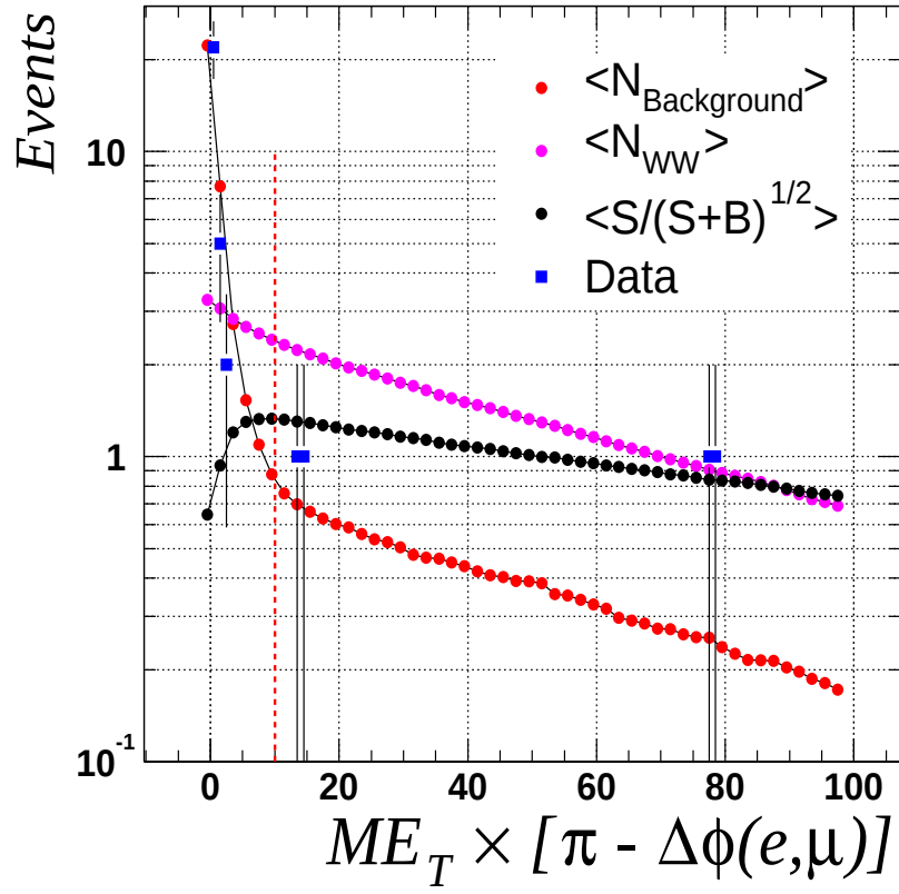
Figure 8.13: Optimization of the point of selection for the quantity E_T \times [\pi - \Delta\phi(e, \mu)] by maximizing \frac{S}{\sqrt{(S+B)}} .
