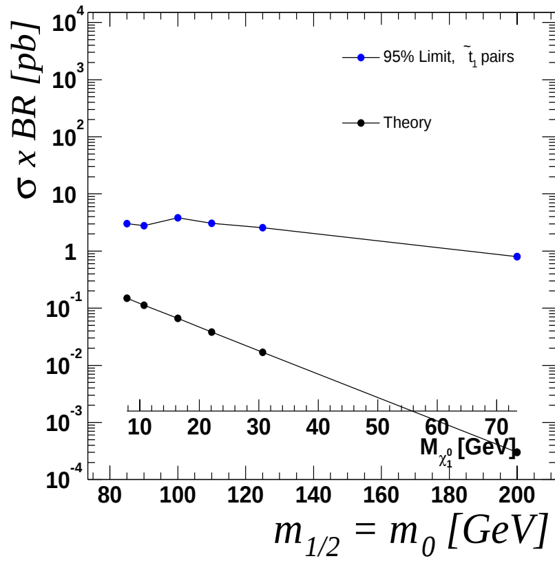
Figure 9.26: Limits on \sigma_{\tilde{t}_1^+ \tilde{t}_1^-} \times BR(e\mu) . m_0 = m_{1/2} .
