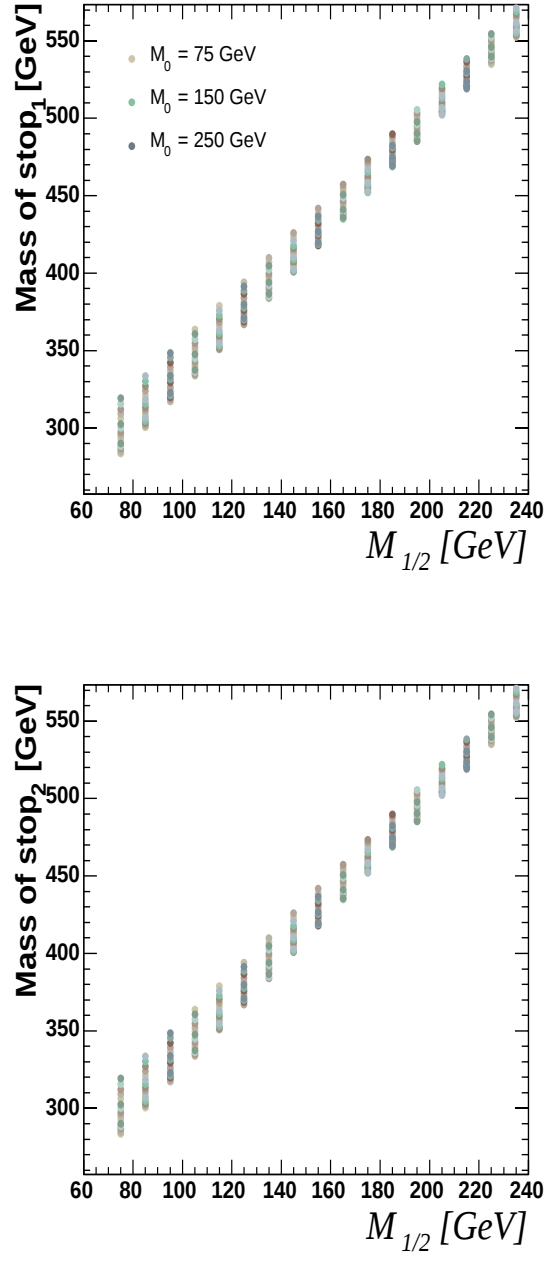
Figure 9.10: Variation in masses of \tilde{t}_{1,2} with mSUGRA parameter m_{\frac{1}{2}} . Various curves demonstrate a scan of m_0 in the region [75, 250] GeV.
