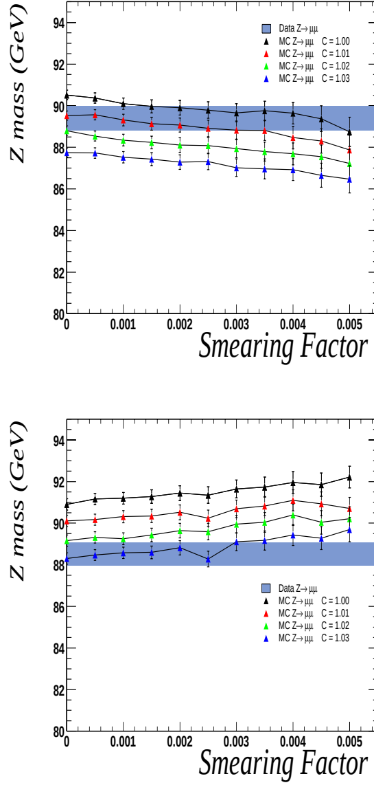
Figure 5.11: Comparison of the fitted mean of the dimuon invariant mass spectrum in real and simulated data, for varying values of the smearing parameters f and C . See text for details.
