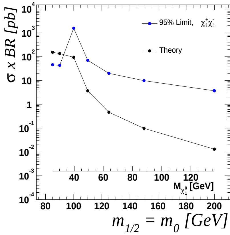
Figure 9.25: Limits on \sigma_{\chi_1^+\chi_1^-} \times BR(e\mu) . m_0 = m_{1/2} .
