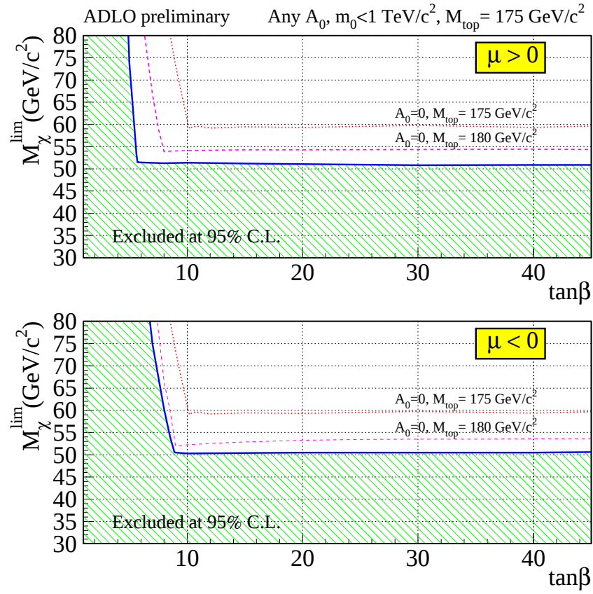
Figure 9.33: Limits on the mass of the lightest supersymmetric particle, derived from limits on m_{\frac{1}{2}} , from [39].
