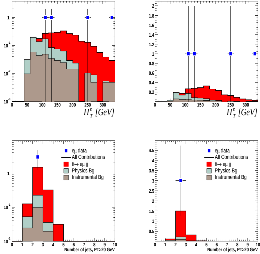
Figure 8.1: Data and backgrounds during topological selection to enhance t\bar{t} signal. Top, distribution in H_T^e , the sum of jet and electron transverse energies; prior to requirement H_T^e > 120 GeV, four candidates remain. Bottom, distribution in jet multiplicity, prior to requirement N_{jets} \geq 2 ; three candidates survive final selection. The same distributions are shown in a log scale ( left ) and linear scale ( right )
