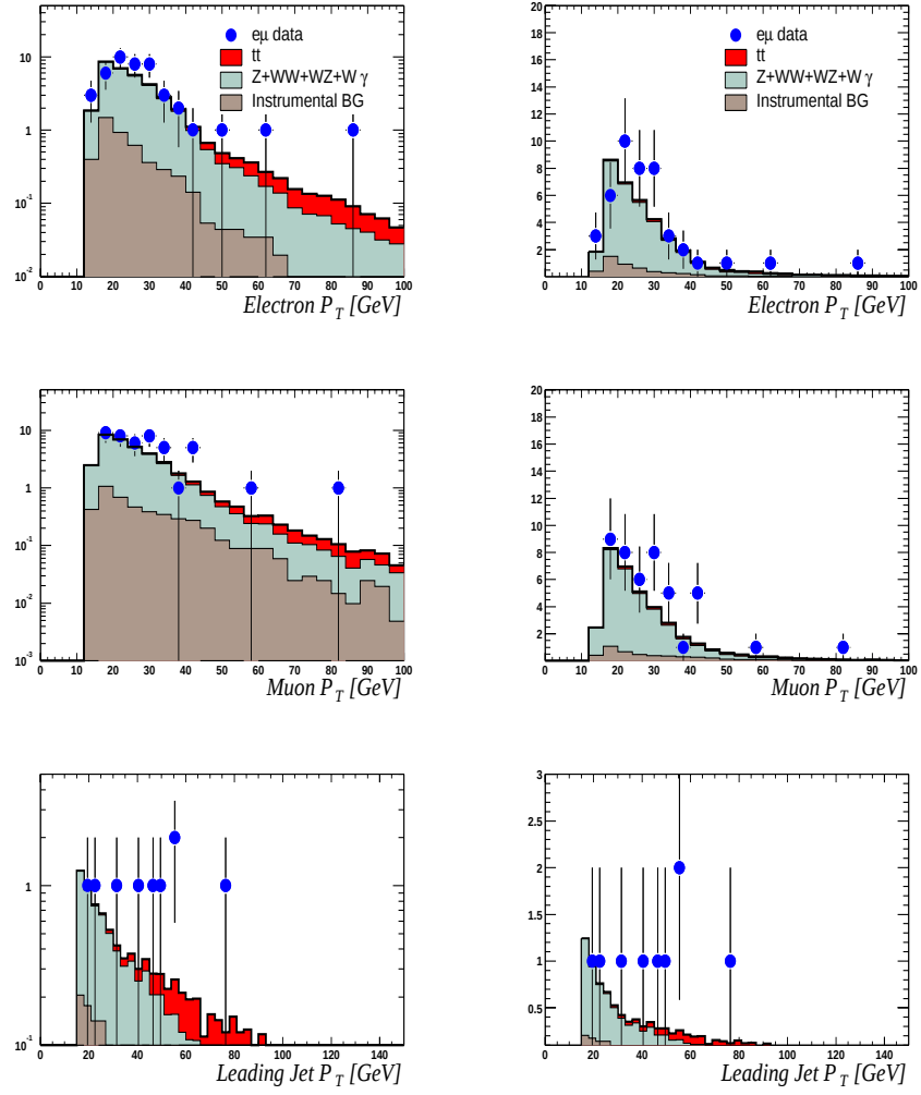
Figure 7.1: Transverse momentum of electrons and muons, in data and backgrounds. The same distributions are shown in a log scale ( left ) and linear scale ( right ).
