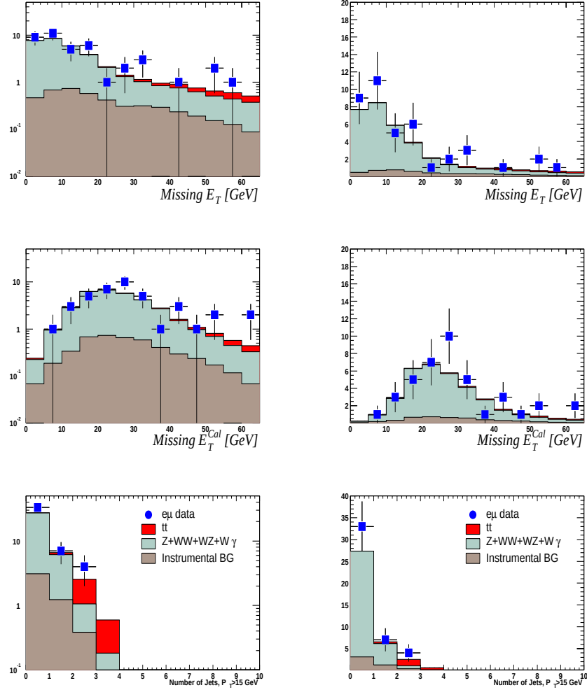
Figure 7.2: Missing transverse energy, calorimetric missing transverse energy and jet multiplicity for data and backgrounds. The same distributions are shown in a log scale ( left ) and linear scale ( right )
