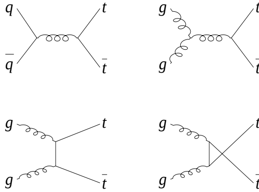
Figure 2.3: Feynman diagrams which represent leading order top quark pair production processes.
