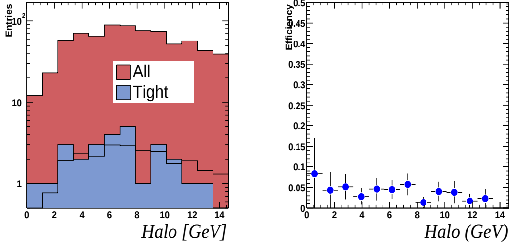
Figure 6.2: Simulated heavy flavor QCD events which contain a loose electron, and the subset of those events which contain a tight electron, ( left ). The rate at which loose electrons pass the tight cuts, as a function of the muon halo energy ( right ). Shown for the central calorimeter.
