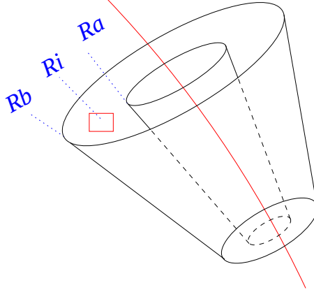
Figure C.2: A hollow cone in R , with inner edge R_a and outer edge R_b surrounding the muon. Calorimeter cell i is included in the cone if R_b > R_i > R_a .
