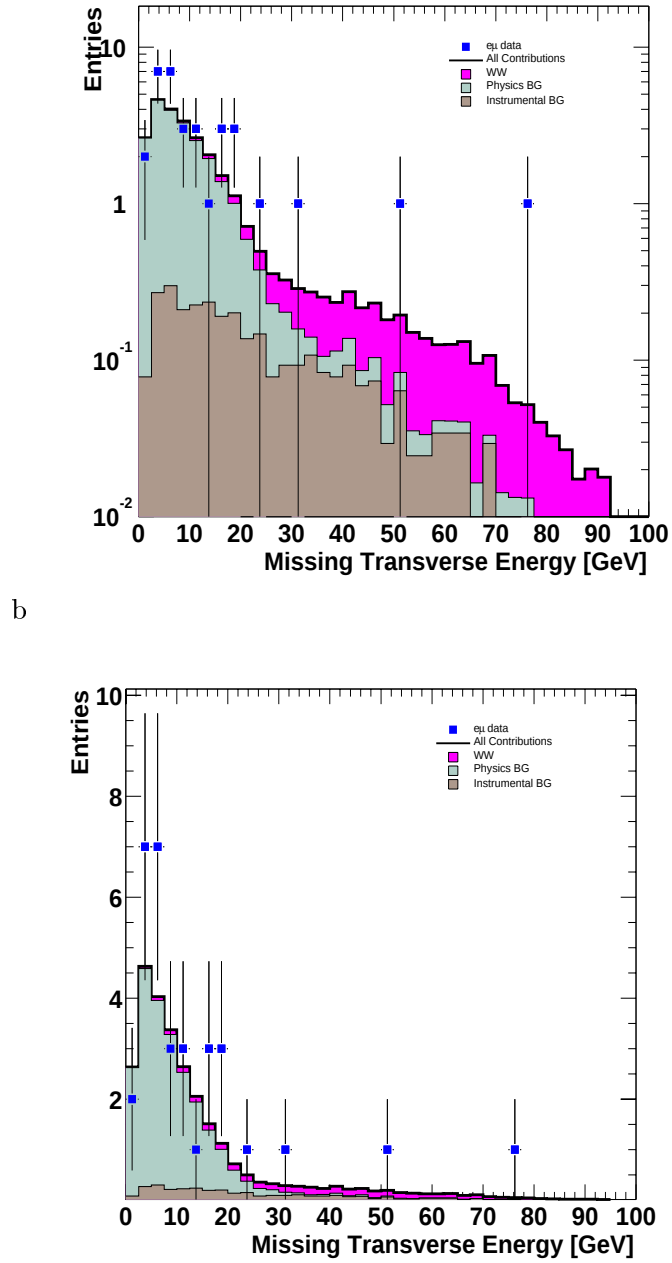
Figure 8.11: Data and backgrounds after requiring no reconstructed jets in order to enhance WW signal.
