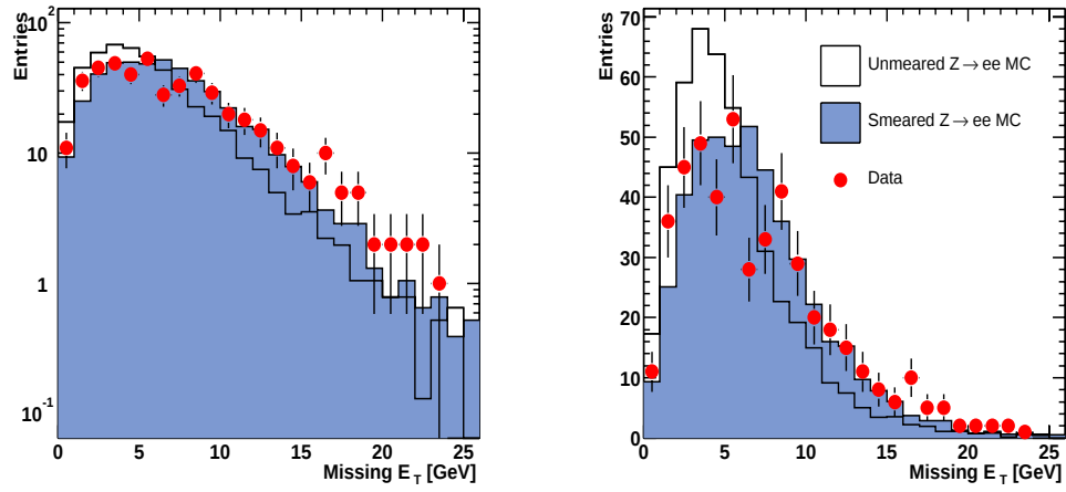
Figure 5.21: Agreement of missing transverse energy distributions in observed and simulated Z \rightarrow ee events. The distributions are shown in both log ( left ) and linear ( right ) scales.
