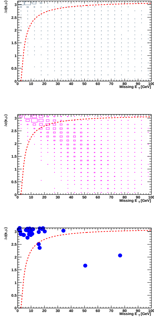
Figure 8.12: Distribution in Missing Transverse Energy and distance in \phi between leptons; physics backgrounds ( top ), expected signal ( middle ), and data ( bottom ).
