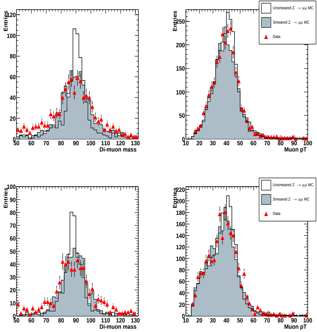
Figure 5.13: Agreement between simulated and real data in the di-muon invariant mass spectrum ( left ) and muon P_T spectrum ( right ) for central ( top ) and forward ( bottom ) muons.
