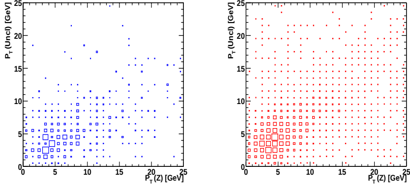
Figure 5.18: Correlations between the transverse momentum of the Z boson and the unclustered energy, in data ( left ) and in simulation ( right ).
