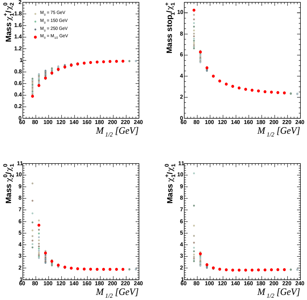
Figure 9.11: Variation in ratios of masses of relevant particles with mSUGRA parameter m_{\frac{1}{2}} . Various curves demonstrate a scan of m_0 in the region [75, 250] GeV.
