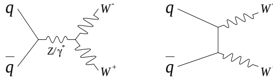
Figure 2.4: Feynman diagrams which represent leading order W boson pair production processes.
