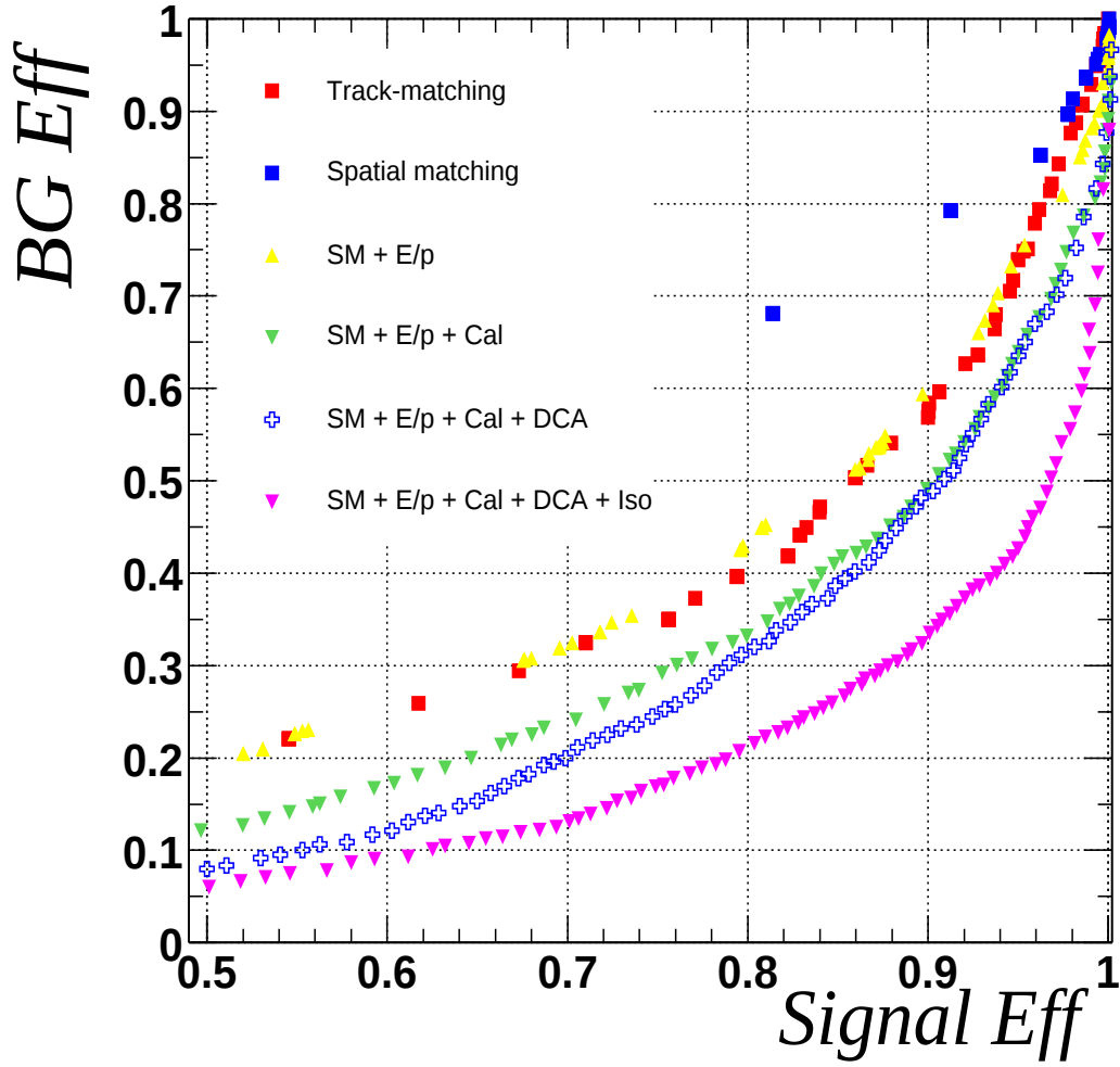
Figure B.6: Signal and background efficiencies in the central calorimeter for varying thresholds of the discriminants shown in Figure B.4. Note that the signal and background efficiencies assume a candidate track, the efficiency for which is detailed in Table 1.
