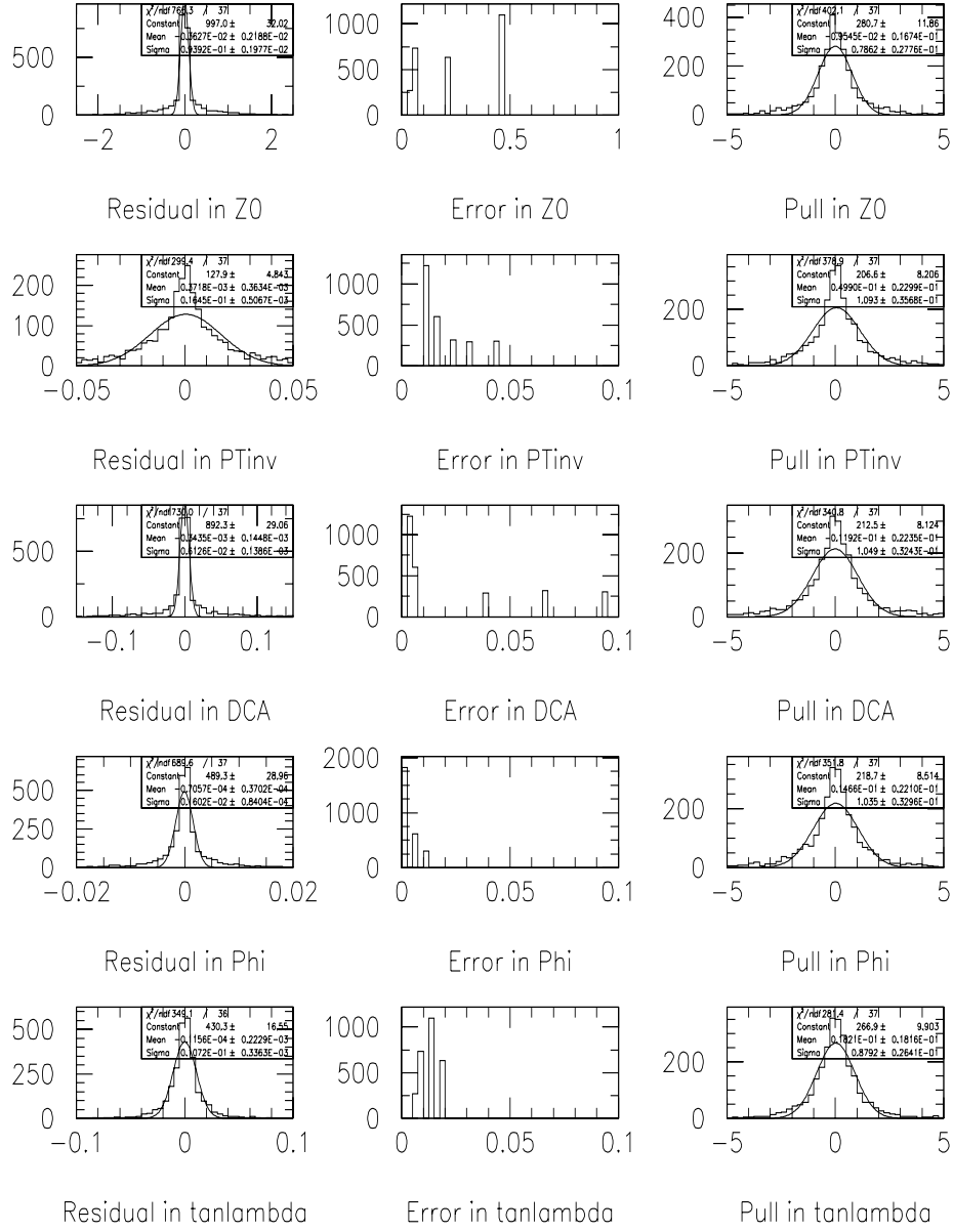
Figure A.21: Residual, error and pull for each of the five track parameters, for reconstructed tracks in 100 t\bar{t} \rightarrow lljj events.
