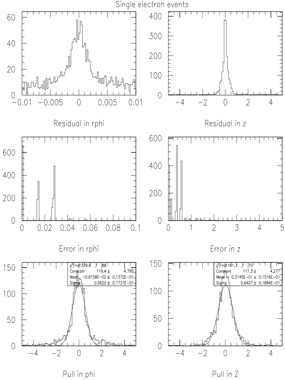
Figure A.22: Top shows hit to track residuals; middle shows cluster errors; bottom shows hit to track pulls. Left column shows quantities in r\phi ; right column shows quantities in z . From single electron Monte Carlo events.
