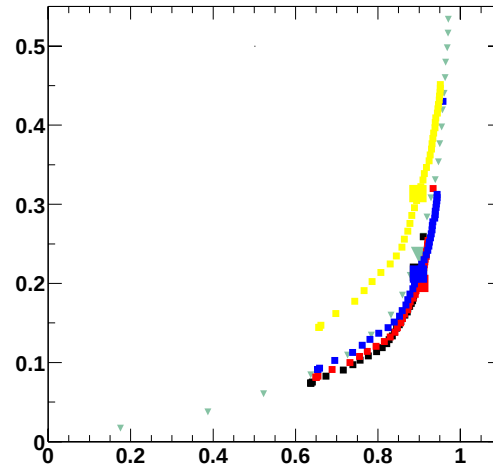
Figure C.11: Efficiency and purity curves for signal and background samples for track halo cuts, with different calorimeter halo cuts. Each curve begins at the calorimeter halo curve and describes the performance of the combined isolations.
