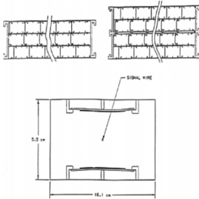
Figure 3.10: Drift tubes in the central muon system. An example tube ( below ) and stacking of tubes in the A ( upper left ) and BC ( upper right ) layers.
