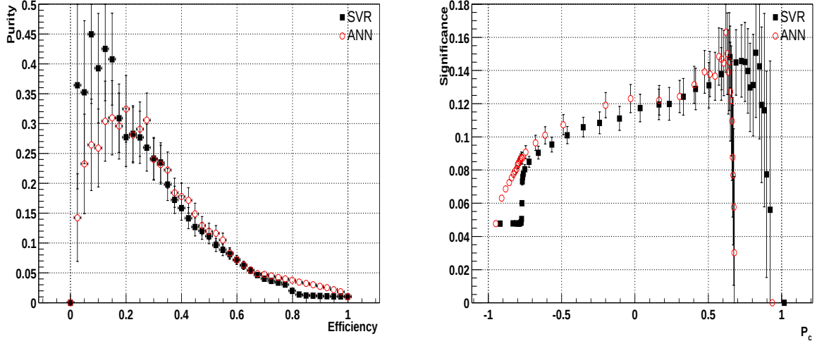
Figure D.3: Left, purity, p and efficiency, \varepsilon , as defined in the text, for support vector regression and an artificial neural network algorithm. Right, significance s for both algorithms. See text for detailed discussion.
