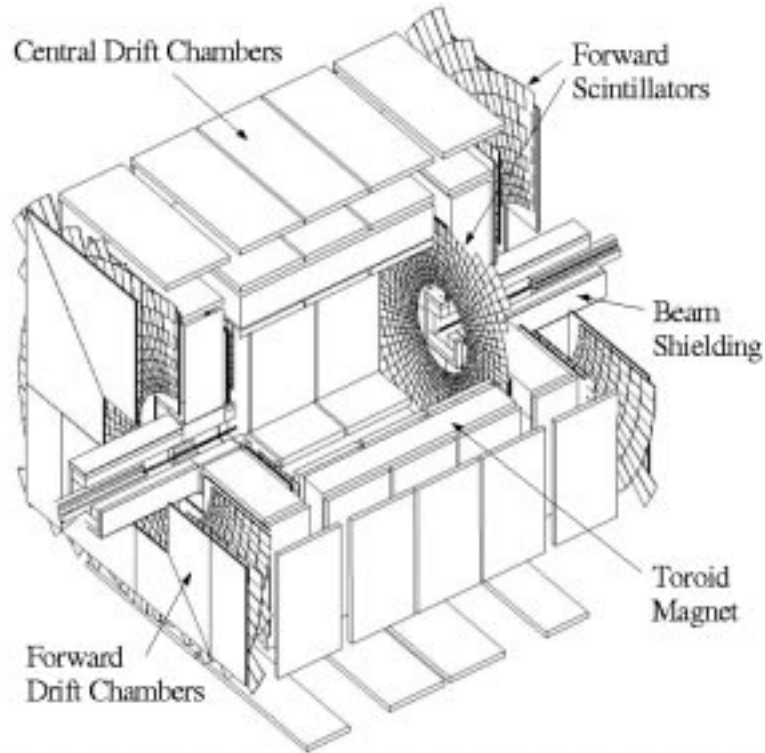
Figure 3.9: The DØ muon system.
