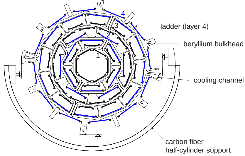
Figure 3.5: A view of the structure of the silicon microstrip tracker along the beam axis.
