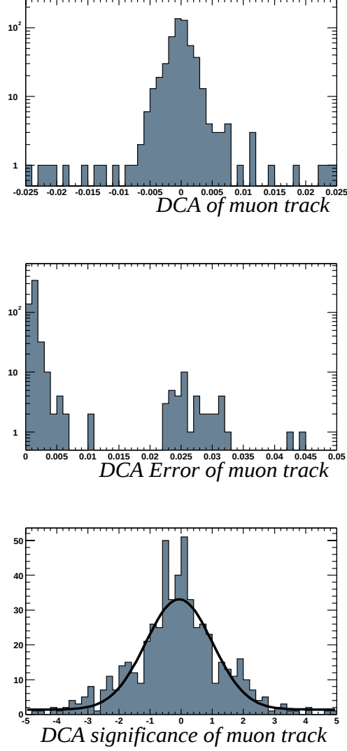
Figure 5.2: Muon distance of closest approach (DCA), ( top ), DCA error ( middle ), and DCA significance, ( bottom ) in t\bar{t} \rightarrow e\mu jj events.
