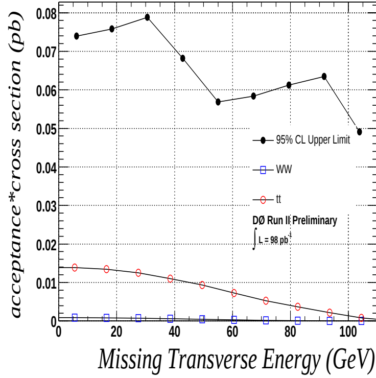
Figure 9.39: Upper limits on the production cross section of new physics in the e\mu jj channel, as a function of the cut on missing transverse energy in the event.
