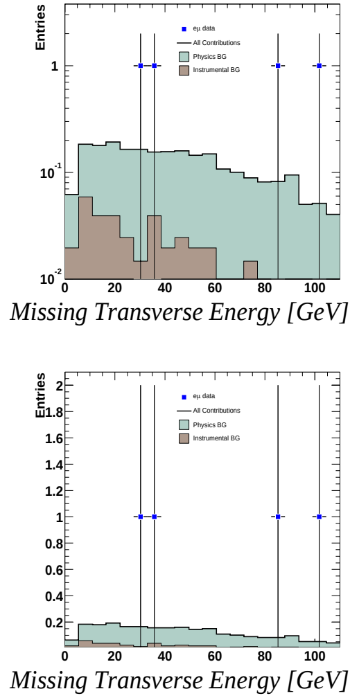
Figure 9.36: Missing transverse energy in e\mu events with two jets, for data and backgrounds in both log and linear scales.
