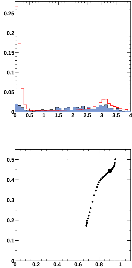
Figure C.3: Distribution of the jet to Muon distance in R (a). Efficiency and purity when R thresholds are varied (b).
