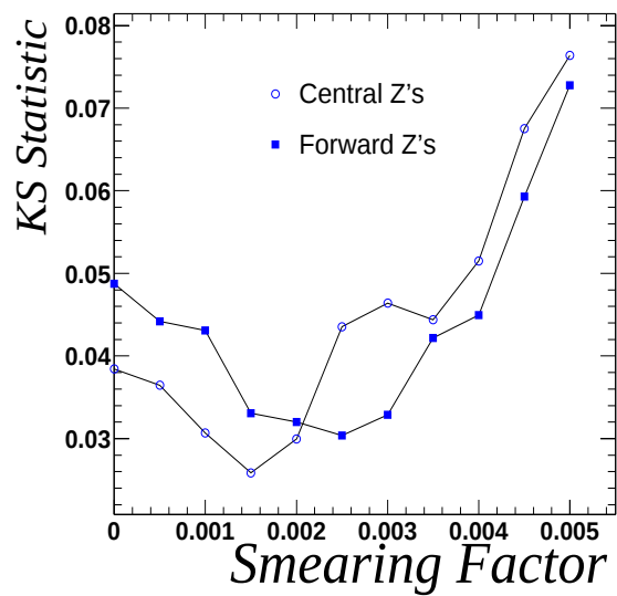
Figure 5.12: Kolmogorov-Smirnoff statistic between distributions of muon P_T spectrum in simulated and real data, for central and forward muons from Z \rightarrow \mu\mu events.
