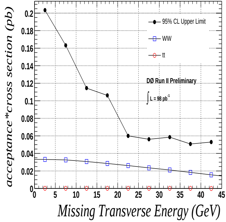
Figure 9.37: Upper limits on the production cross section of new physics in the e\mu channel, as a function of the cut on missing transverse energy in the event.
