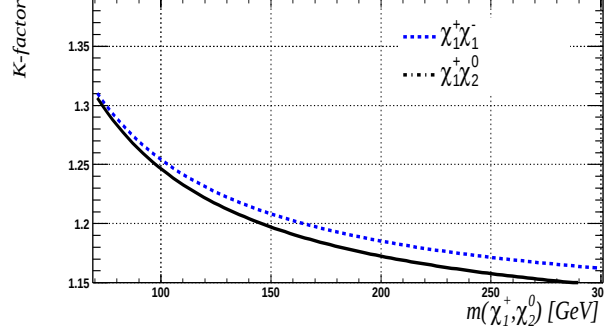
Figure 9.3: Next to leading order corrections to production cross sections for p\bar{p} \rightarrow \chi_1^+ \chi_2^0 and p\bar{p} \rightarrow \chi_1^+ \chi_1^- , adapted from [44].
