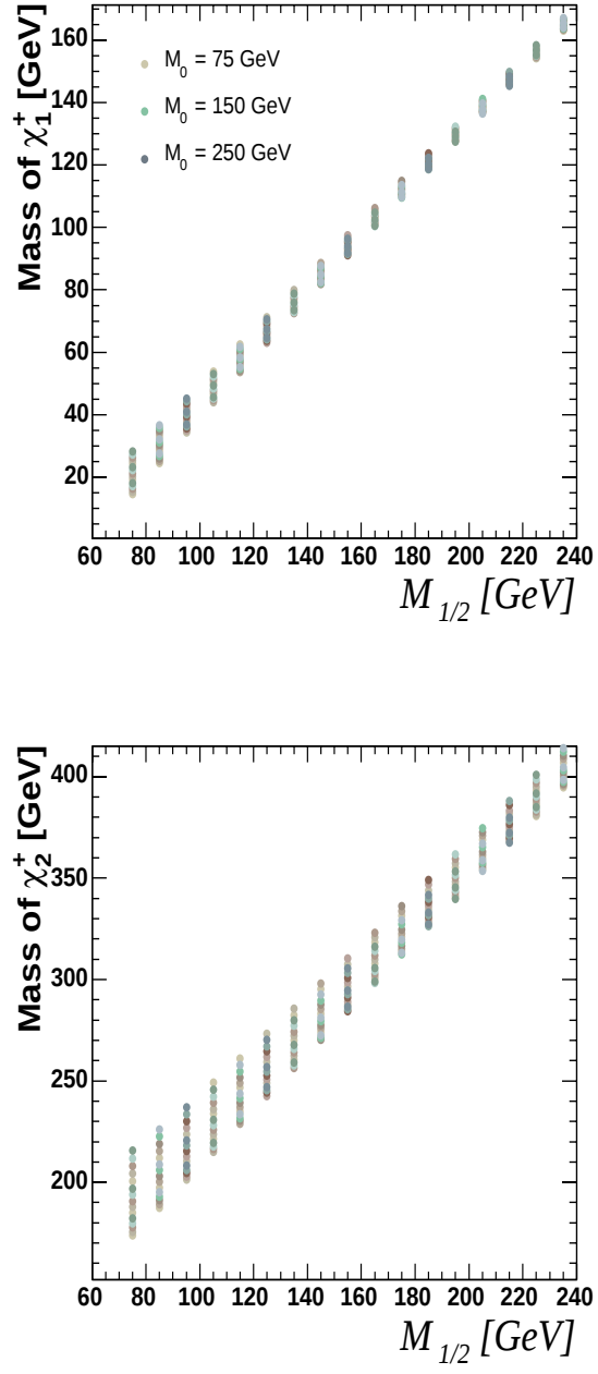
Figure 9.9: Variation in masses of \chi_{1,2}^\pm with mSUGRA parameter m_{\frac{1}{2}} . Various curves demonstrate a scan of m_0 in the region [75, 250] GeV.
