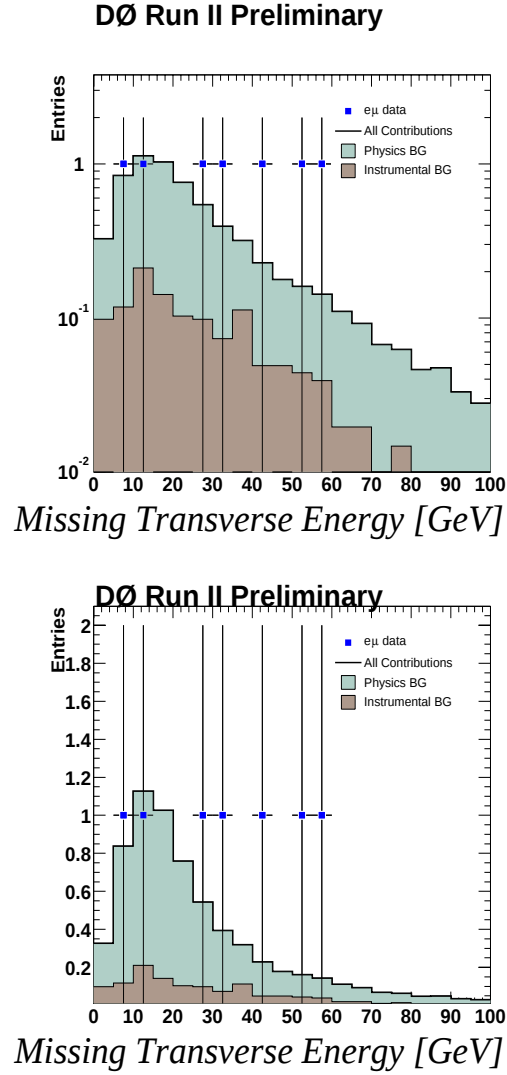
Figure 9.35: Missing transverse energy in e\mu events with a single jet, for data and backgrounds in both log and linear scales.
