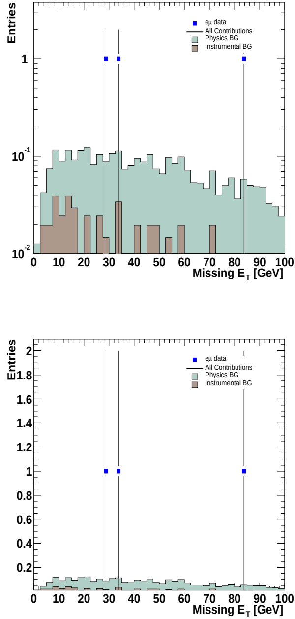
Figure 9.22: Missing transverse energy in e\mu events with 2 reconstructed jets, for data and backgrounds in both log and linear scales.
