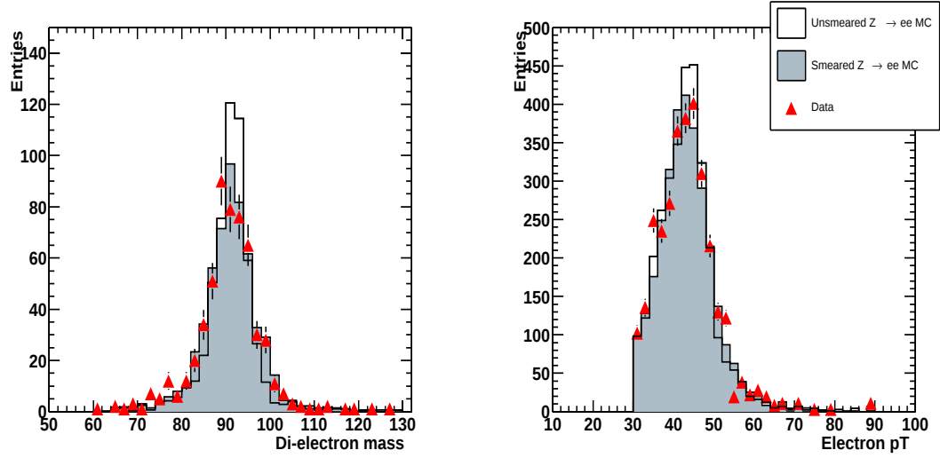
Figure 5.15: Agreement between simulated and real data in the di-electron invariant mass spectrum ( left ) and electron P_T spectrum ( right ) for central electrons.
