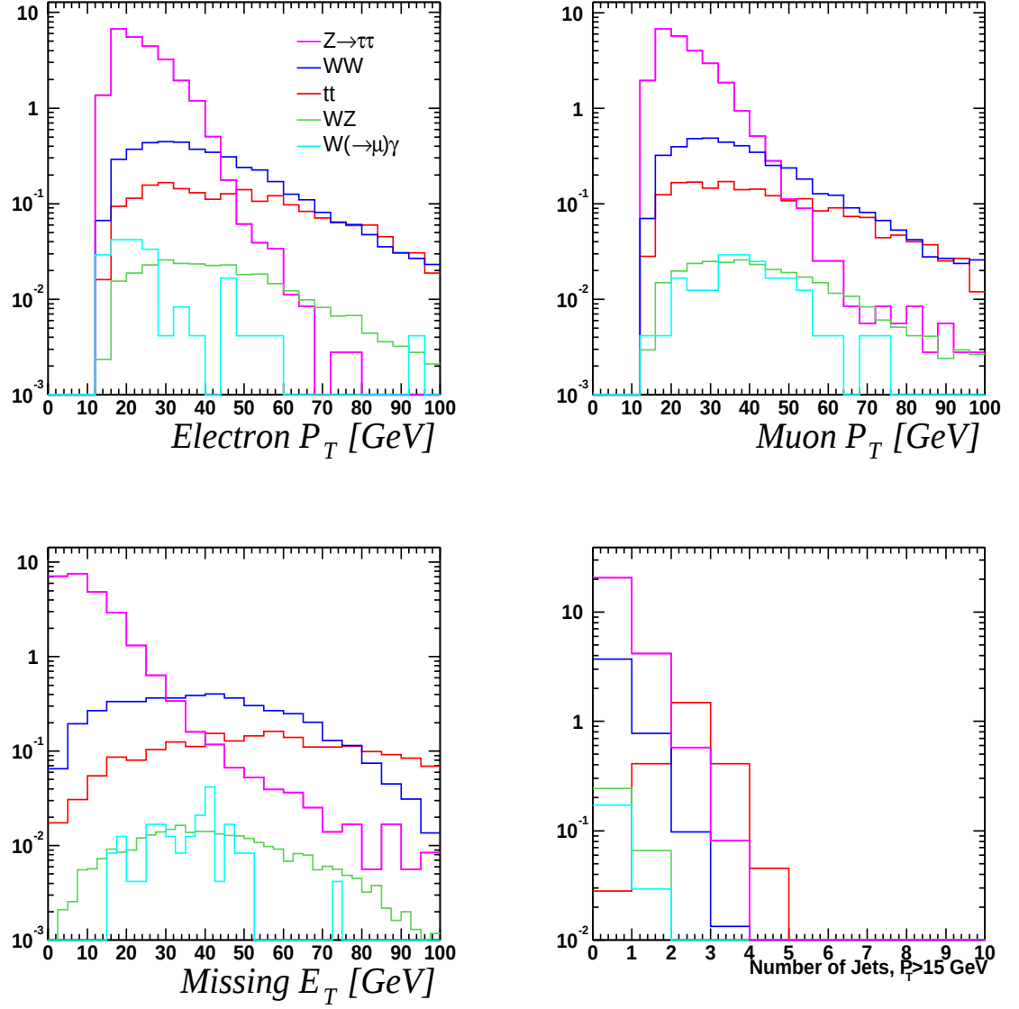
Figure 6.6: Distributions in lepton P_T , missing transverse energy and number of jets for the largest Standard Model contributions to e\mu .
