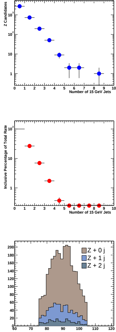
Figure 6.8: Jet multiplicity in Z \rightarrow \mu\mu events ( top ), inclusive percentage of total rate ( middle ) and invariant mass distributions for leading portions ( bottom ).
