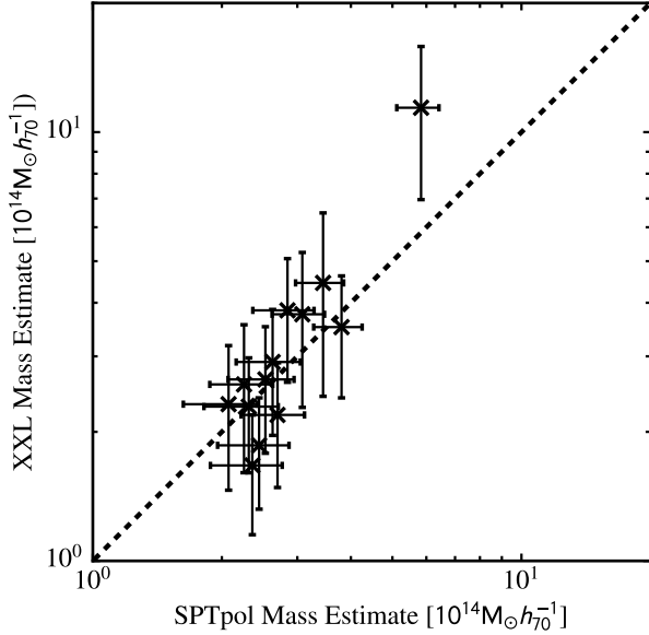
Figure 7. Galaxy cluster masses as measured by SPTpol and XXL. Both the XXL and SPTpol mass uncertainties are calculated using a scaling relation with an intrinsic scatter in the mass-observable relation (see §3.4), which leads to an X-ray or SZ mass uncertainty that is highly correlated between clusters in the sample. Only 13 of the 14 clusters found in both surveys are included, because the mass is not provided for one of the XXL clusters.
