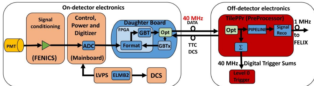
Figure 3 - Readout scheme for the upgrade, showing on- and off-detector electronics.
