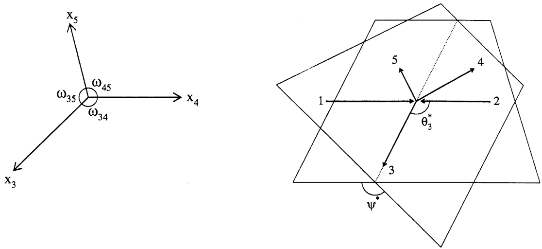
FIG. 1. Illustration of the topological variables: x_i , \omega_{ij} , \theta_3^* and \psi^* for the three-jet events.
