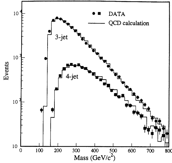
FIG. 3. The mass distributions of the selected three- and four-jet events before the mass requirement. The QCD matrix element calculations are normalized to the data.
