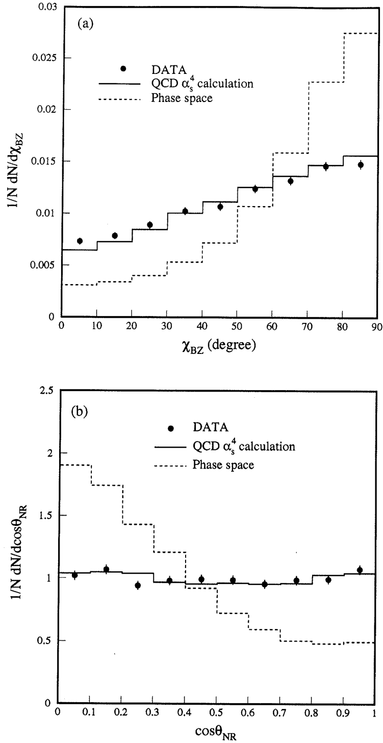
FIG. 11. The distribution of the angle between the planes of (a) the two leading jets and the two non-leading jets and (b) the momentum vector differences of the two leading jets and the two non-leading jets, for four-jet events in their center-of-mass system. Only statistical errors are shown. The RMS of the fractional differences is 5.7% for \chi_{BZ} and 4.1% for \cos\theta_{NR} . The estimated systematic uncertainty on the measurement is 6%. The data are also listed in Table VIII.
