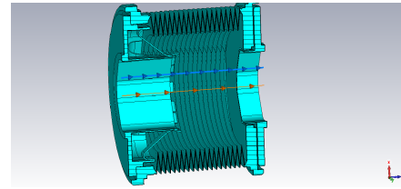
Figure 2: The simplified model of bellow for CST simulations. The orange line is the beam and blue line is the integration path.
