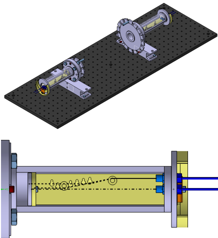
Figure 1: top :The representative picture of measurement setup. down: The endcaps of the measurement setup.
