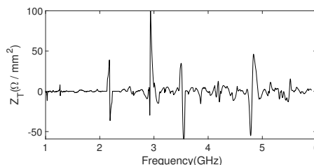
Figure 5: The transverse impedance results of the bellow performed with 1 mm wire with 5 different offset and extracted from moving wire data by fitting parabola.
