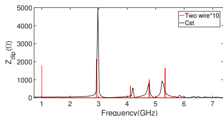
Figure 4: Two wire measurements which performed with 1 mm wire comparison with the CST simulation results.
