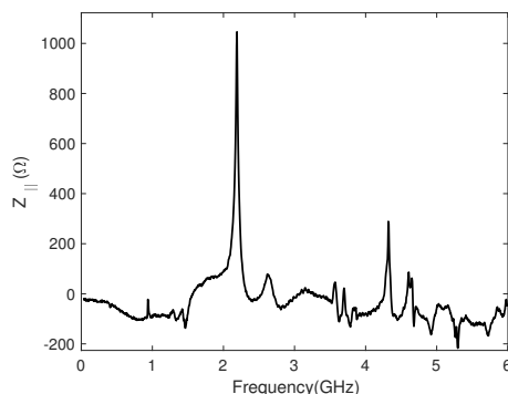
Figure 3: Longitudinal impedance which is measured on axis with 1 mm wire.
