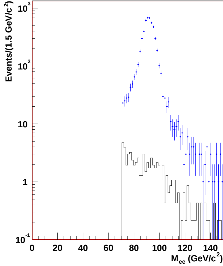
Figure 7.3: Invariant mass distributions for data (points with error bars) and estimated QCD background (histogram) in the mass region 70 < M_{ee} < 150 \text{ GeV} with 1.5 \text{ GeV} bin width.
