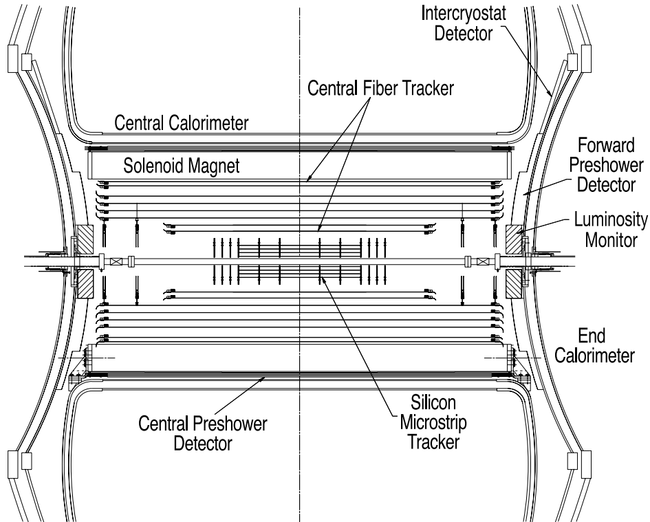
Figure 2.3: The central tracking system.
