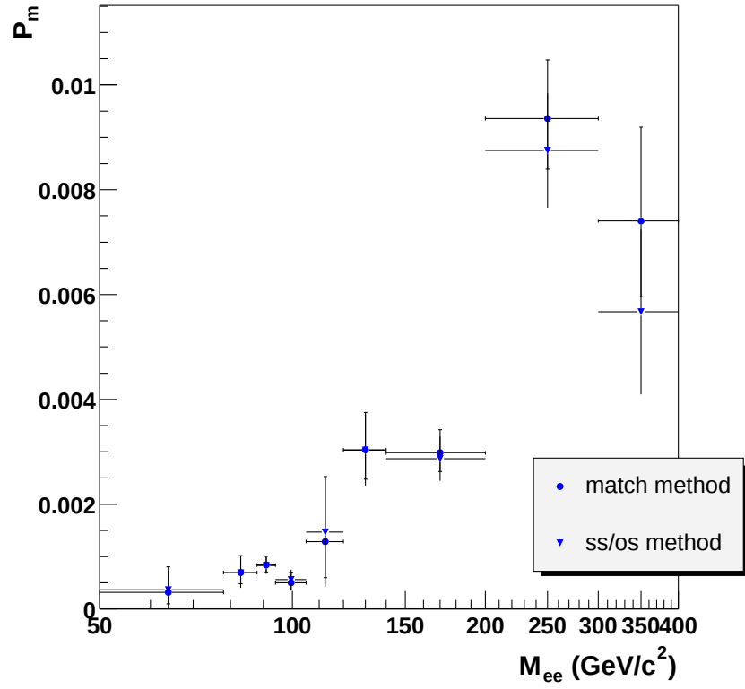
Figure 8.22: Monte Carlo charge mismeasurement probability vs. M_{ee} for match method and same-sign/opposite-sign method. The probabilities are not normalized to data.
