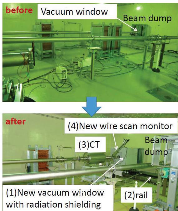
Figure 3: Pictures of beam transport line near beam dump (we call 100-deg beam dump, shown in Fig. 3(1)) before and after improvements in 2014 summer shut down.
