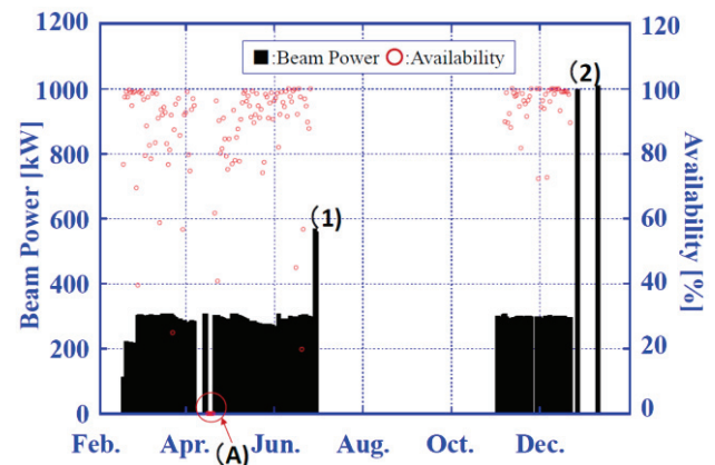
Figure 1: Output beam power and availability of the RCS from February 2014 to January 2015. Black line shows beam power and read circle shows availability. Beam studies were performed at the number (1) and (2) shown in this figure. Availability was zero at period of (A) shown in this figure due to failure of an oil cooling pump in the bending magnet choke transformer.
