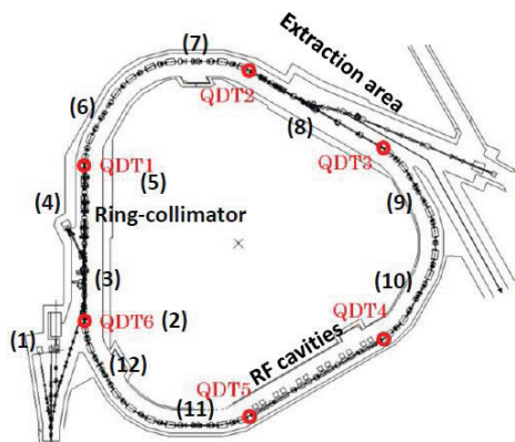
Figure 2: Residual does measurement points and new correction magnets installation points at RCS.
