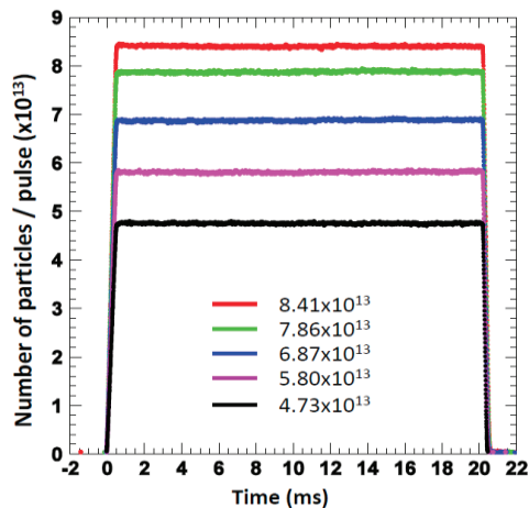
Figure 4: Circulating beam intensity over 20 ms from injection to extraction measured by current transformer (DCCT). Horizontal shows time and vertical is the number of particles per pulse measured by the DCCT.
