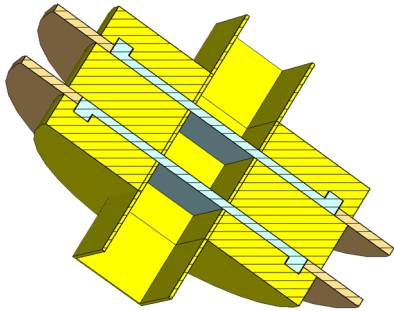
Figure 5: Two-section 80 kV DC break with the composite insulator.
