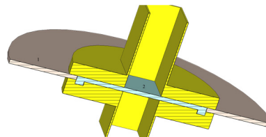
Figure 3: 40 kV DC break design with composite dielectric. (1) Alumina. (2) PTFE.
