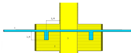
Figure 1: 40 kV DC break design with PTFE. (1) Insulator. (2) Waveguide flange. (3) WR340 waveguide.
