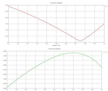
Figure 2: Scattering parameters of the simple 40 kV DC break section.
