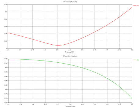
Figure 4: Scattering parameters of the 40 kV DC break section with composite dielectric.
