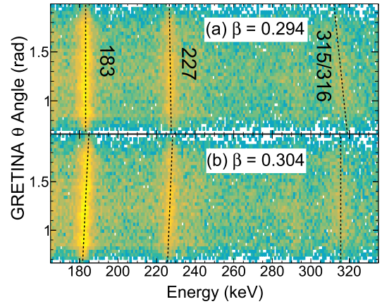
Fig. 3. Doppler-corrected \gamma -ray spectra for ^{79}\text{Y} against the detected polar angle of GREINA, corrected with the indicated recoil velocities. It is clear that a slower recoil velocity is required to correct the 183-keV transition, panel (a), compared to that needed to optimise transitions such as the 315/316-keV decays, which predominantly occur whilst the recoil is within the target, panel (b). The latter transitions are expected to decay from shorter lived (few ps) states. The dashed black lines are to guide the eye.
