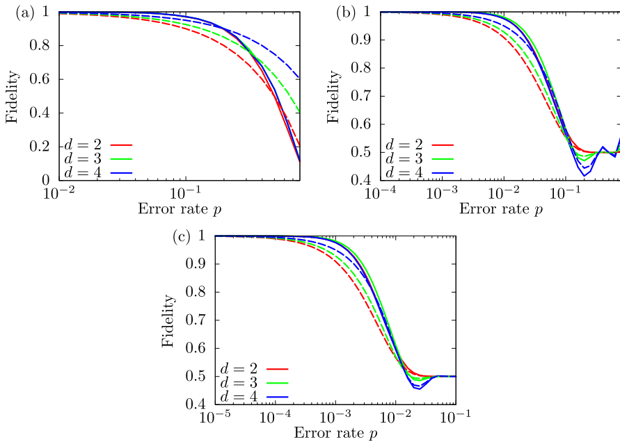
Fig. 12 Process fidelity for the Z-type error model. Solid lines and dashed lines depict results with and without QEC, respectively. We use states at a \tau = 1 , b \tau = 10 , and c \tau = 100 . The initial state is the maximally entangled state
