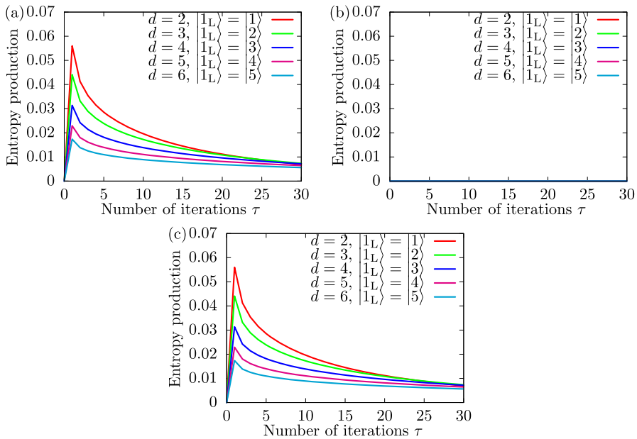
Fig. 6 Entropy production of a the encoding subspace, b the nonencoding subspace, and c the total space for the Z-type error model. The initial state is the maximally entangled state. The maximally polarized state is used: |0_L\rangle = |0\rangle and |1_L\rangle = |d-1\rangle , where d is the number of energy levels
