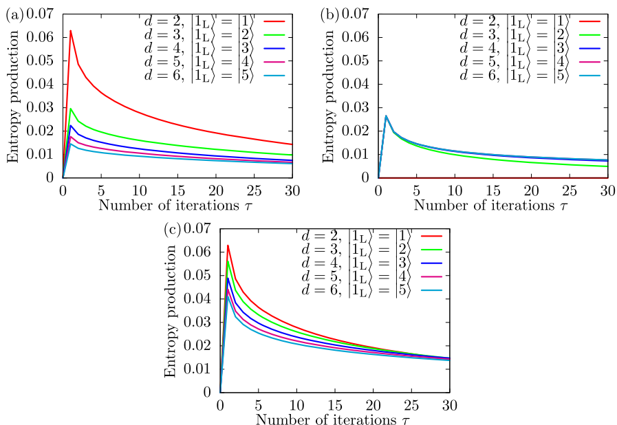
Fig. 8 Entropy production of a the encoding subspace, b the nonencoding subspace, and c the total space for the X' -type error model and Z-type error model. The initial state is the maximally entangled state. The maximally polarized state is used: |0_L\rangle = |0\rangle and |1_L\rangle = |d-1\rangle , where d is the number of energy levels
