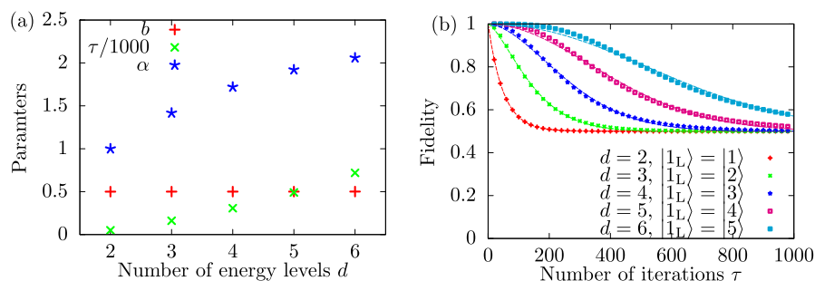
Fig. 5 Estimated parameters of the fitted Kohrausch function for the process fidelity in the case of the X' -type error model. a Dependence of b , \tau , and \alpha on d . b Raw data and fitting curves. The original data are shown in dots and the fitting curves are depicted via dashed lines. We have varied |1_L\rangle from |1\rangle to |5\rangle , while |0_L\rangle is fixed to |0\rangle
