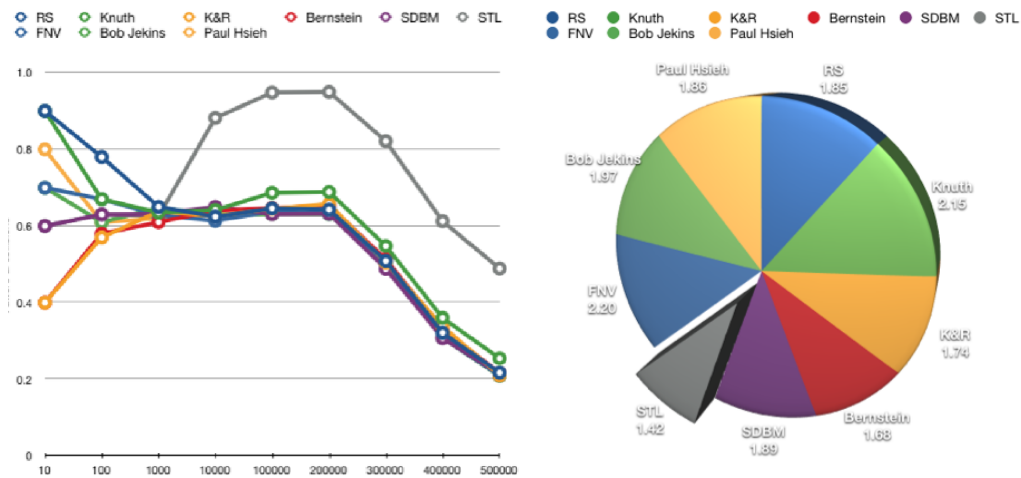
Figure 4. Test results for different hashing functions. The tests have been performed on a set of real ATLAS histogram names. Left: the collisions factor as a function of the hash table size for different hashing functions, smaller factor is better. Right: time spent (a.u.) by different algorithms, smaller numbers are better. The Bernstein algorithm has good performances while keeping small the number of collisions.
