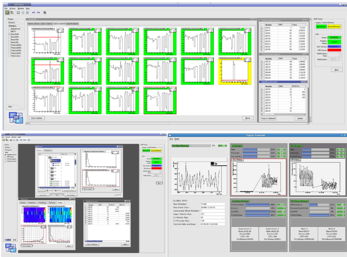
Figure 3. Some examples of plug-ins. The top figure shows the MDI interface with several other plug-ins running. In addition to canvases a user-defined plug-ins shows, in a tabular form, the electronic channel with high noise. Bottom left figure shows another instance of OHP with the histogram browser, a table plug-in and a canvas with several drawing options configured. Bottom right picture shows the main GUI of the TriP plug-in, this is used to display trigger information.
