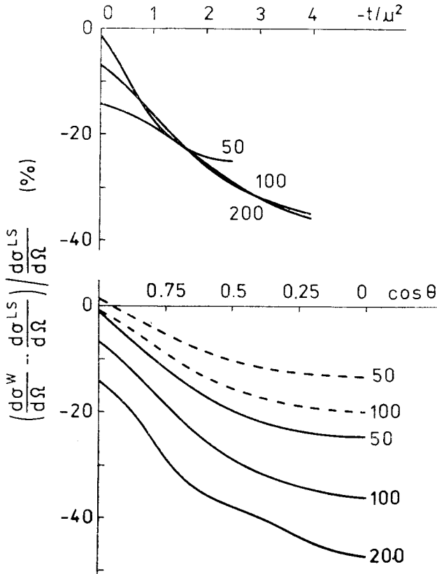
Fig. 1. The relative difference of the differential cross sections for the same value of the coupling constant. The numbers associated with curves denote the laboratory energy in MeV. The broken curves correspond to the local modification
