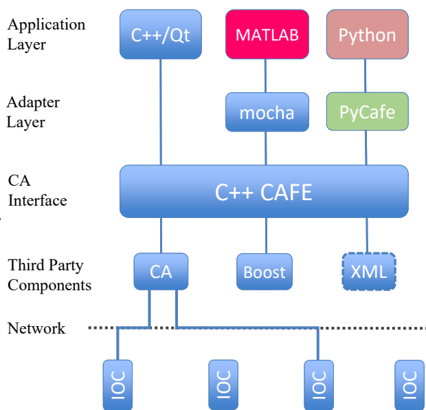
Figure 1: The software architecture for the integration of CAFE to high-level applications. The mocha and PyCafe adapters have been written in C++ and Cython, respectively.
