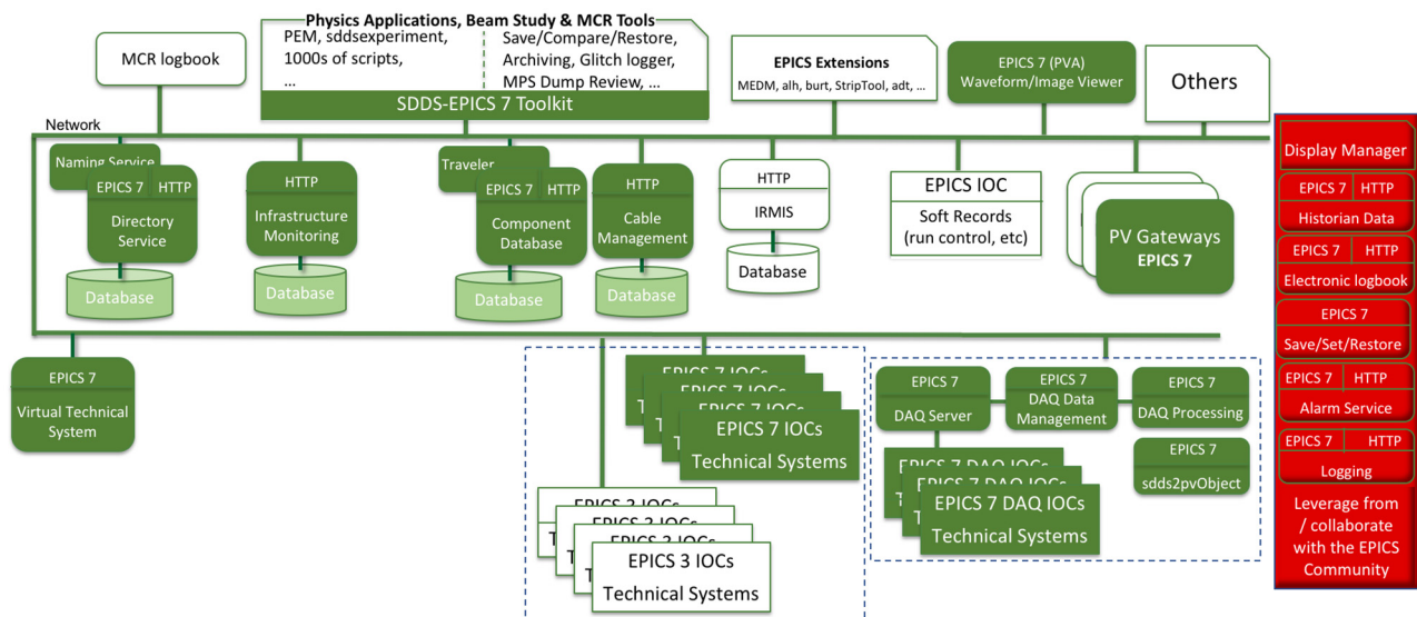
Figure 3: The control architecture plan of APS, showing the typical usage model enabled by EPICS now - a three tier system of front end computers (IOCs), middleware services, and intelligent clients for both display and machine analysis. Notably at APS, EPICS 7 is used to publish the results of the SDDS physics analyses package on the network.
