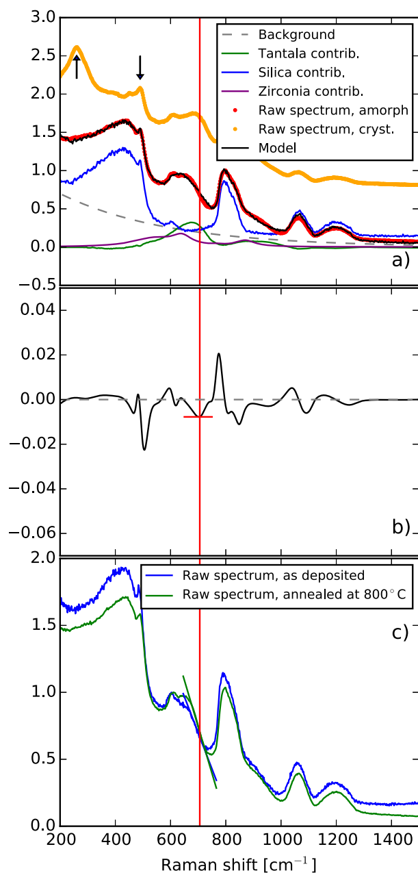
Figure 22. Measured Raman spectra of HiPIMS/RF-MS \text{Ta}_2\text{O}_5\text{--ZrO}_2 thin films and their analysis: (a) example of a spectrum obtained for an amorphous sample with, super-imposed, a model resulting from different contributions summed together (see text for details); (b) derivative of the raw Raman spectrum, smoothed using bi-cubic splines; (c) raw, normalized spectrum of the same sample, as-deposited and annealed. The slopes extracted using the derivative method shown in (b) are represented by straight lines. The vertical red line across all panels is the position of the minimum of the first derivative of the Zr contribution shown in (a).
