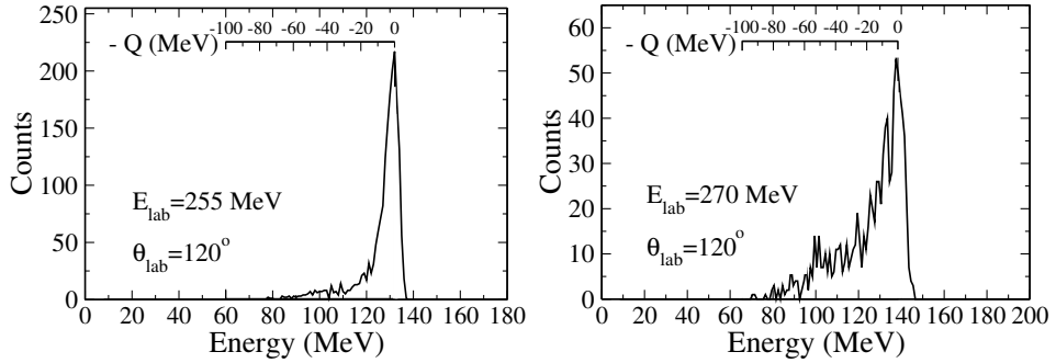
Fig. 2. Measured energy spectra for the ^{48}\text{Ti}+^{232}\text{Th} system at E_{\text{lab}} = 255 MeV and 270 MeV (left and right panel, respectively) along with the reaction Q value scale for the inelastic exit channel.
