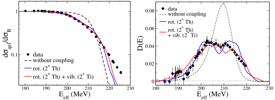
Fig. 3. Left panel: Experimental QE excitation function and its fit from the coupled-channel calculation. Right panel: Experimental barrier distribution and its fit from the coupled-channel calculation for the ^{48}\text{Ti}+^{232}\text{Th} system.
