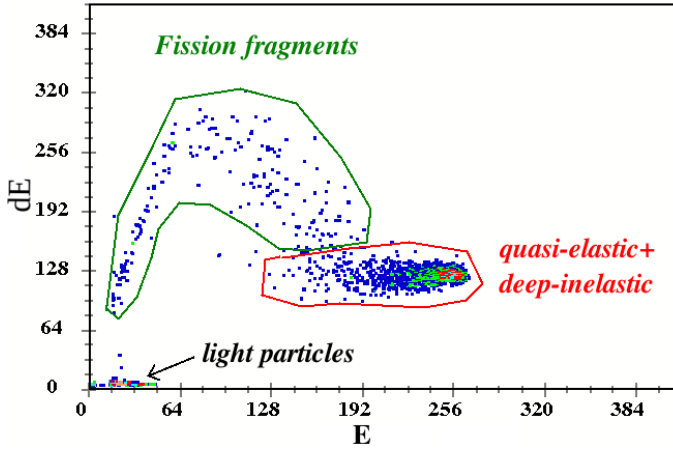
Fig. 1. Online 2D spectra (energy loss versus residual energy) of the ^{48}\text{Ti}+^{232}\text{Th} system for E_{\text{lab}} = 260 MeV and \theta_{\text{lab}} = 120^\circ relative to the beam direction.
