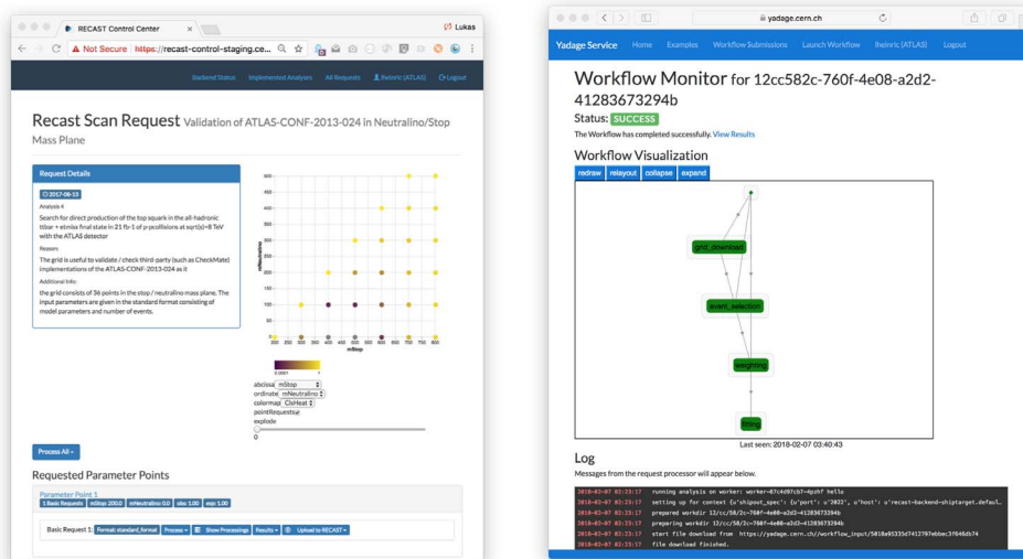
Figure 83. Left: web-based interface for the RECAST back end for and experiment that presents the requested parameter points and color-coded results. Right: an experiment-internal reinterperation executing on the distributed infrastructure built by CAP and RECAST.
