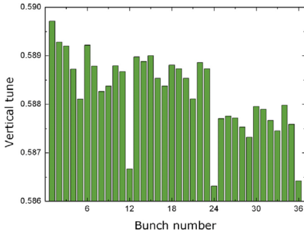
Figure 2: Vertical tunes of the 36 proton bunches measured by the DTM at the end of the store # 5301.
