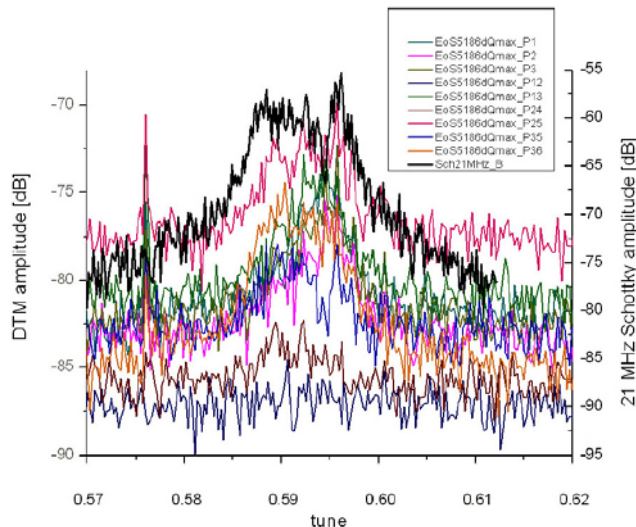
Figure 4: Spectrum from 21.4 MHz Schottky monitor and DTM (for selected proton bunches) measured at the end of the store # 5186.
