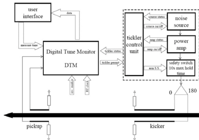
Figure 5: Schematic of the Digital Tune Monitor and Tickler.
