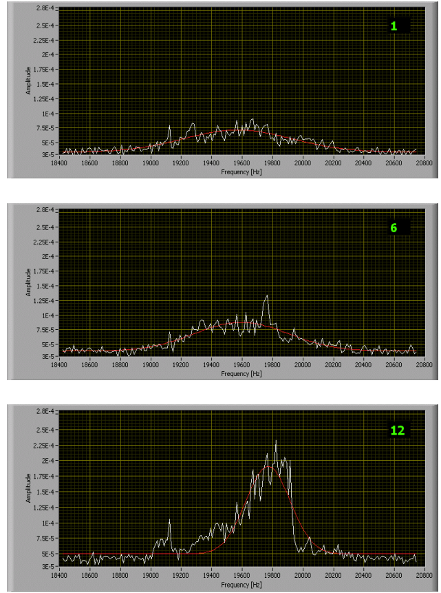
Figure 3: Spectra reported by the DTM for the first, the sixth and the twelfth bunch. Data taken at the end of store #5301.
