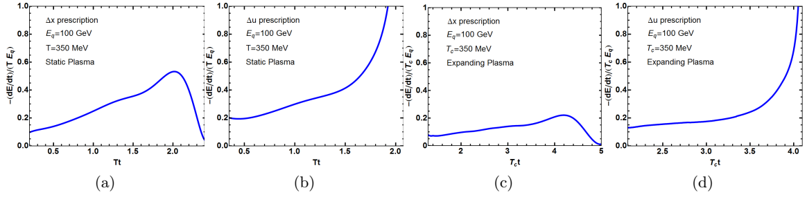
Figure 2: The instantaneous energy loss of a light quark jet, as a function of time in the AdS-Sch metric using the (a) \Delta x -prescription of jet and (b) \Delta u -prescription of jet and JP metric using the (c) \Delta x -prescription of jet and (d) \Delta u -prescription of jet. The normalization constant E_q = 100 GeV is the energy of half of the string and T = 350 MeV is the temperature of plasma. Our jet definition reconstruct the Bragg peak in the energy loss rate of light quark in both static and expanding plasma.
