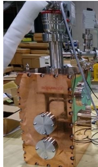
Figure 6: Assembled cavity after second machining.
