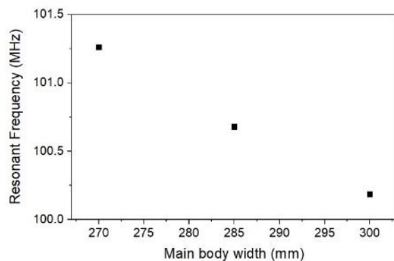
Figure 3: Main body width and resonant frequency.
