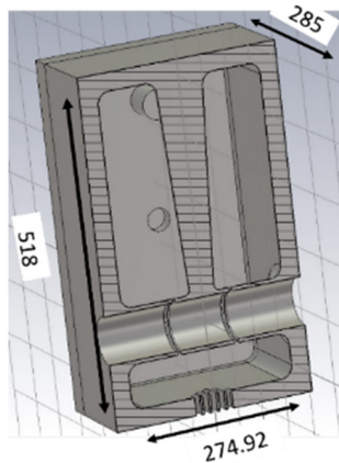
Figure 2: Cavity inner dimension.
