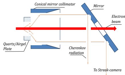
Figure 3: Scheme of Cherenkov sensor for measuring of longitudinal beam profile.
