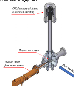
Figure 2: Scheme of fluorescent sensor in SKIF linac.
