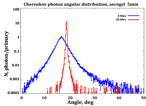
Figure 5: The angular distributions of Cherenkov photons emitted by 3 MeV and 50 MeV electron beam passing through 5 mm aerogel.
