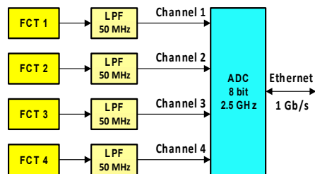
Figure 8: Block diagram of beam charge measurements.
