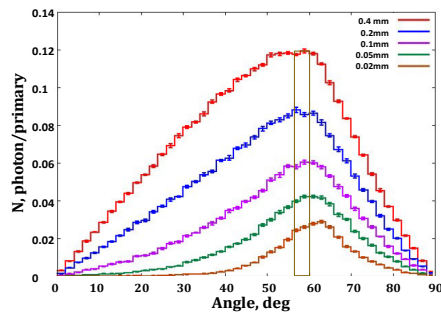
Figure 4: Cherenkov radiation angular distribution of 0.6 MeV electrons beam through different quartz plate.
