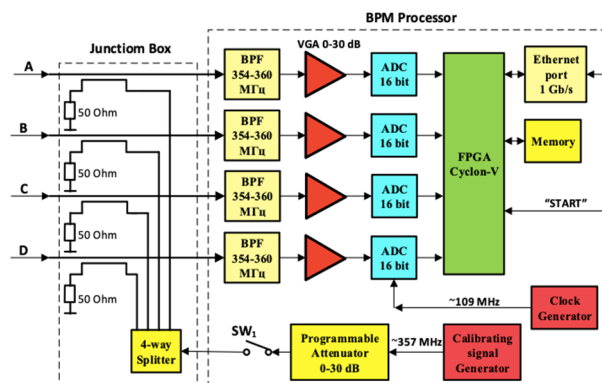
Figure 10: A functional diagram of electronics for one BPM.
