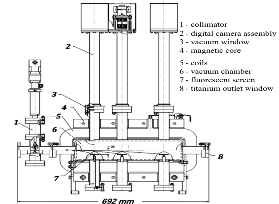
Figure 6: Layout of magnet spectrometer.
