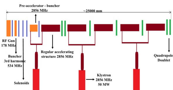
Figure 1: Layout of SKIF linear accelerator.
