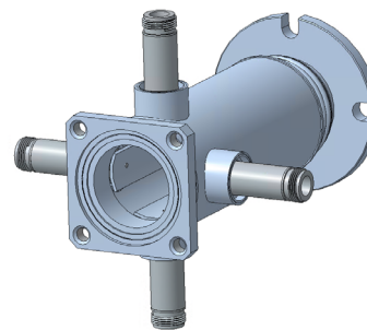
Figure 9: Stripline type BPM.
