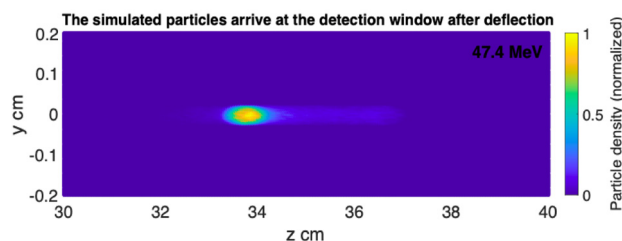
Figure 7: The simulated longitudinal profile of the beam.
