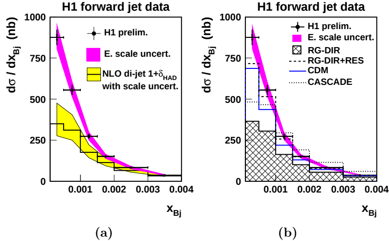
Fig.1. Forward-jet cross section [1] and the predictions of (a) DISENT and (b) RAPGAP (RG), ARIADNE (CDM) and CASCADE.
