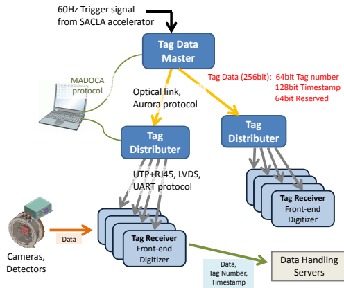
Figure 2: A schematic view of the tag data supply system.
