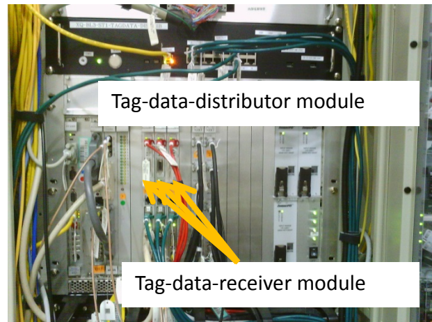
Figure 4: An example of the installation of tag-data-distributor and tag-data-receiver modules.
