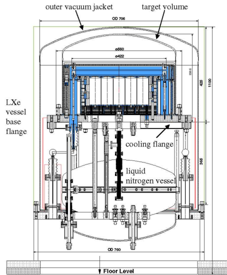
Fig. 9. ZEPLIN III detector.
