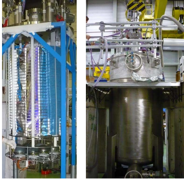
Fig. 13. Left: Inner ArDM detector. In the image the installed PMTs, field shaping rings and the external part of the wavelength shifter sheets can be seen. Right: ArDM vessel. The empty flange on top connects the vessel with the purification and recirculation systems.
