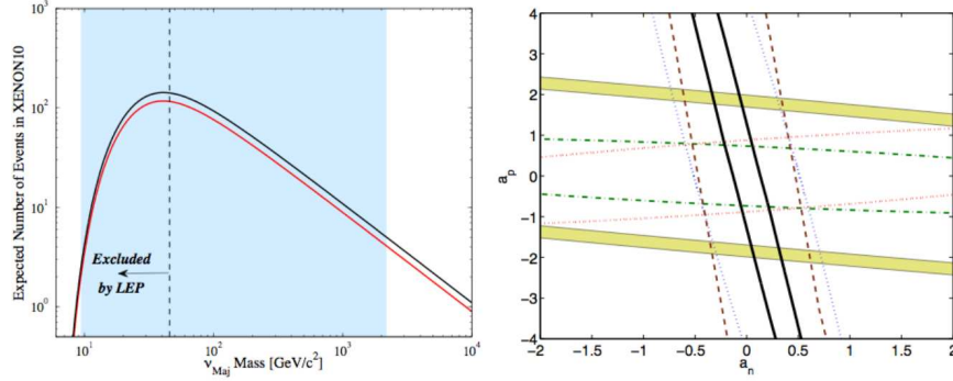
Fig. 4. Left: Predicted number of events in XENON10 for a heavy Majorana neutrino with standard weak interaction as a function of the neutrino mass, using the main (upper, black) and alternate (lower, red) form factors. The light shaded area shows the excluded mass region at 90% C.L. Right: Regions allowed at the 90% C.L. in a_n - a_p parameter space for a WIMP mass of 50 GeV/c 2 . The combined limit from ^{129}\text{Xe} and ^{131}\text{Xe} is shown as a dark solid curve (using the main form factor). The exteriors of the corresponding ellipses are excluded, the common space inside the ellipses being allowed by the data. We also show the results obtained by KIMS (dot-dashed), COUPP (horizontal ellipses) and CDMS (dotted), ZEPLIN-II (dashed) and the DAMA evidence region (vertical ellipses).
