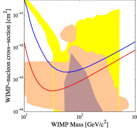
Fig. 2. Spin-independent WIMP-nucleon cross-section upper limits (90% C.L.) versus WIMP mass. Shown curves are for the previously best published limit (upper, blue) and the current work (lower, red). The shaded area is for parameters in the MSSM models (light-grey, yellow), the Constrained MSSM models (grey, marron) and CMSSM with the recent improved Standard Model prediction for the branching ratio of \bar{B} \Rightarrow X_s \gamma (dark-grey, brown).
