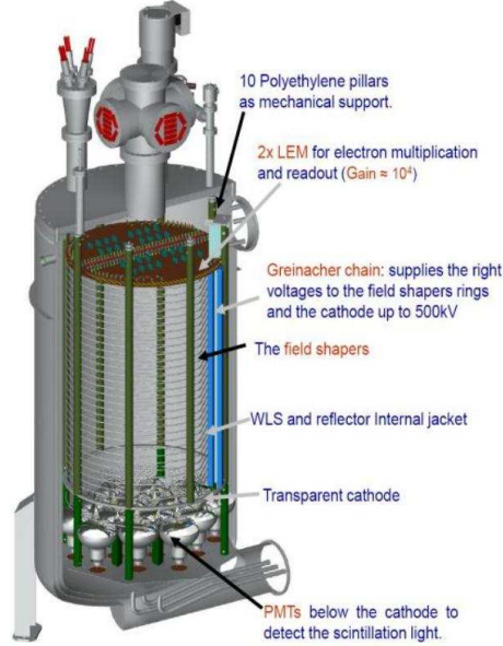
Fig. 12. Schematic of the ArDM detector. Charge and light produced in interactions are readout with a LEM and 14 PMTs. An electric field, uniformized by field shaping rings is used to drift the charge up to the LEM.
