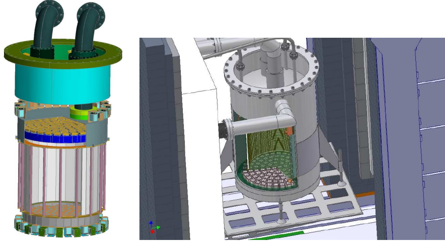
Fig. 6. Schematic of the XENON100 TPC (left) and the cryostat inside the shield (right).
