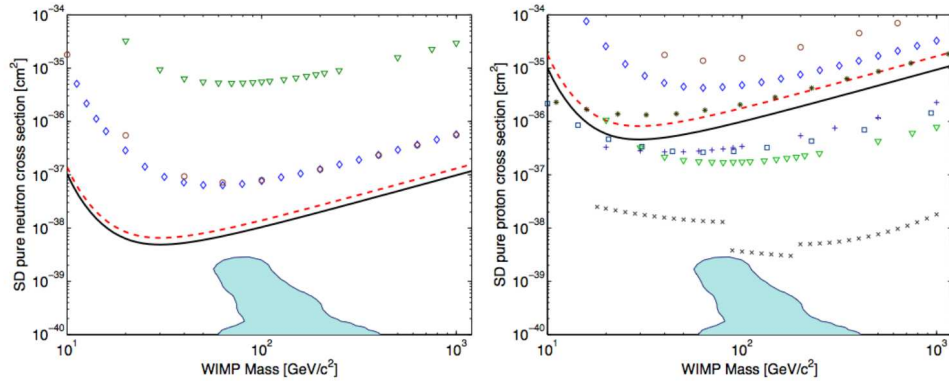
Fig. 3. Combined 90% C.L. exclusion Limits for ^{129}\text{Xe} and ^{131}\text{Xe} for pure neutron (left) and pure proton (right) couplings (solid curves). The dashed curves show the combined Xe limits using the alternate form factor. Also shown are the results from the CDMS experiment (diamonds), ZEPLIN-II (circles), KIMS (triangles), NAIAD (squares), PICASSO (stars), COUPP (pluses) and SuperK (crosses). The theoretical regions (constrained minimal supersymmetric model) are also shown.
