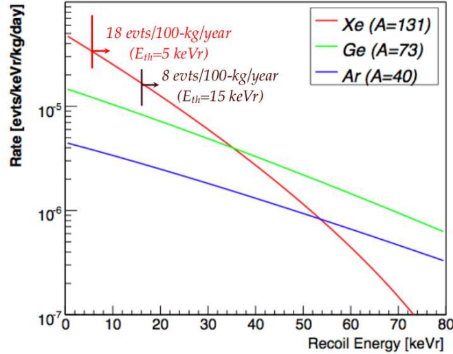
Fig. 1. Event rates for a 100 \text{ GeV}/c^2 WIMP with spin-independent WIMP-nucleon cross-section of 10^{-44} \text{ cm}^2 for different target materials.
