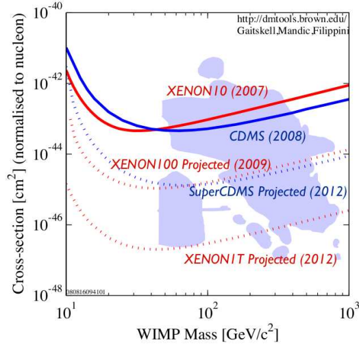
Fig. 5. WIMP-nucleon cross-section upper limit (90% C.L.) from direct dark matter search experiments. The projected upper limits are shown as dashed lines.
