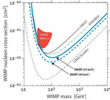
Fig. 10. 90% C.L. spin-independent limits obtained for a total fiducial exposure of 96.5 kgd and a threshold of 55 keV (solid blue curve), and also with a threshold of 40 keV (dashed blue curve).
