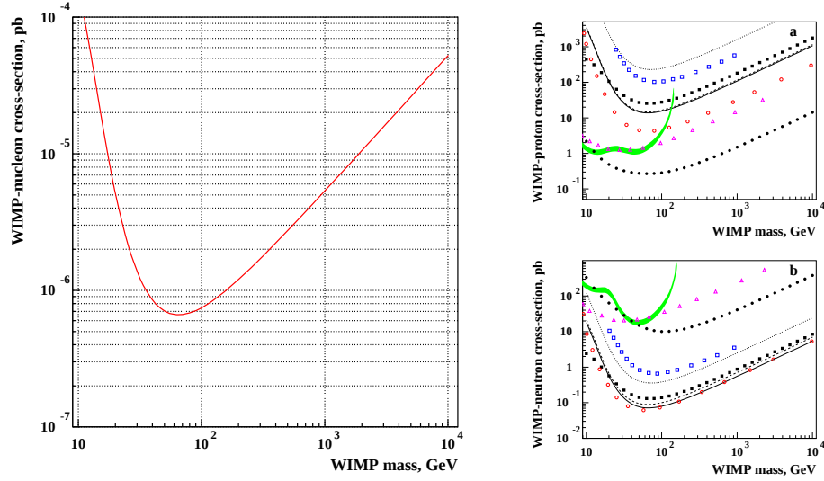
Fig. 8. ZEPLIN II 90% C.L. upper limit on the cross-section of WIMP-nucleon spin-independent interactions (left). 90% C.L. upper limits on the WIMP-proton (right, up) and WIMP-neutron (right, down) spin-dependent cross-sections (solid curves). Also are shown the results from: NAIAD (filled circles), ZEPLIN I (filled squares), CDMS (circles), EDELWEISS (squares) and PICASSO (triangles).
