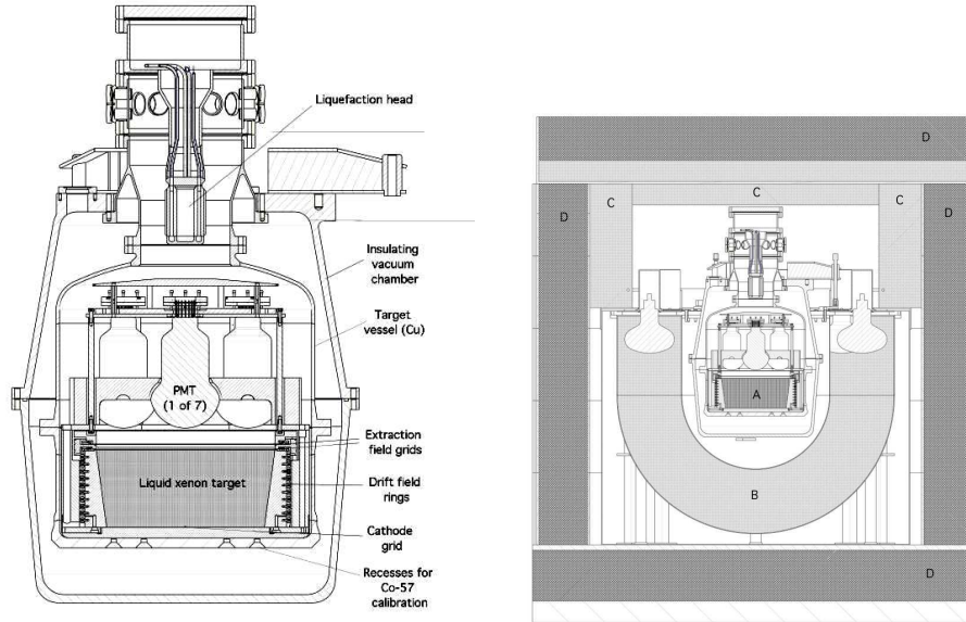
Fig. 7. Schematic of the ZEPLIN II detector (left). The ZEPLIN II detector (A) within its \gamma (25 cm Pb (D)) and neutron shielding (30 cm Gd-loaded polypropylene (C) and 1 tonne liquid scintillator active veto (B)) (right).
