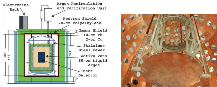
Fig. 11. WArP detector layout.
