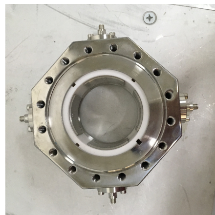
Figure 3: Picture of the XiPAF button BPM.
