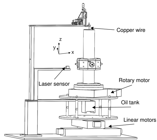
Figure 2: Picture of the test bench.
