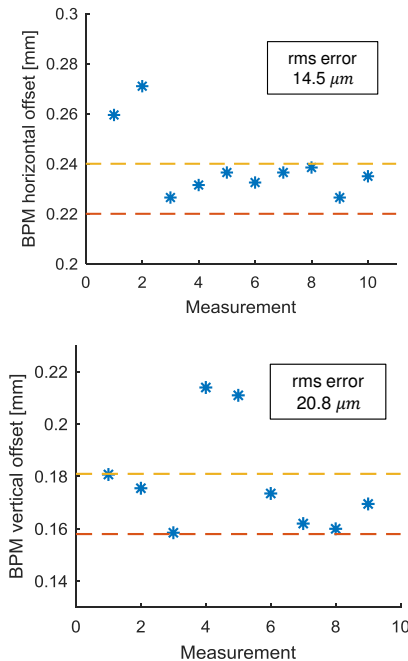
Figure 4: Measured electric offsets of the button BPM.
