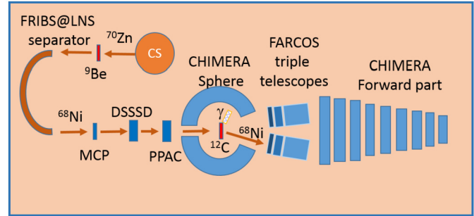
Fig. 1. Sketch, not to scale, of the used experimental set up (color online).
