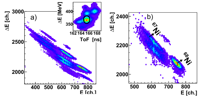
Fig. 2. a) \Delta E - E scatter plot observed with the FARCOS array irradiated by the reactions products produced with the whole cocktail fragmentation beam. Isotopic identification of fragments with Z from 27 to 30 is observed. In the inset the \Delta E -ToF identification scatter plot of the cocktail beam is reported. b) Reaction products detected with the FARCOS array in coincidence with ^{68}\text{Ni} ions, as shown in the black circle in the inset of Fig. 2a (color online).
