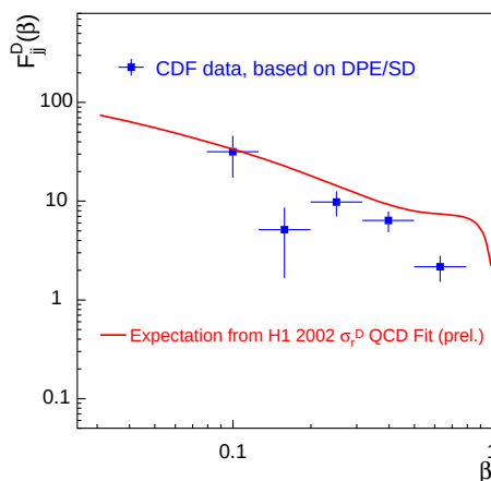
Fig. 4. Comparison of the diffractive structure function of the proton in CDF DPE events [12] with expectations from H1 parton densities from diffractive DIS at HERA [13].
