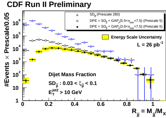
Fig. 6. Number of events as a function of dijet mass fraction in DPE for 5.5 < \eta_{\text{gap}} < 7.5 (open circles), 3.6 < \eta_{\text{gap}} < 7.5 (filled circles), and for SD events (triangles).
