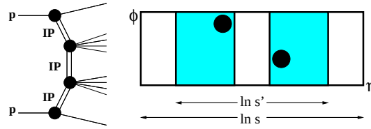
Fig. 5. Schematic diagram and event topology in \eta - \phi space of a DPE interaction pp \rightarrow p + \text{GAP} + X + \text{GAP} + p at c.m. energy \sqrt{s} , where X is a hard DD interaction \mathbb{P}\mathbb{P} \rightarrow \text{JET} + \text{GAP} + \text{JET} at c.m. energy \sqrt{s'} .
