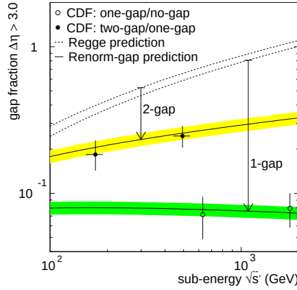
Fig. 2. Ratios of SDD to SD rates (filled circles) and of DD to total cross sections (open circles) as a function of the collision energy of the sub-process, \mathbb{P}p and \bar{p}p , respectively. The uncertainties are mainly systematic and are highly correlated among all four data points. The dashed lines are predictions from Regge theory, and the solid lines from the renormalized gap probability model.
