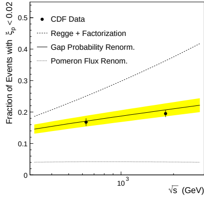
Fig. 3. Fraction of DPE events with \xi_p < 0.02 in events with 0.035 < \xi_{\bar{p}} < 0.095 as a function of \sqrt{s} of the \bar{p}p collision, for CDF data (filled circles), and for predictions from: (solid line) the renormalized gap probability model [10]; (dashed line) standard Regge theory based on factorization; (dotted line) the pomeron flux renormalization model in which the proton and antiproton flux factors are renormalized independently for DPE [11].
