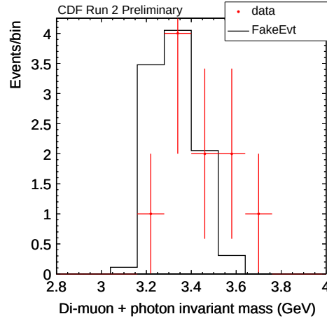
Fig. 7. The invariant mass of the di-muon and \gamma candidate compared to a sample of MC-generated \chi_c^0 events passed through a simulation of the CDF detector.
