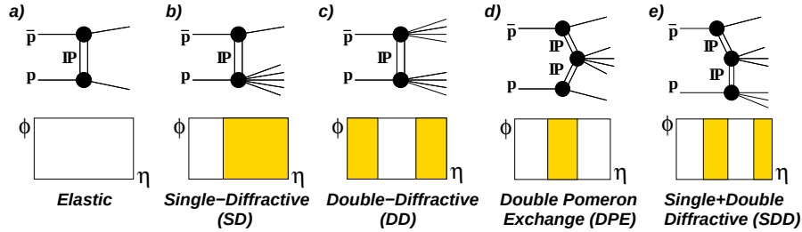
Fig. 1. Event topologies in pseudorapidity ( \eta ) vs azimuthal angle ( \phi ) for (a) elastic, (b) single-diffractive, (c) double-diffractive, (d) double-pomeron exchange, and (e) “single+double diffractive” (SDD) \bar{p}p interactions. Shaded areas represent regions of particle production, while white areas are “rapidity gaps”.
