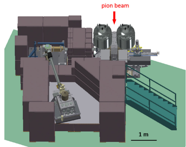
Fig. 4 Set-up of cyclotron trap (top right) and crystal spectrometer in the \pi\text{E5} area at PSI for the \pi\text{H}(2p-1s) transition ( \Theta_B = 54^\circ using the silicon 111 reflection). The massive concrete shielding provides an efficient reduction of beam-induced background which, in addition, yields an efficient temperature stabilisation to \approx \pm 1^\circ\text{C} . The roof of the concrete cave is not shown
