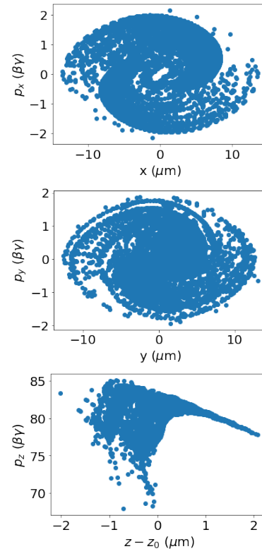
Figure 4: Final witness beam phase space with z_0 representing the witness beam location.
