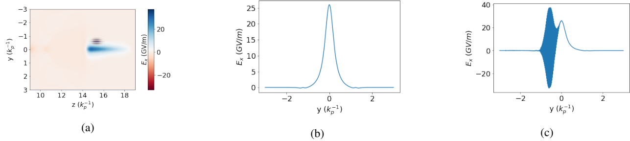
Figure 3: The laser pulse interacts with the beam radial fields on both sides of the mid-plane. The fields on one side of the mid-plane are shown here. The radial field of the beam without the laser is shown in (b) while the superposition of the laser field and beam radial field is shown in (a) and as a lineout in (c) at position x = -7.96 \mu\text{m} .
