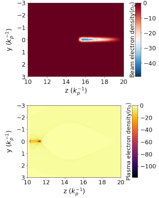
Figure 1: Beam charge (a) and plasma charge densities (b) on the mid-plane y-z.
