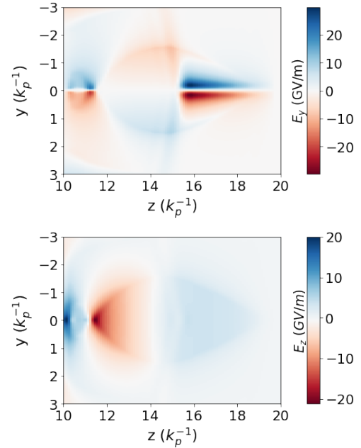
Figure 2: Transverse (a) and longitudinal fields (b) on the mid-plane y-z.
