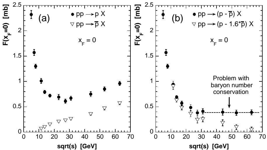
Fig. 5. (a) p_T -integrated invariant p and \bar{p} yields at x_F = 0 as a function of \sqrt{s} ; (b) p - \bar{p} and p - 1.6 \cdot \bar{p} as a function of \sqrt{s} .
