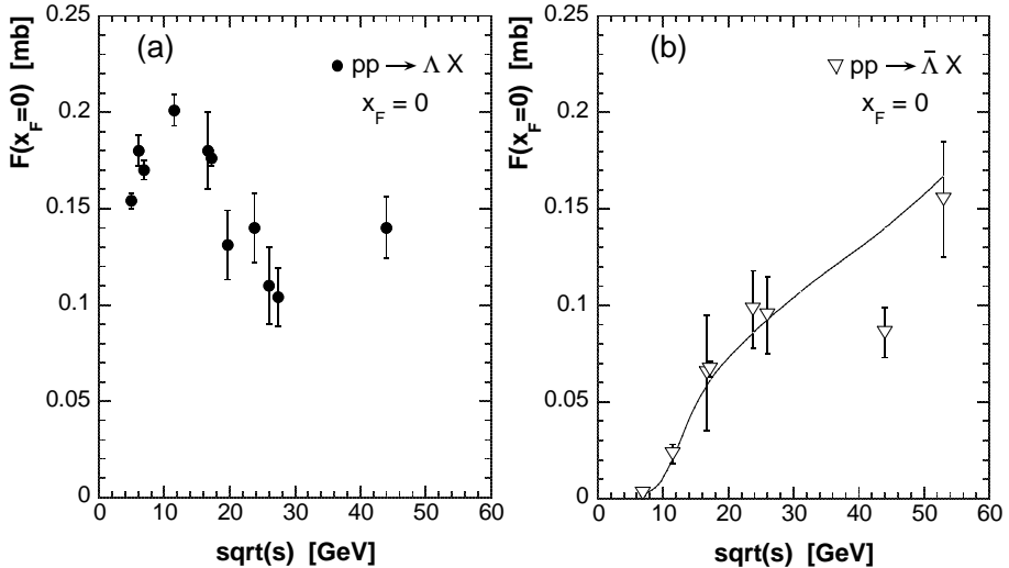
Fig. 6. p_T integrated invariant cross sections at x_F = 0 for (a) Lambda and (b) Anti-Lambda as a function of \sqrt{s} . The line in Fig. 6(b) gives the scaled s -dependence of anti-protons.
