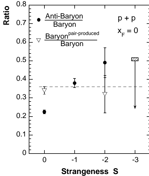
Fig. 7. Anti-baryon/baryon and pair-produced-baryon/baryon ratios at x_F = 0 in p + p interactions as a function of strangeness content.
