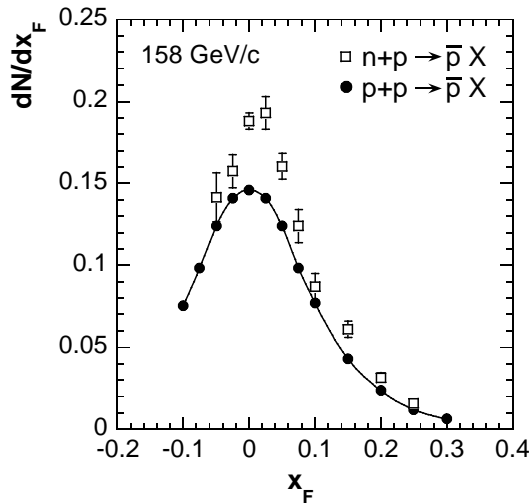
Fig. 4. Anti-proton density distribution as a function of x_F for p + p and n + p interactions.
