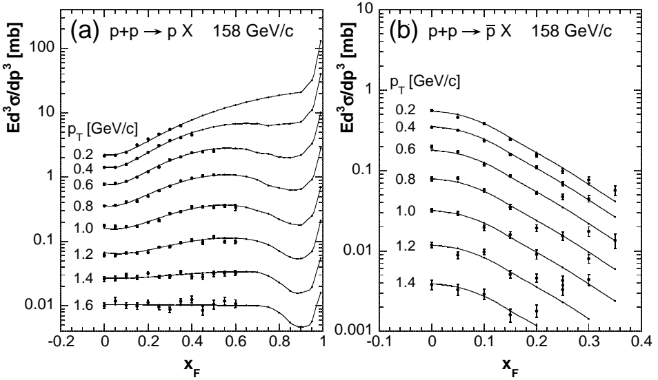
Fig. 1. Invariant inclusive cross section (before hyperon feeddown correction) of (a) protons and (b) anti-protons as a function of x_F in bins of transverse momentum.
