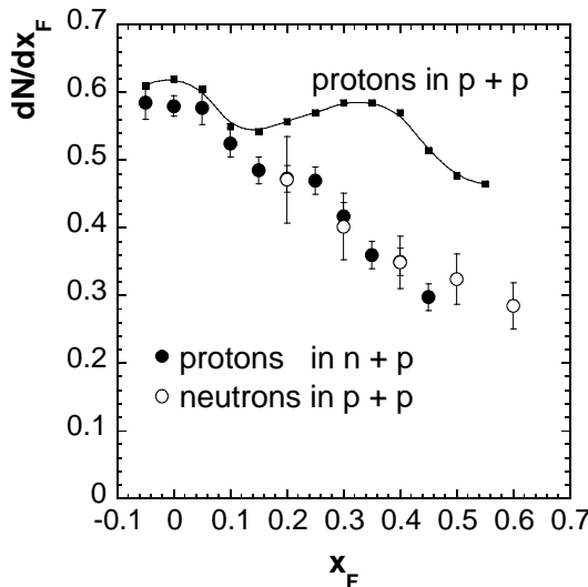
Fig. 2. p_T integrated x_F distributions of protons and neutrons from p + p as well as protons from n + p interactions.
