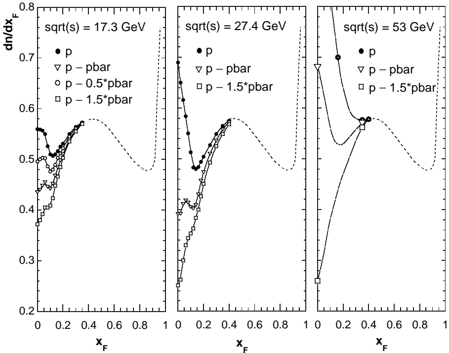
Fig. 3. Net proton distributions as a function of x_F for three c.m.s. energies, subtracting different fractions of anti-proton densities from proton densities.
