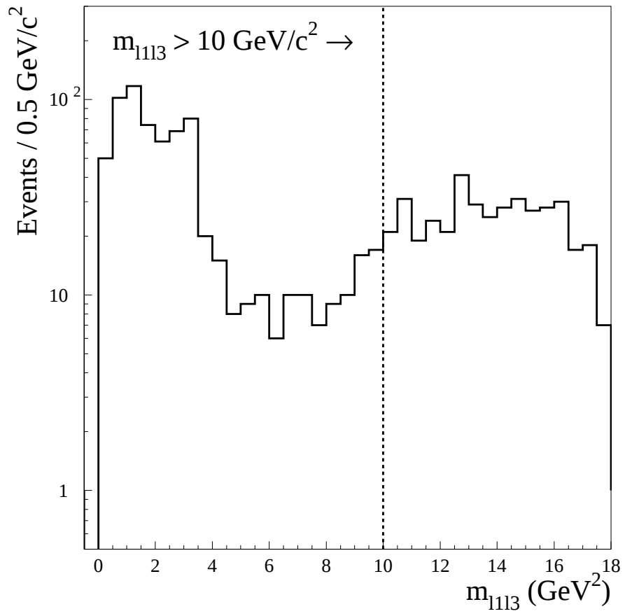
Figure 3.4: Low mass distribution of m_{\ell_1 \ell_3} . The m_{\ell_1 \ell_3} > 10 \text{ GeV}/c^2 cut is marked by the dashed line.
