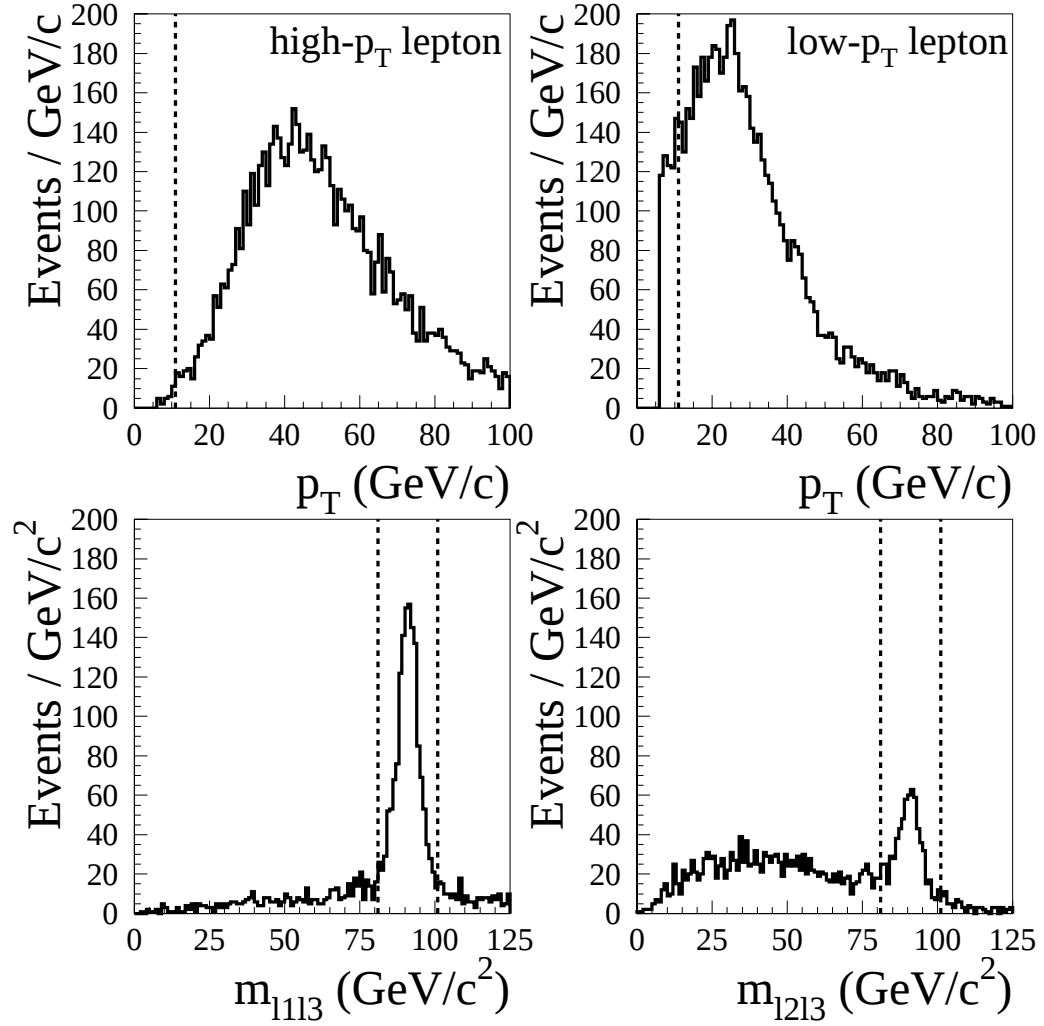
Figure 3.12: Distributions of p_T for both high and low- p_T leptons and m_{\ell_1\ell_3} and m_{\ell_2\ell_3} in W^\pm Z^0 Monte Carlo events prior to applying any LSD analysis cuts. The p_T > 11 GeV/ c cut for each lepton and 81 \text{ GeV}/c^2 < m_{\ell\ell} < 101 \text{ GeV}/c^2 resonance window are marked by dashed lines.
