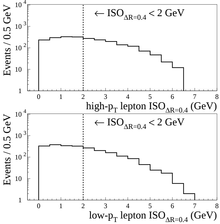
Figure 3.9: Distribution of ISO_{\Delta R=0.4} for the high- p_T lepton (top) and low- p_T lepton (bottom) in the LS dilepton pair. The ISO_{\Delta R=0.4} < 2 \text{ GeV} requirement is marked by the dashed lines. The ISO_{\Delta R=0.7} < 7 \text{ GeV} has already been applied to these distributions.
