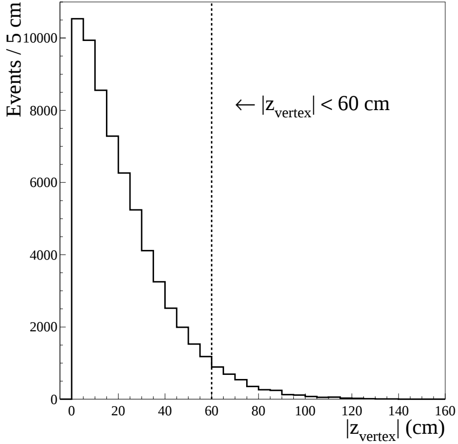
Figure 3.1: Distribution of |z_{\text{vertex}}| . The |z_{\text{vertex}}| < 60 cm cut is marked by the dashed line.
