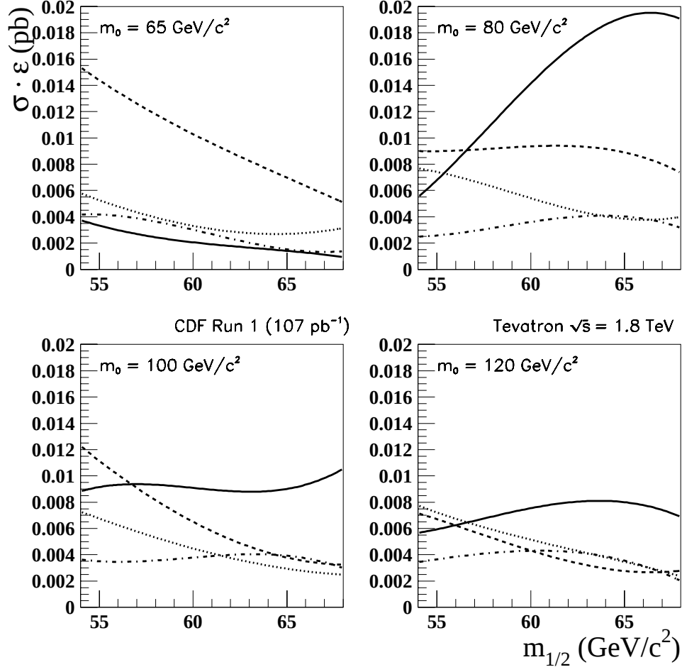
Figure 4.5: Production cross section times the total event acceptance as a function of m_{1/2} for \tilde{\chi}_1^\pm \tilde{\chi}_2^0 (solid line), \tilde{q} \tilde{q} (dashed), and \tilde{\chi}_1^\pm \tilde{g} (dotted) production modes, as well as all other production modes which contribute to the LSD sensitivity (dot-dash).
