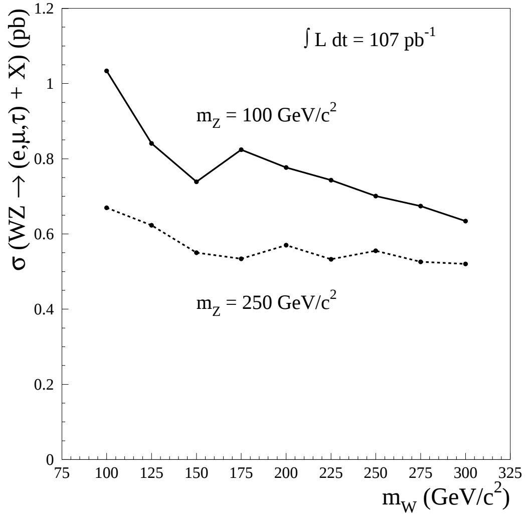
Figure 4.3: WZ -like \bar{\sigma}_{95} as a function of W -like particle mass for two representative points of Z -like particle mass: m_Z = 100 GeV/c 2 (solid line) and 250 GeV/c 2 (dashed line).
