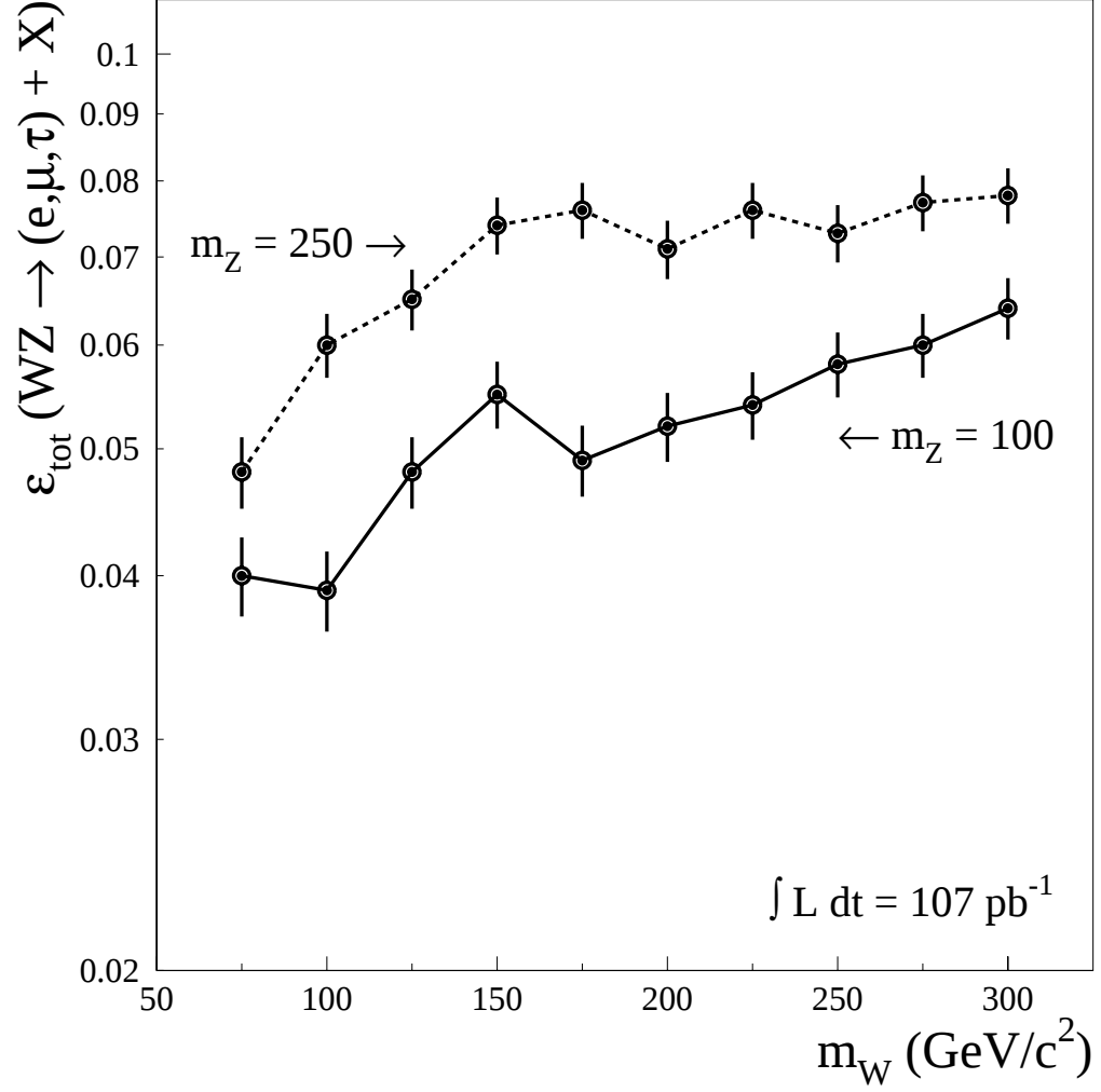
Figure 4.1: WZ -like \epsilon_{tot} as a function of W -like particle mass for two representative points of Z -like particle mass: m_Z = 100 \text{ GeV}/c^2 (solid line) and 250 \text{ GeV}/c^2 (dashed line).
