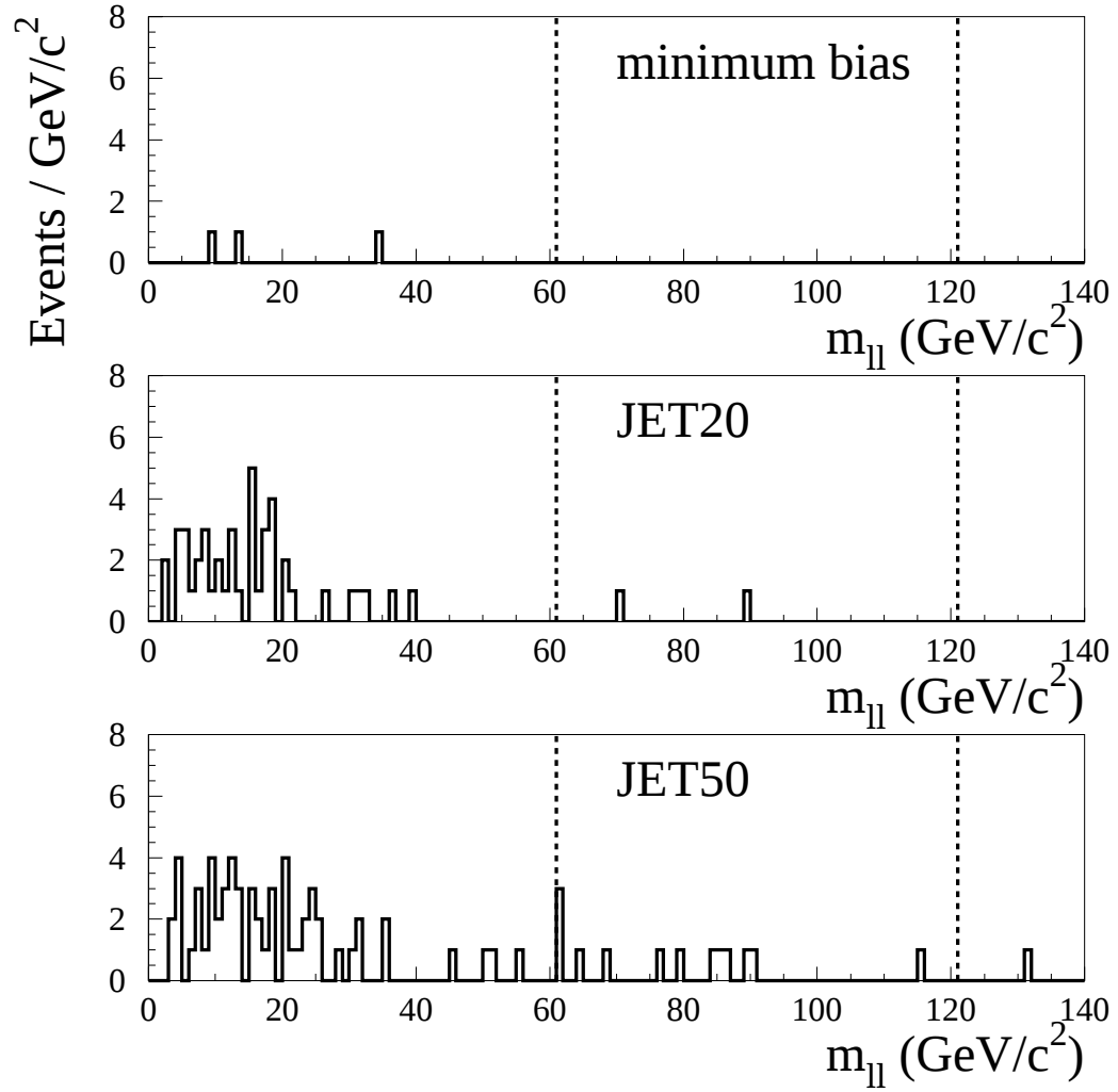
Figure B.6: Distribution of m_{\ell\ell} in minimum bias, JET20, and JET50 data. The invariant mass range 61 \text{ GeV}/c^2 < m_{\ell\ell} < 121 \text{ GeV}/c^2 is marked by the dashed lines. Events with no dilepton pair have been suppressed.
