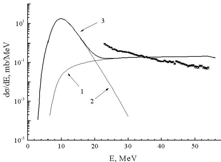
Fig. 3. Comparison of the experimental integrated cross sections for ^{59}\text{Co}(^3\text{He},\alpha\alpha) reactions with calculations within the exciton model. Symbols, experiment: 1 — pre-equilibrium component, 2 — equilibrium emission, 3 — total.
