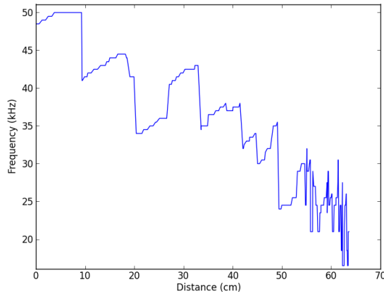
Figure 3: Most Prominent Frequency vs. Microphone Distance from Breakdown Spark Source.
