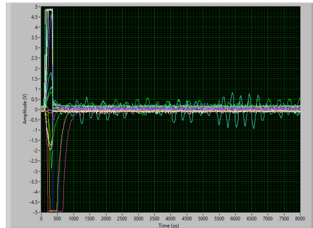
Figure 1: 8 ms of a typical MICE cavity non-spark signal.
