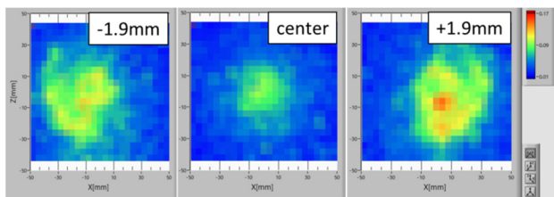
Figure 5: Observed 2D image of Cherenkov ring.
