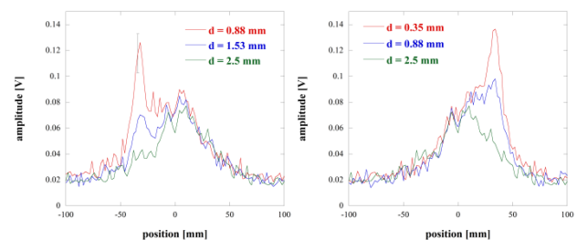
Figure 3: Beam position dependence of the radiation intensity. The beam was steered to -1.05, -1.65 mm (left) and +1.35, +1.85 mm (right). An error bar represents the typical standard deviation of the measured signal.
