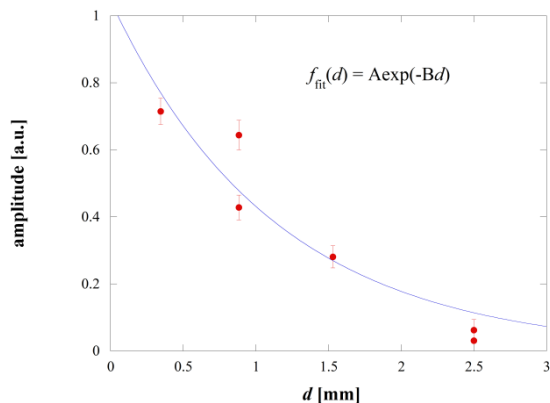
Figure 4: Impact parameter dependence of the coherent ChDR signal.
