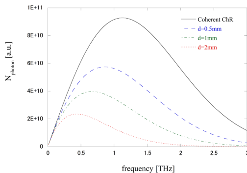
Figure 1: Coherent ChDR spectrum for some impact parameters (0.5, 1, 2 mm), where beam energy of 22 MeV and Gaussian bunch shape of 100 fs (rms) are assumed.
