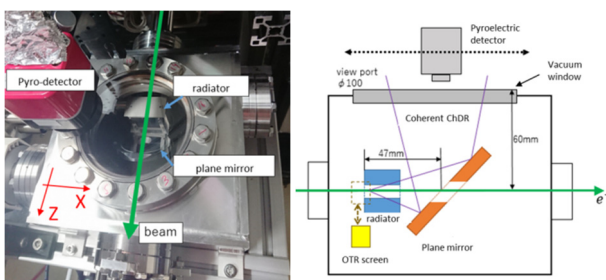
Figure 2: Experimental set-up.
