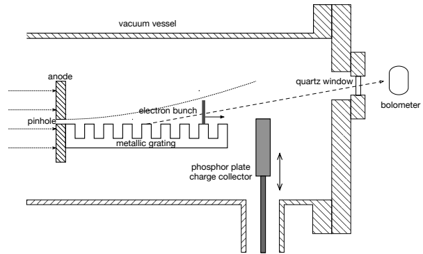
Figure 3: Experimental setup.
