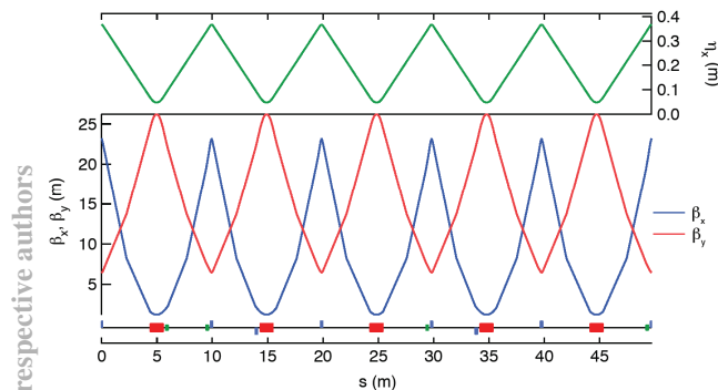
Figure 2: Optical functions for 1/10^{\text{th}} of the Sirius booster lattice.
