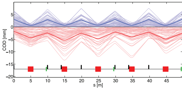
Figure 5: Horizontal (blue) and vertical (red) uncorrected closed orbit for 50 random machines. The bold curves represent one rms value.
