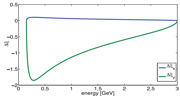
Figure 9: Chromaticities induced by eddy currents due to the ramping process.
