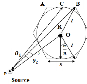
FIG. 1: Schematic diagram for an isotropic point source placed axially at a distance y from the conical detector of an n -sided polygonal cross-section of circumradius l represented here as a hexagon.
