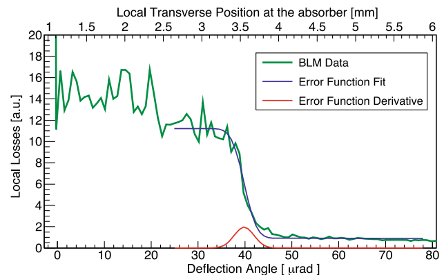
Fig. 6 Beam losses as a function of jaw position and the equivalent deflection at collimator position, recorded at the TCSG.D4L7.B1 during a linear scan with vertical crystal in channeling orientation. The collimator used as absorber has an active jaw of 1 m of CFC (see Table 1) that does not stop all the energy carried by the channeled halo, but is adequate for the measurement of deflection angle
