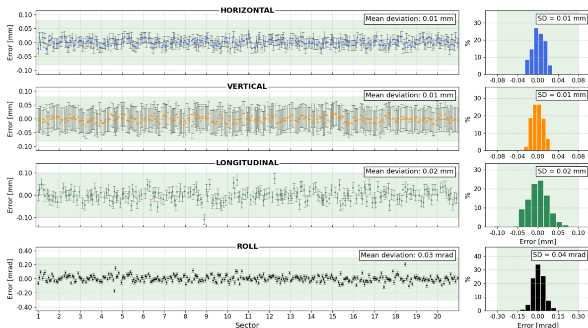
Figure 5: Alignment results for SR magnets. Specific quadrupoles and dipoles were used as positioning references for each of the girders and DOF, and the plotted data are the results for these magnets.
