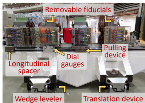
Figure 2: Devices used during alignment operations.
