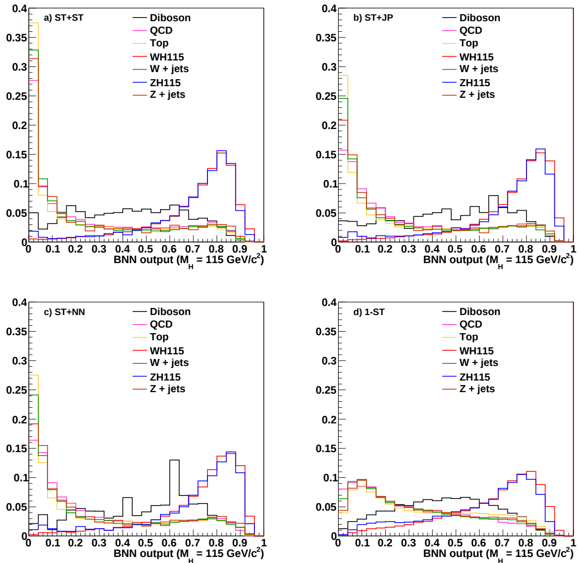
FIG. 1: Comparison of the BNN output for signal ( M_H = 115 \text{ GeV}/c^2 ) and background events with all lepton types included. From (a) - (d) the b -tag categories are ST+ST, ST+JP, ST+NN, and ST, respectively. Signal and background histograms are each normalized to unit area. The WH and ZH signals peak near the 1.0 value. The QCD multijet, top quark, W + \text{jets} and Z + \text{jets} peak near the 0.0 value. The diboson background has a broad peak in the middle region as its kinematics is very close to the signal ones. The diboson spike in figure (c) is a statistical fluctuation.
