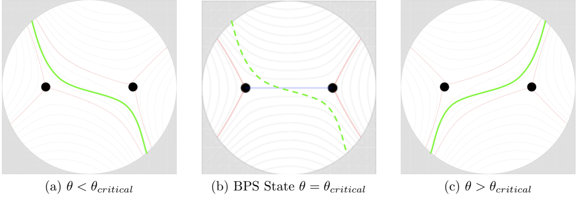
Figure 3.6: Evolution of the special lagrangian flows with the BPS angle \theta . In each picture the black dots indicate the branch points of the cover where flows emerge. Red trajectories are flows that emerge from the branch points and terminate on the boundary at |x| = \infty , while gray trajectories indicate generic flow lines. The green trajectory denotes a representative of a generic flow line which can serve as an edge in the triangulation. In (b) the BPS angle of the flow aligns with the phase of the central charge and a new kind of trajectory, shown in blue, traverses between branch points. Afterwards in (c) the green line has flipped.
