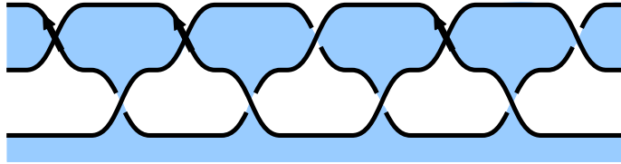
Figure 4.31: The singular braid of the A2 flow in the maximal chamber.
