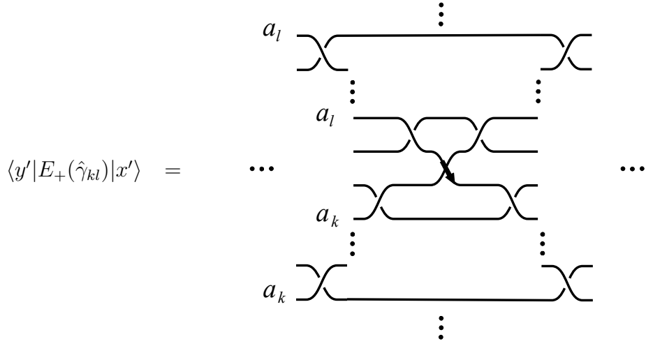
Figure 4.27: Braid realization of a local singularity. The relevant branch points come close to each other until they collide in the singularity and loose their individual identities. After that they depart again until they reach their original positions in the braid.
