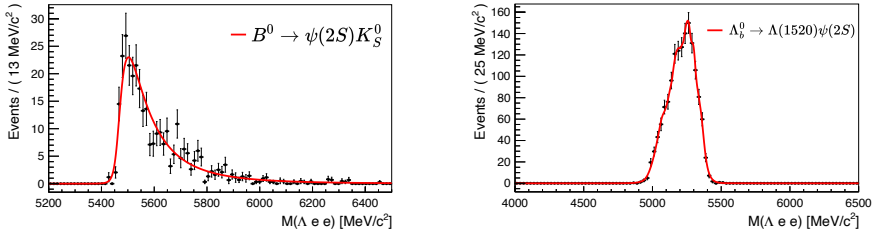
Figure 6.2: Invariant mass likelihood fits on MC simulation for the misidentified B^0 \rightarrow \psi(2S)K_S^0 decays and partially reconstructed \Lambda_b^0 \rightarrow \psi(2S)\Lambda(1520) background (right) for the \Lambda_b^0 \rightarrow \psi(2S)(\rightarrow e^+e^-)\Lambda decay in the combined 2017 and 2018 samples using downstream reconstructed \Lambda hadrons.
