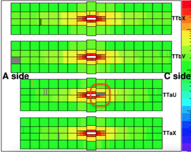
Figure 5.4: Relative occupancy distribution of the TT layers in 2017 data [72]. The red circle at the u layer indicates the broken sensor in the high occupancy region.
