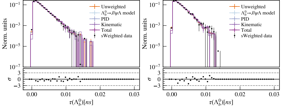
Figure 4.9: Distribution of the lifetime of \Lambda_b^0 \rightarrow J/\psi(\rightarrow \mu^+\mu^-)\Lambda decays for signal data (black points) and simulation before (orange lines) and after (dark purple lines) the re-weighting. The left plot describes samples with the \Lambda baryon reconstructed with downstream tracks, while the right one describes the samples with long tracks, both using 2018 data.
