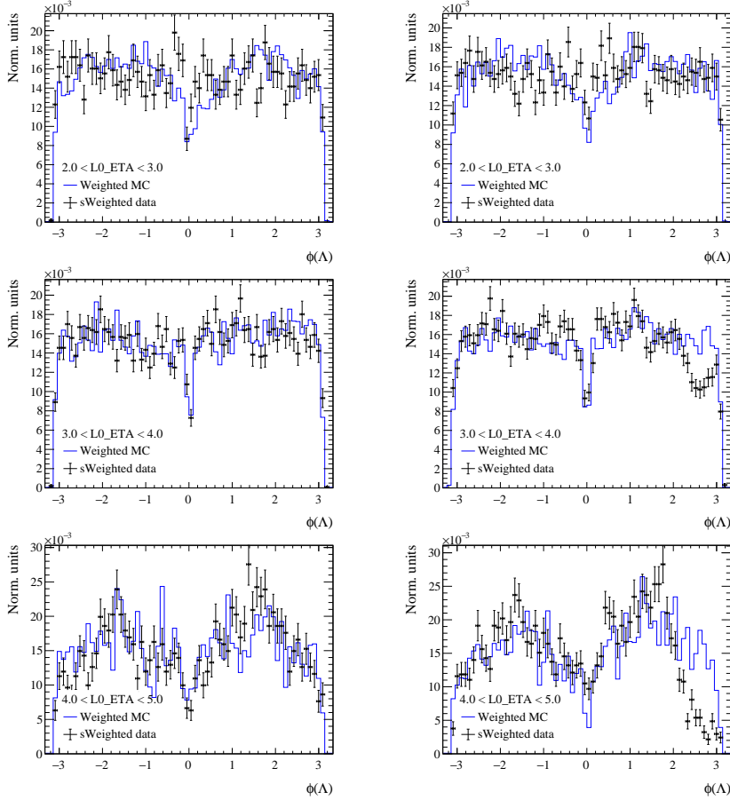
Figure 5.2: sWeighted data and MC simulation \phi(\Lambda) comparison for \Lambda_b^0 \rightarrow J/\psi(\rightarrow \mu^+\mu^-)\Lambda decays for the 2016 (left) and 2018 (right) samples in different bins of \eta(\Lambda) with the \Lambda reconstructed using downstream tracks. A discrepancy is visible for 2018 in the high \eta and \phi region.
