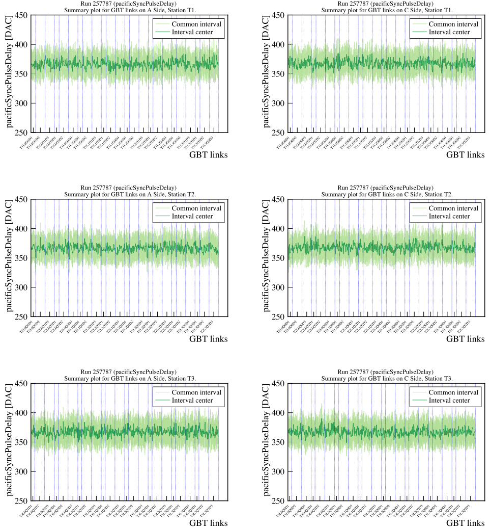
Figure 7.19: 2D overview histograms for the full SciFi detector showing the error-free region in DAC values per link for the PACIFIC SyncPulse scan split by side and T station, where the dotted blue lines indicate the TELL40 boundaries. Compared to the PACIFIC main clock scan, here an error-free region for the whole detector is visible.
