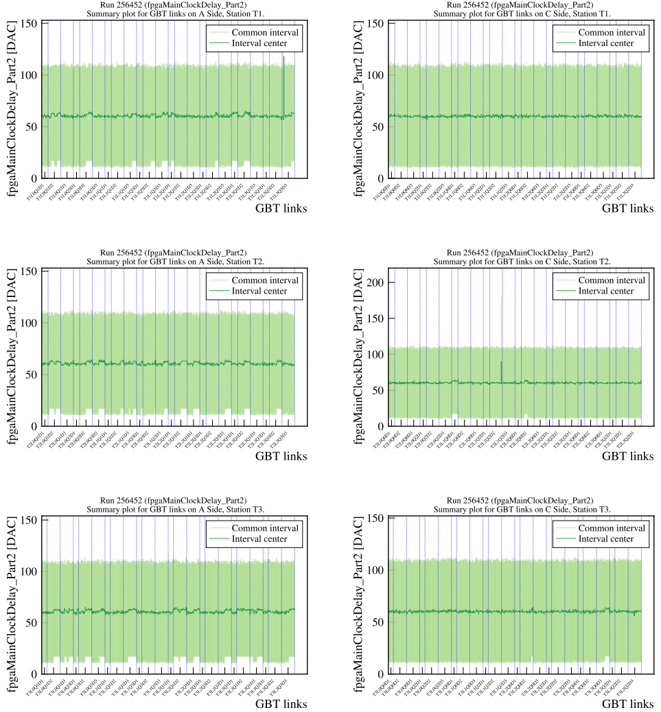
Figure 7.14: 2D overview histograms for the full SciFi detector showing the error-free region in DAC values per link for the FPGA Main clock scan. Each plot shows the result for a given station (top to bottom) and detector side (left and right) where the dotted blue lines indicate the TELL40 boundaries. A similar interval center is visible throughout the whole detector.
