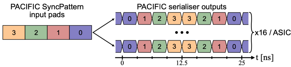
Figure 7.10: Schematic drawing of the PACIFIC SyncPattern, showing that the 4 bits are combined with the same, inverted 4 bits, such that 12.5 ns phase shifts can be detected.
