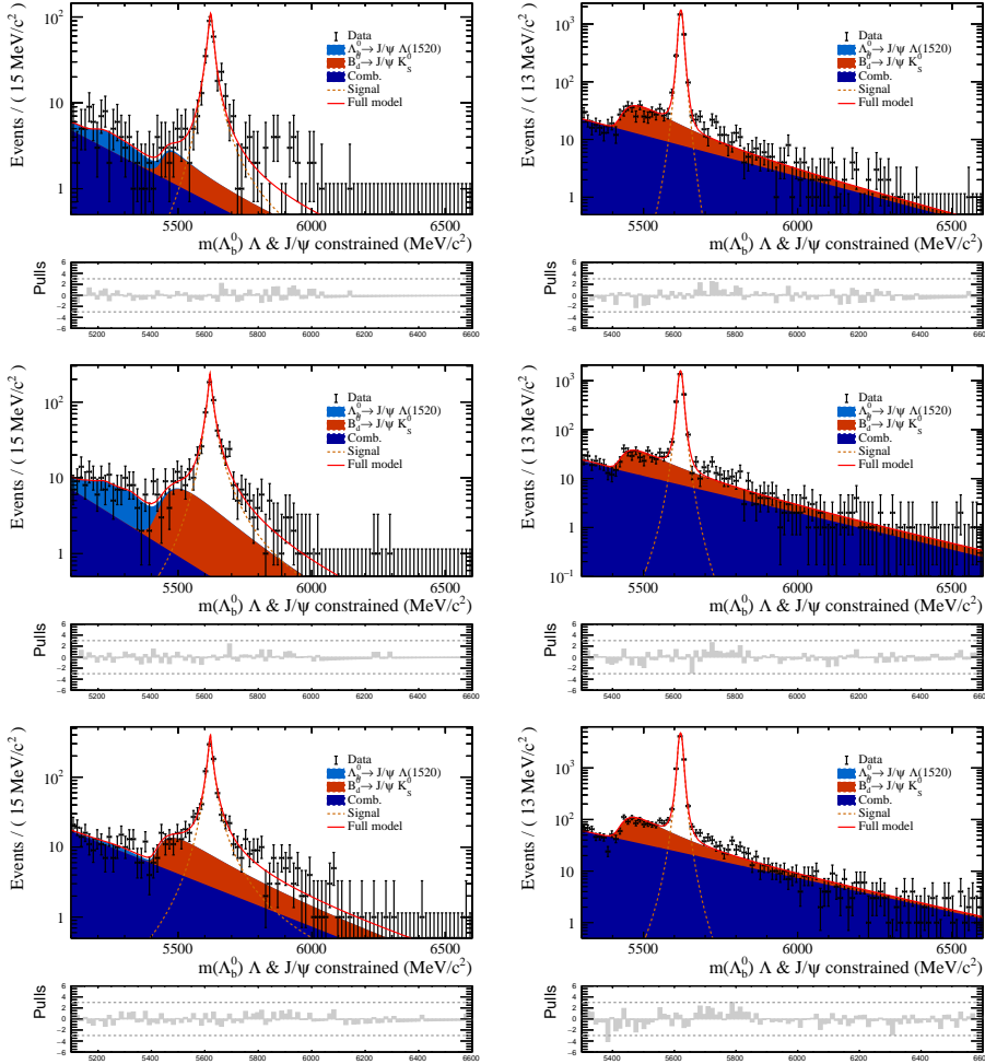
Figure E.7: Maximum likelihood invariant mass fits for the \Lambda_b^0 \rightarrow J/\psi(\rightarrow e^+e^-)\Lambda (left) and \Lambda_b^0 \rightarrow J/\psi(\rightarrow \mu^+\mu^-)\Lambda (right) candidates using long reconstructed \Lambda candidates using the Run 1 (top), 2015+2016 (middle), and 2017+2018 (bottom) data samples. The red line shows the total fit model, the orange dotted line the fitted signal, the dark blue filled area the combinatorial background, the red filled area the mis-identified background, and the light blue filled area the partially reconstructed background.
