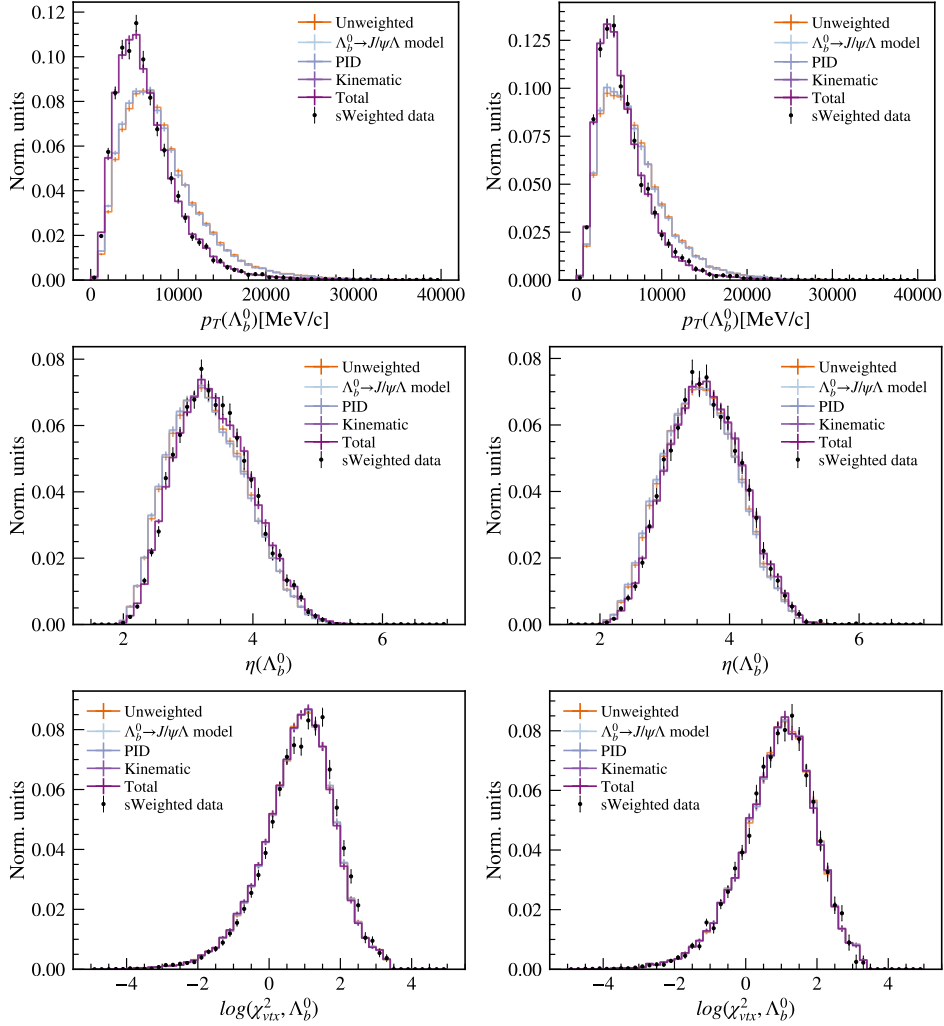
Figure 4.17: p_T(\Lambda_b^0) (top), \eta(\Lambda_b^0) (middle) and \chi_{VTX}^2(\Lambda_b^0) (bottom) distributions for \Lambda_b^0 \rightarrow J/\psi(\rightarrow \mu^+ \mu^-) \Lambda decays for sWeighted data (black points) and simulation before (orange lines) and after (dark purple line) the re-weighting. The left graphs show the candidates with the \Lambda reconstructed using downstream tracks in 2018 data sample, while the right shows the long track sample for 2018 data. The effect of the tracking and trigger weights are included in the "Total", and have a small effect. Therefore, the "Total" and "Kinematic" lines almost completely overlap.
