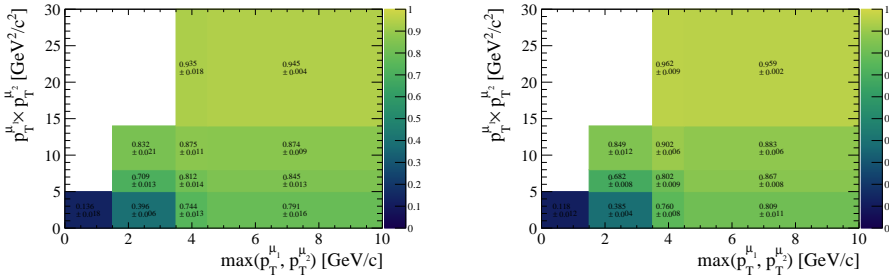
Figure 4.15: TISTOS efficiency maps for the 2015 trigger selection for \Lambda_b^0 \rightarrow J/\psi(\rightarrow \mu^+\mu^-)\Lambda data (left) and simulation (right).
