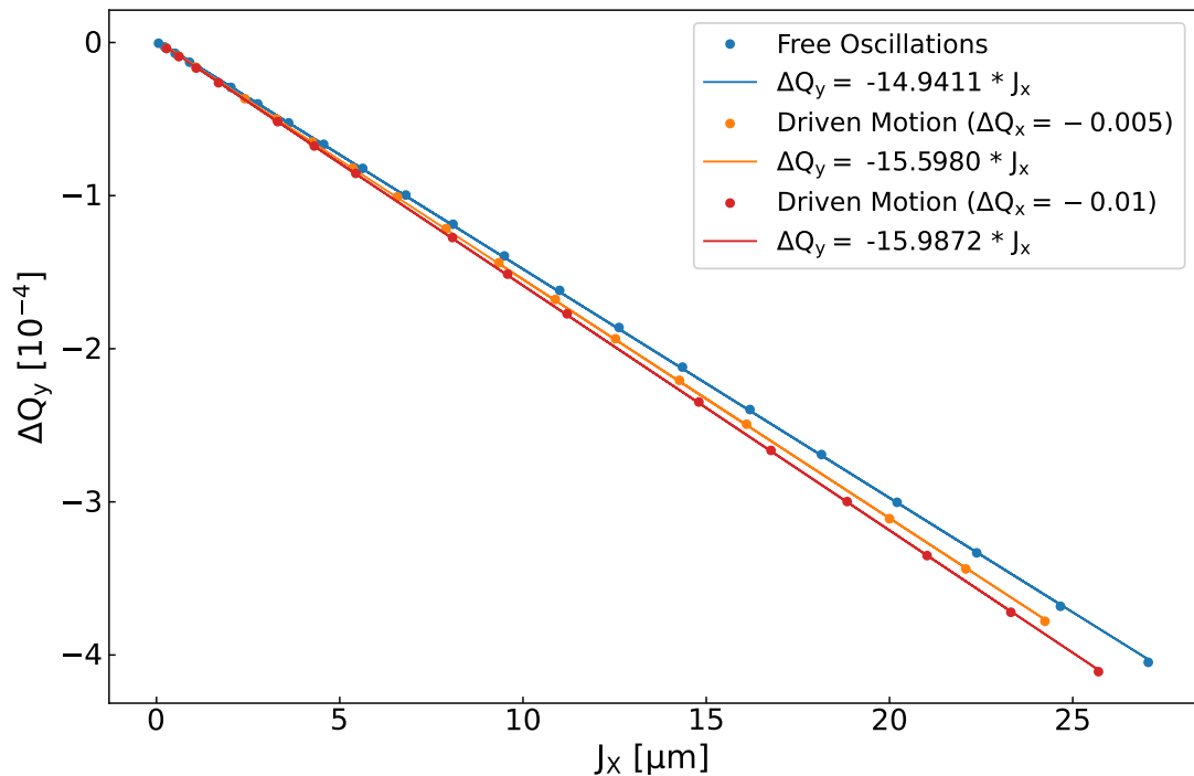
FIGURE 6.9: Natural vertical tune Q_y shift with horizontal free or forced action ( J_x or A_x ), in the case of free oscillations (blue) and driven motion with \Delta Q_x = -0.01 (red) and \Delta Q_x = -0.005 (orange).
