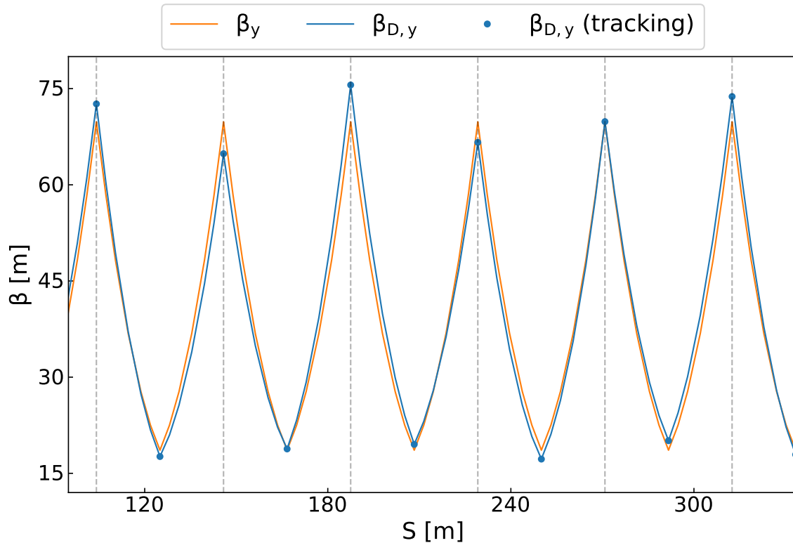
FIGURE 3.16: Resulting vertical \beta -functions in a FODO lattice in the case of free (orange) and driven (blue) oscillations.
