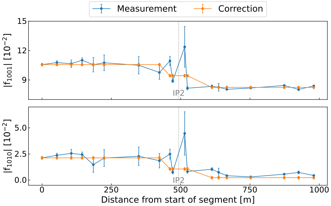
FIGURE 3.22: Local coupling RDTs correction in IR2 (vertical line indicates IP2) from the LHC 2021 beam test. The blue line shows the measured RDTs, while the orange line shows the attempt at canceling the contribution at the edges of the segment with the two available correctors in the IR.
