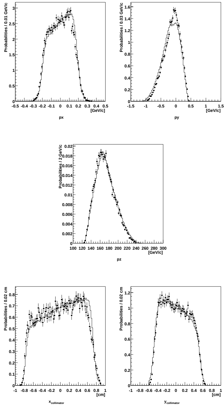
Figure 4.38: Comparisons of momentum components ( p_x , p_y , p_z ) and positions ( x_{\text{collimator}} , y_{\text{collimator}} ) of K^+ at the exit of the collimator for data (histograms) and MC (dots).
