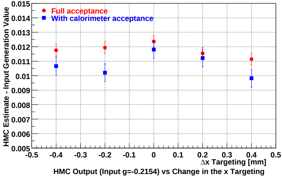
Figure 4.43: Difference between HMC estimates and input g value as a function of X position at the target.
