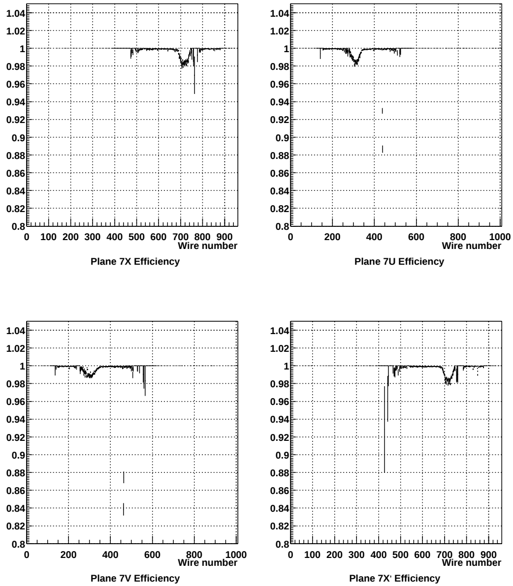
Figure 3.13: Wire efficiency of C7 for positive run 2179.
