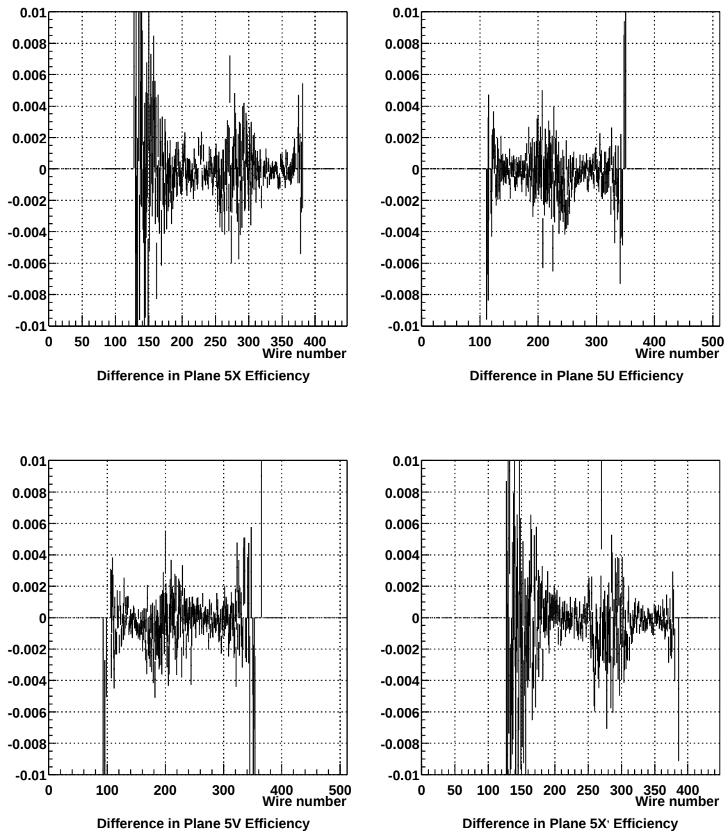
Figure 3.19: Difference in wire efficiency for C5 between positive run 2179 and negative run 2369.
