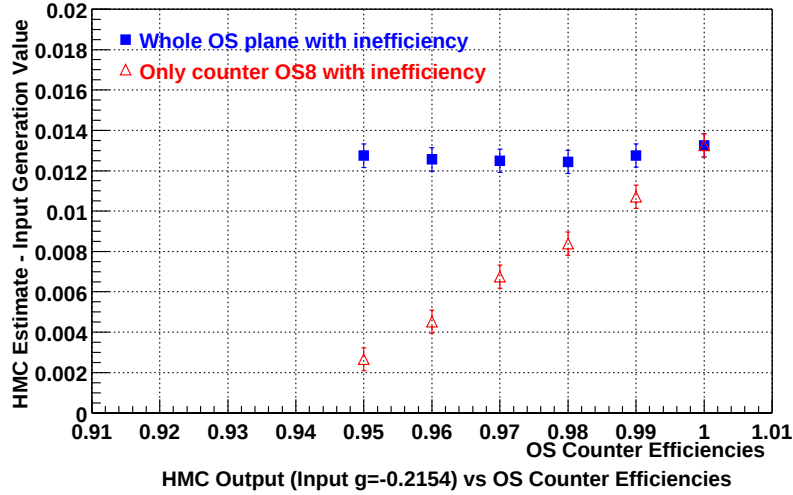
Figure 4.36: Difference between HMC estimates and input g value as a function of OS counter efficiency with reconstructed input .
