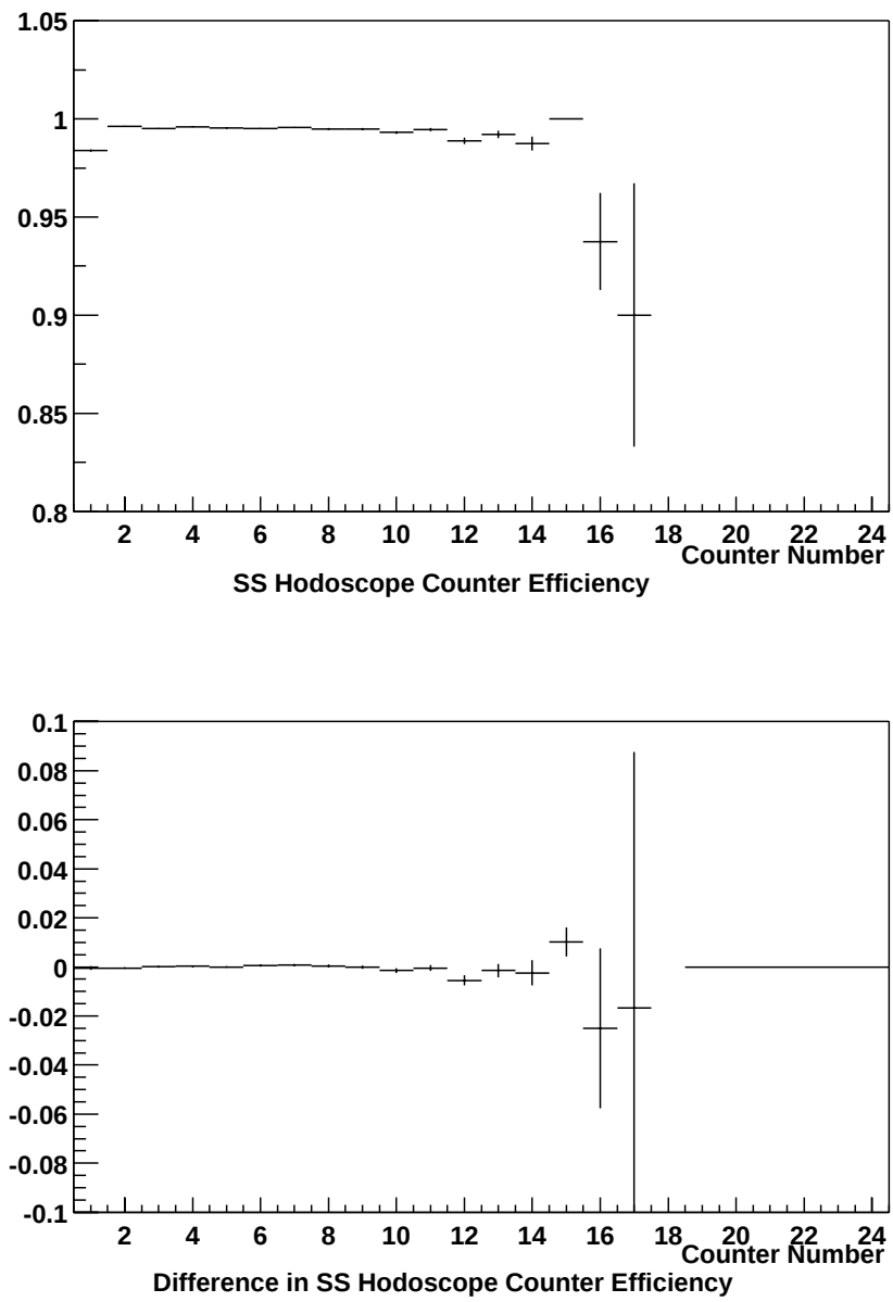
Figure 3.24: Efficiency of SS counters for positive run 2179 is shown in the top plot. Difference in the efficiencies of the SS counters between positive run 2179 and negative run 2369 is shown in the bottom plot.
