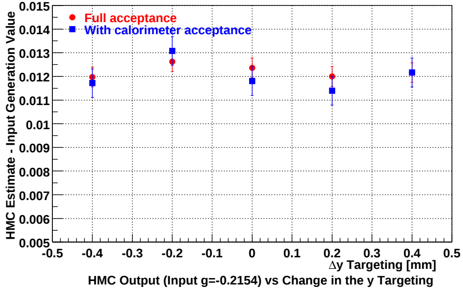
Figure 4.44: Difference between HMC estimates and input g value as a function of Y position at the target.
