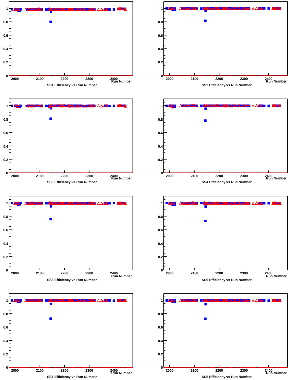
Figure 4.11: Efficiency of SS1 to SS8 versus run number for positive runs (square) and negative runs (open triangle).
