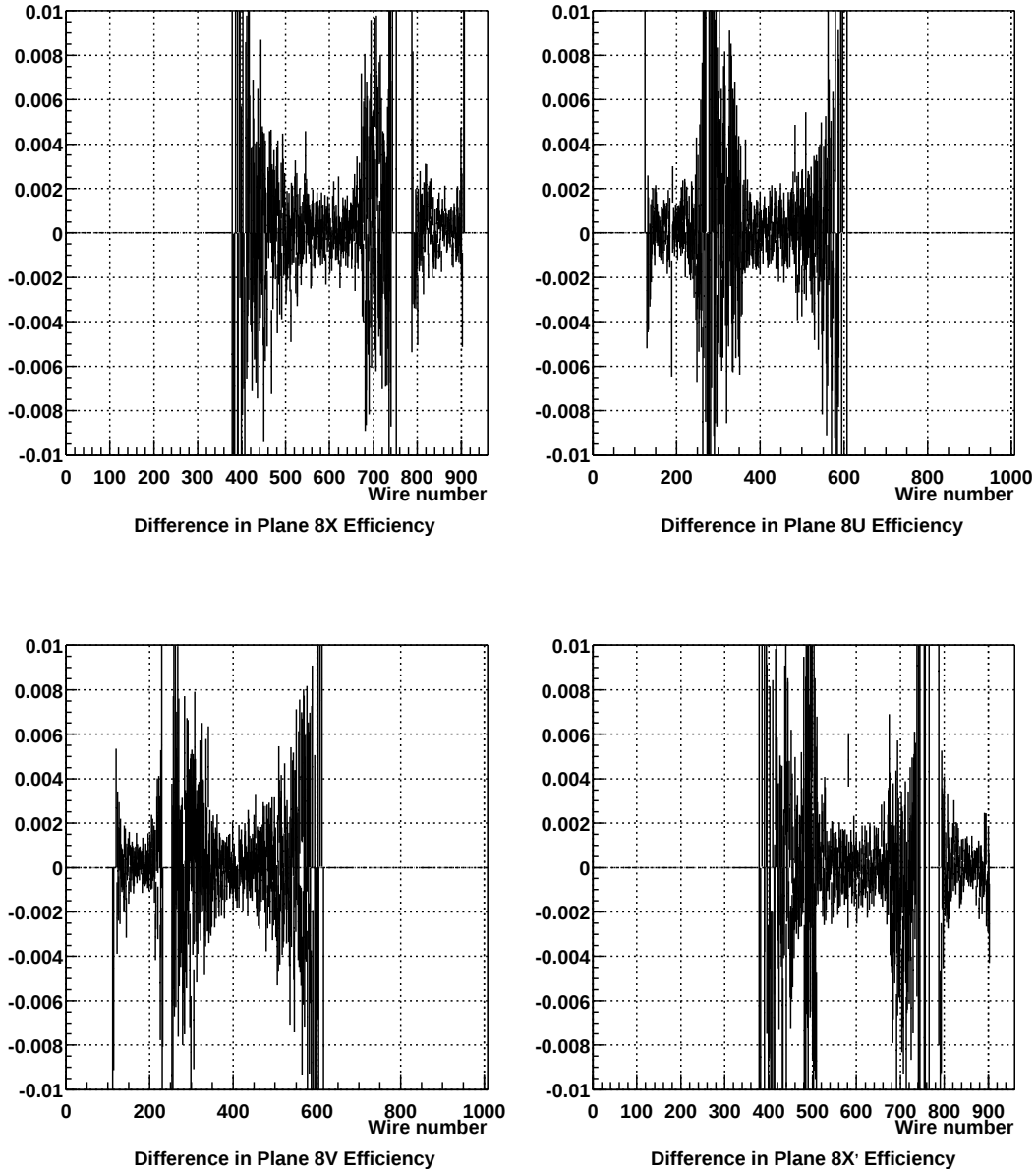
Figure 3.22: Difference in wire efficiency for C8 between positive run 2179 and negative run 2369.
