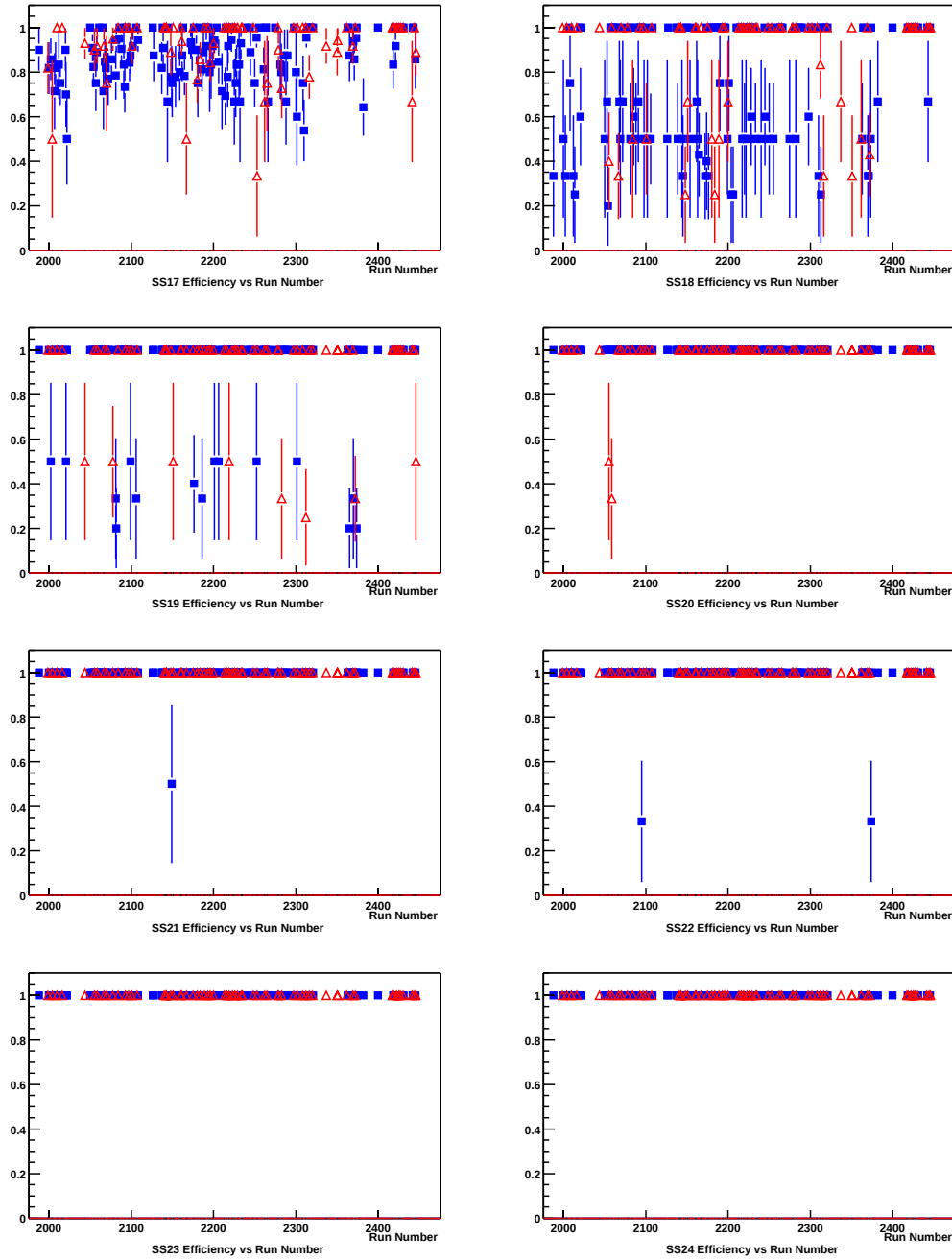
Figure 4.13: Efficiency of SS17 to SS24 versus run number for positive runs (square) and negative runs (open triangle).
