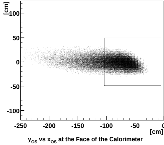
Figure 2.7: Distribution of Y-position versus X-position of opposite-sign pion from simulated \tau decay of charged Kaon at the location of the calorimeter. The box indicates the cross-section of the upstream face of the calorimeter.
