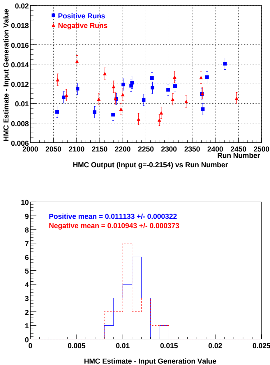
Figure 4.41: Difference between HMC estimates and input g value. Input MC events were generated with the measured response of the trigger hodoscopes. The top plot shows the difference between the HMC estimates and the input g value as a function of run. The bottom plot is a distribution of the difference for the positive (line) and negative (dash) runs with the numbers indicating the mean of the distribution.
